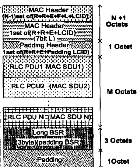
(c) case 3, implicit padding BSR
