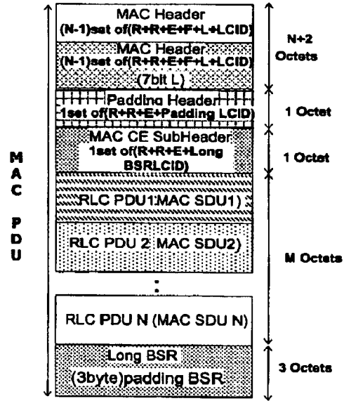
(c) case3, explicit padding BSR
