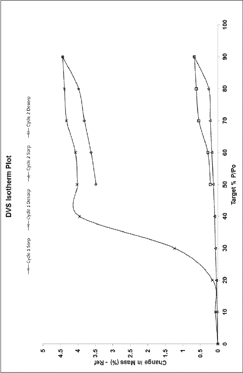
FIG. 7 - Dynamic vapor sorption plot of Form H A at 50°C
