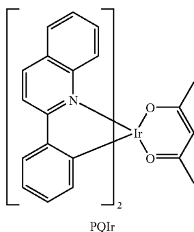
The second transition metal organic complex
