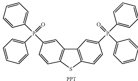
The second host material
