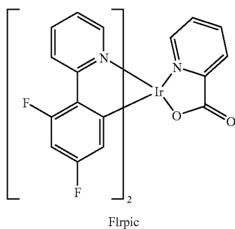
The first transition metal organic complex
