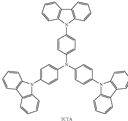
The carrier transport material
