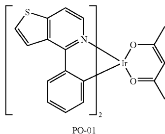
The second transition metal organic complex
