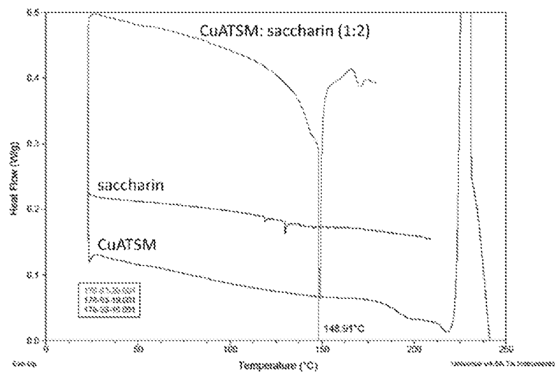
Figure 3. DSC of CuATSM: saccharin (1:2) compared to the DSC of CuATSM and of saccharin.
