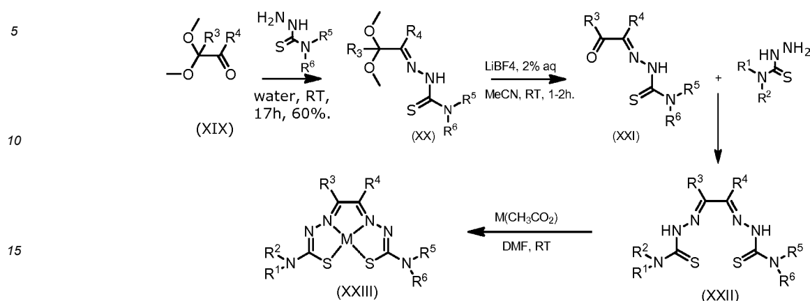
Scheme 3: Alternative Formation of unsymmetrical bis(thiosemicarbazones).
