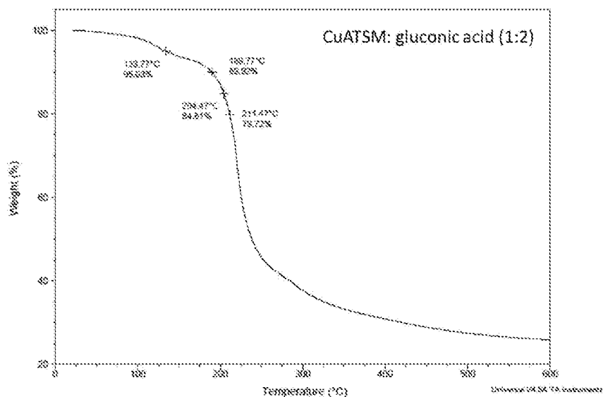
Figure 7. Thermogravimetric analysis (TGA) of CuATSM: gluconic acid (1:2) product of 90-minute ball-milling of ASTMH 2 with Cu(II) gluconate.
