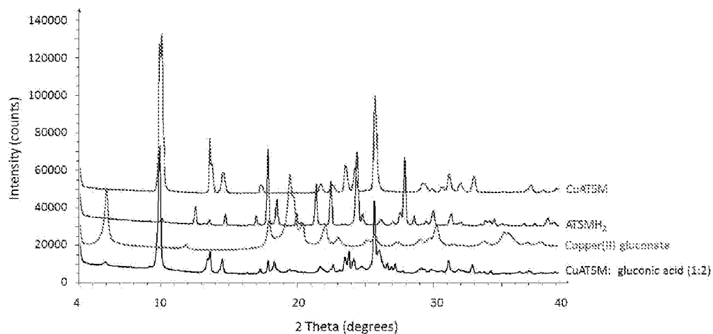
Figure 5. X-ray powder diffraction (XRPD) spectrum of CuATSM: gluconic acid (1:2) prepared by ball-milling, with comparison to XRPD spectra of copper(II) gluconate and ATSMH 2 starting materials, and to XRPD spectrum of CuATSM. Spectra are offset vertically from one another by 10000 counts.
