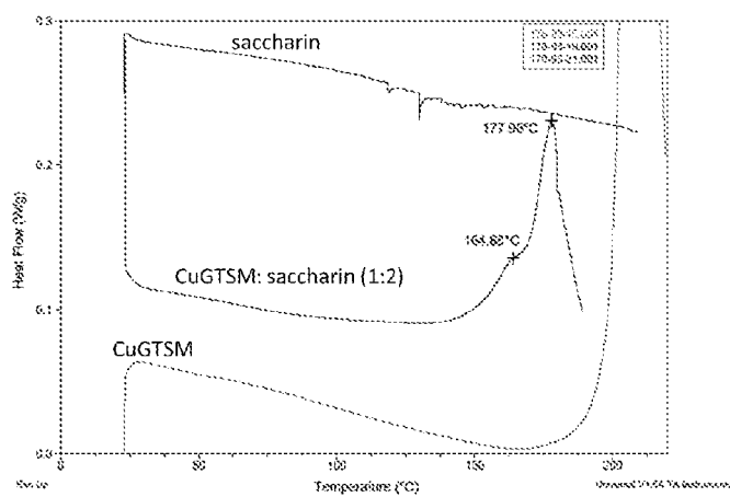
Figure 4. DSC of CuGTSM: saccharin (1:2) compared to DSC of saccharin and of CuGTSM.
