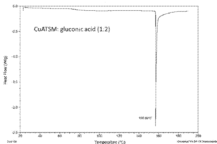
Figure 6. DSC of CuATSM: gluconic acid (1:2) product of 90-minute ball-milling of ATSMH 2 with Cu(II) gluconate.
