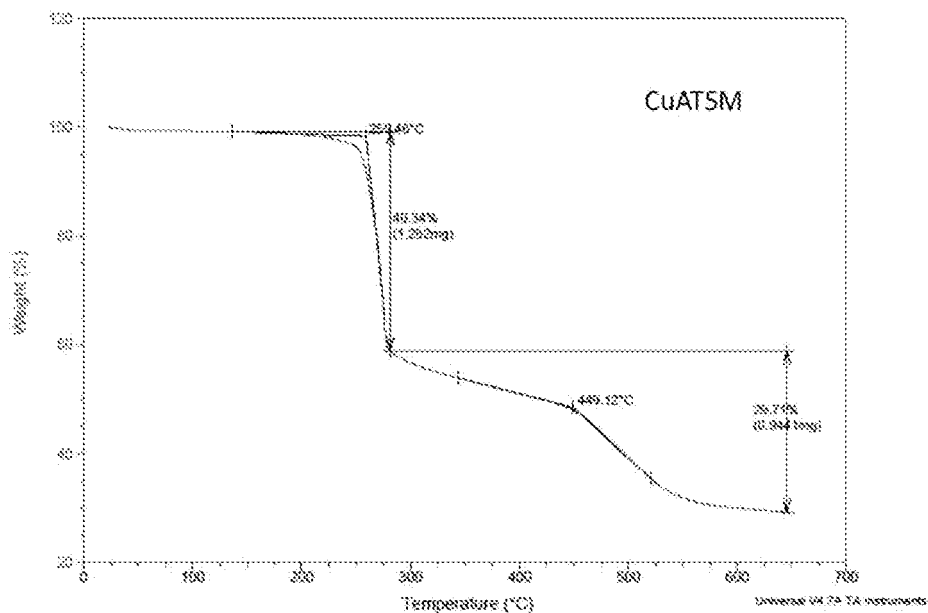
Figure 1. Thermogravimetric analysis of sample of CuATSM (Structure I, R^1 and R^6 = H ; R^2 , R^3 , R^4 and R^5 = Me ) used for preparation of malic acid NCD of Figure 2.
