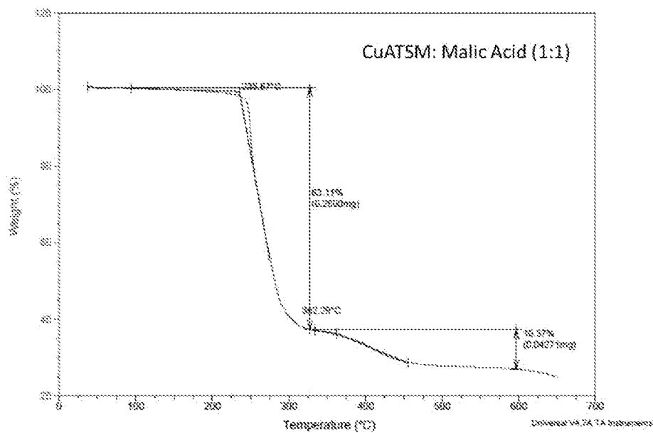
Figure 2. Thermogravimetric analysis of a non-covalent derivative of CuATSM with Malic Acid (1:1).
