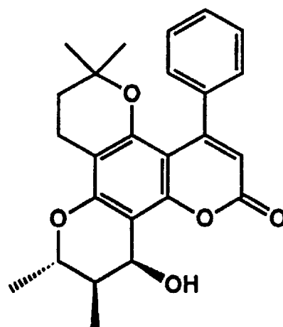
Dihydrosoulattrolide
