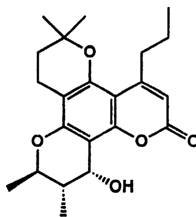
Dihydrocalanolide B
