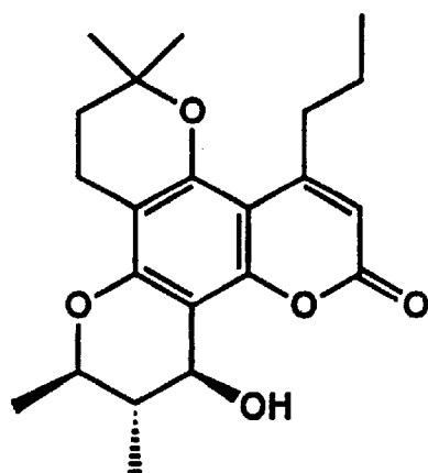
Dihydrocalanolide A
