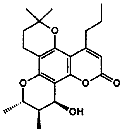
Dihydrocostatolide
