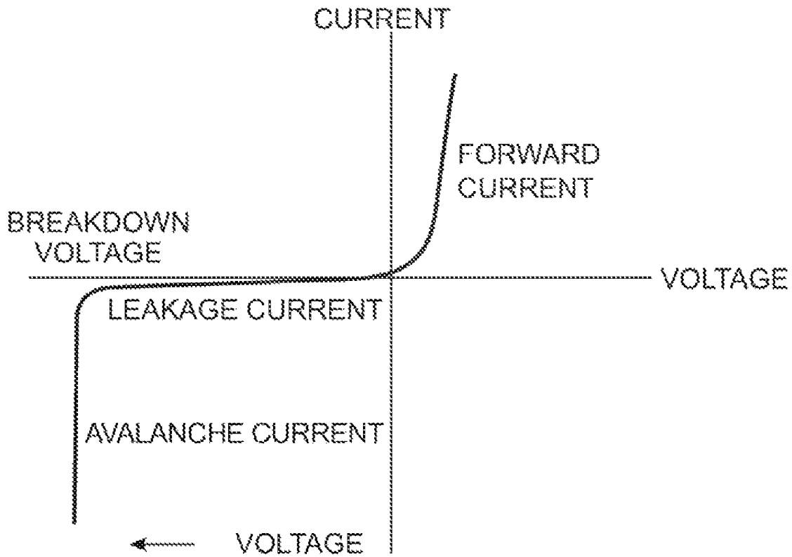
Current-voltage characteristics of a typical P-N junction
