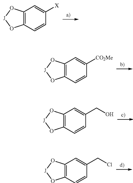
Scheme I-Preparation of cycloalkyl acids.
