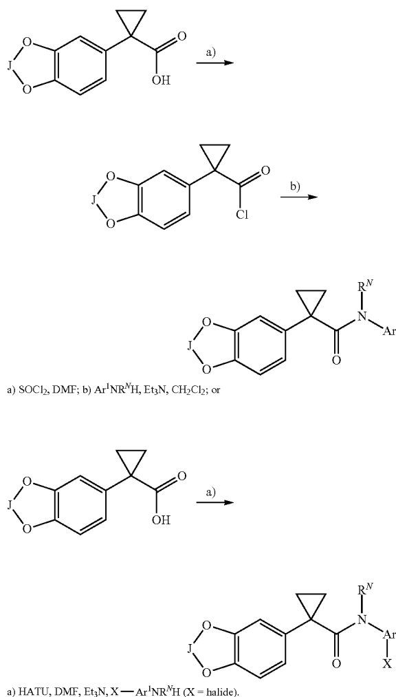
Scheme II-Amid coupling
