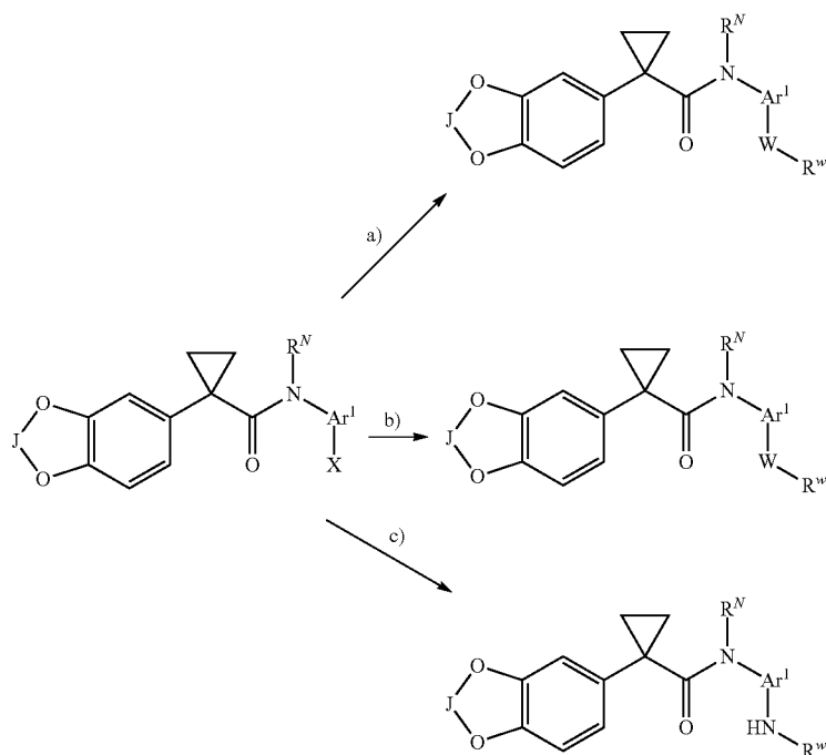
Scheme III-Derivatization of heteroarylhalides
