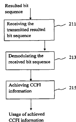
Receiving Flowchart 1
