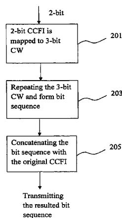
Transmission Flowchart 1
