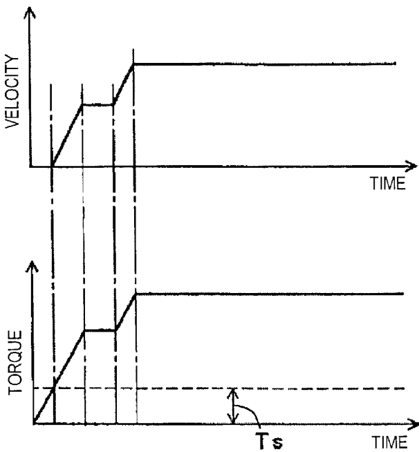
FIG. 8 PRIOR ART
