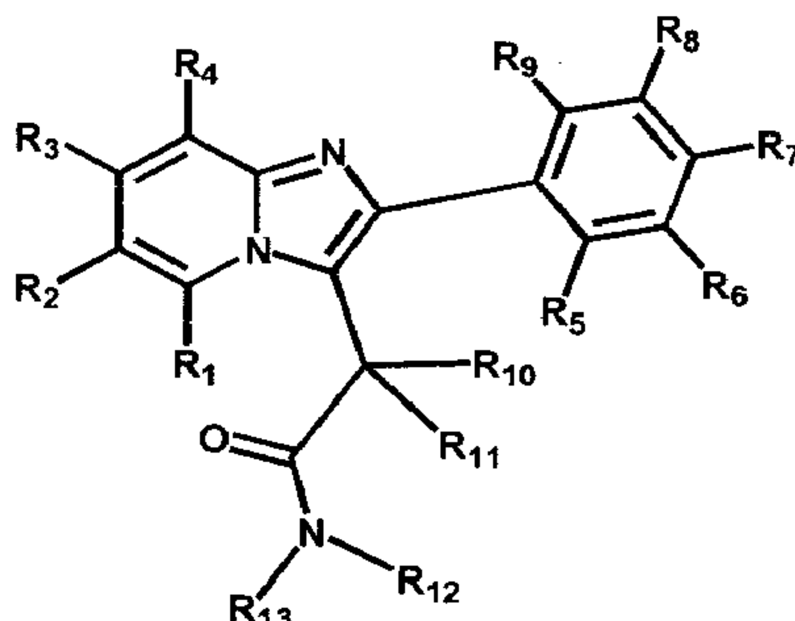
Formula 1
