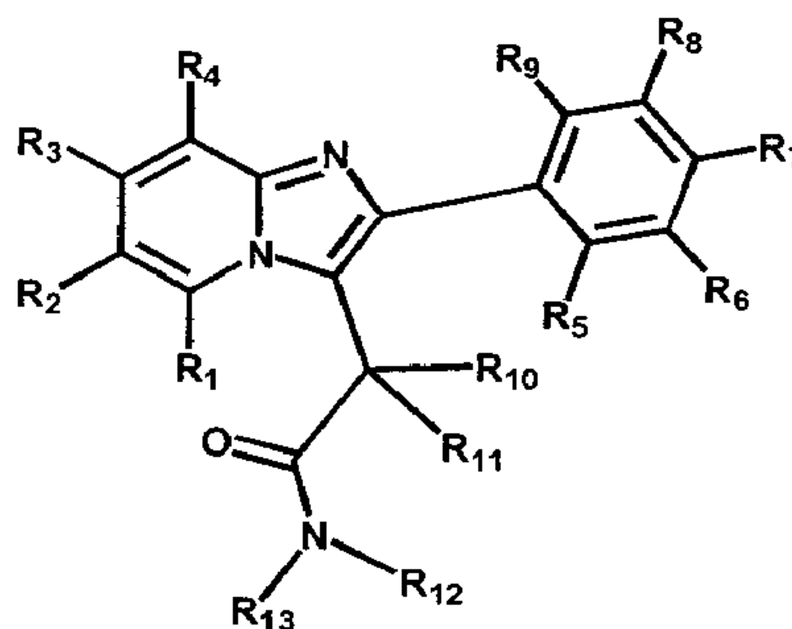
Formula 1
