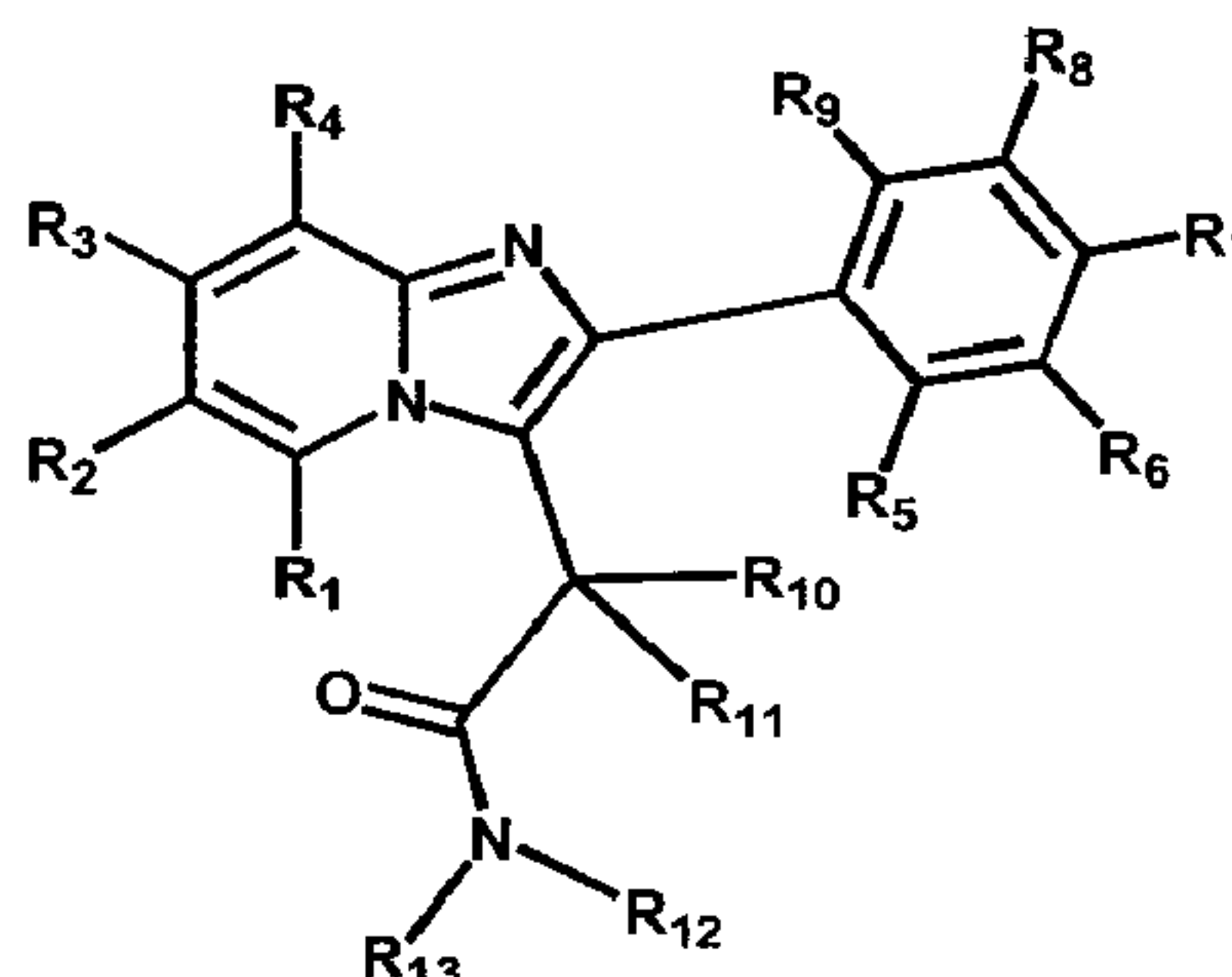
Formula 1
