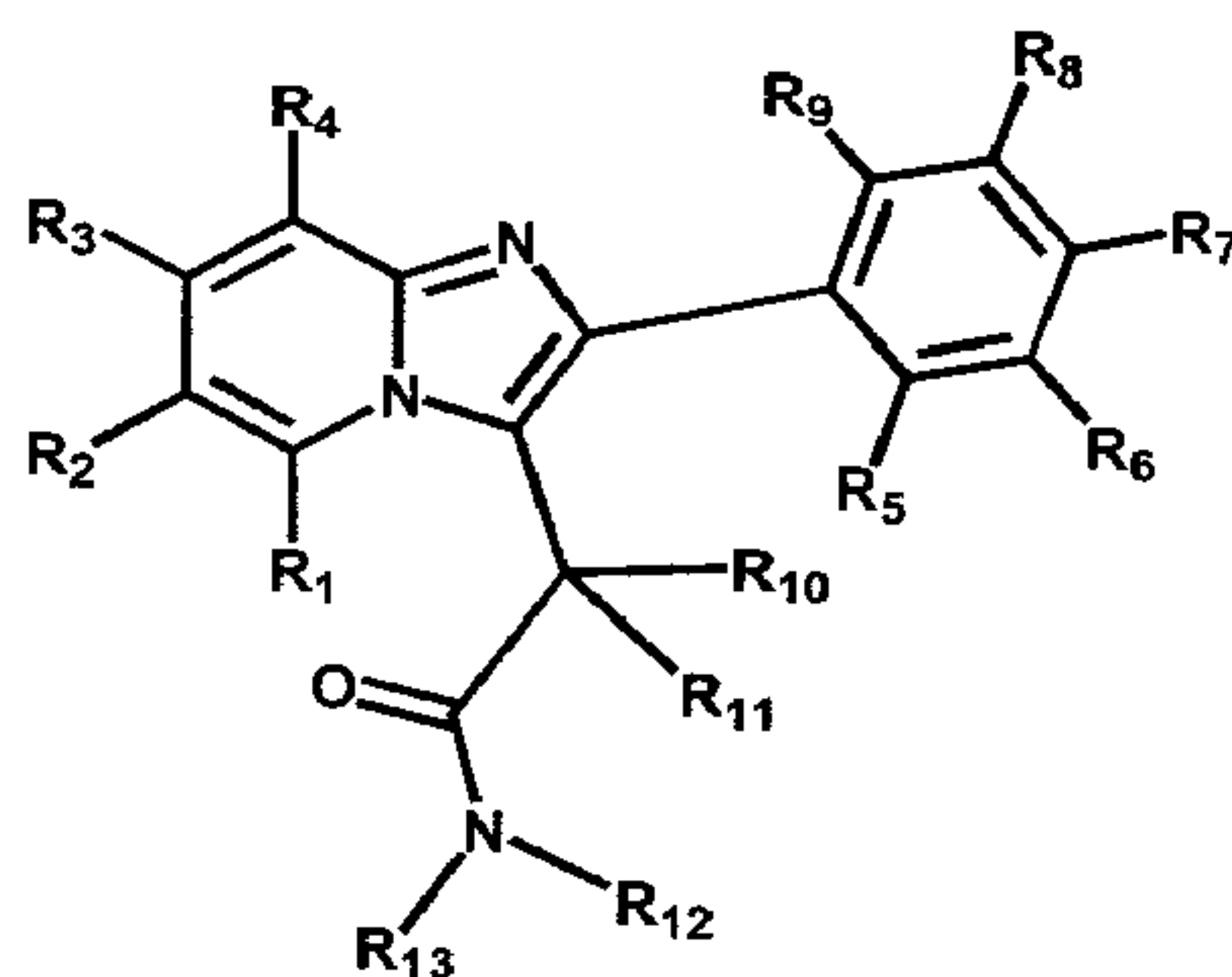
Formula 1
