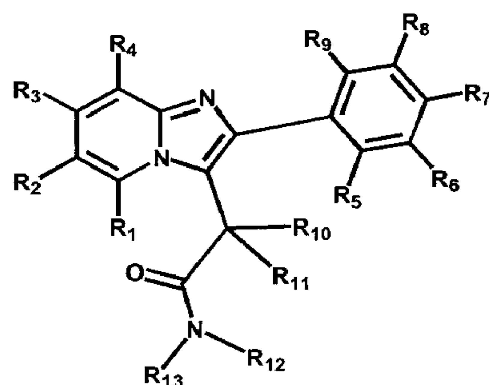
Formula 1
