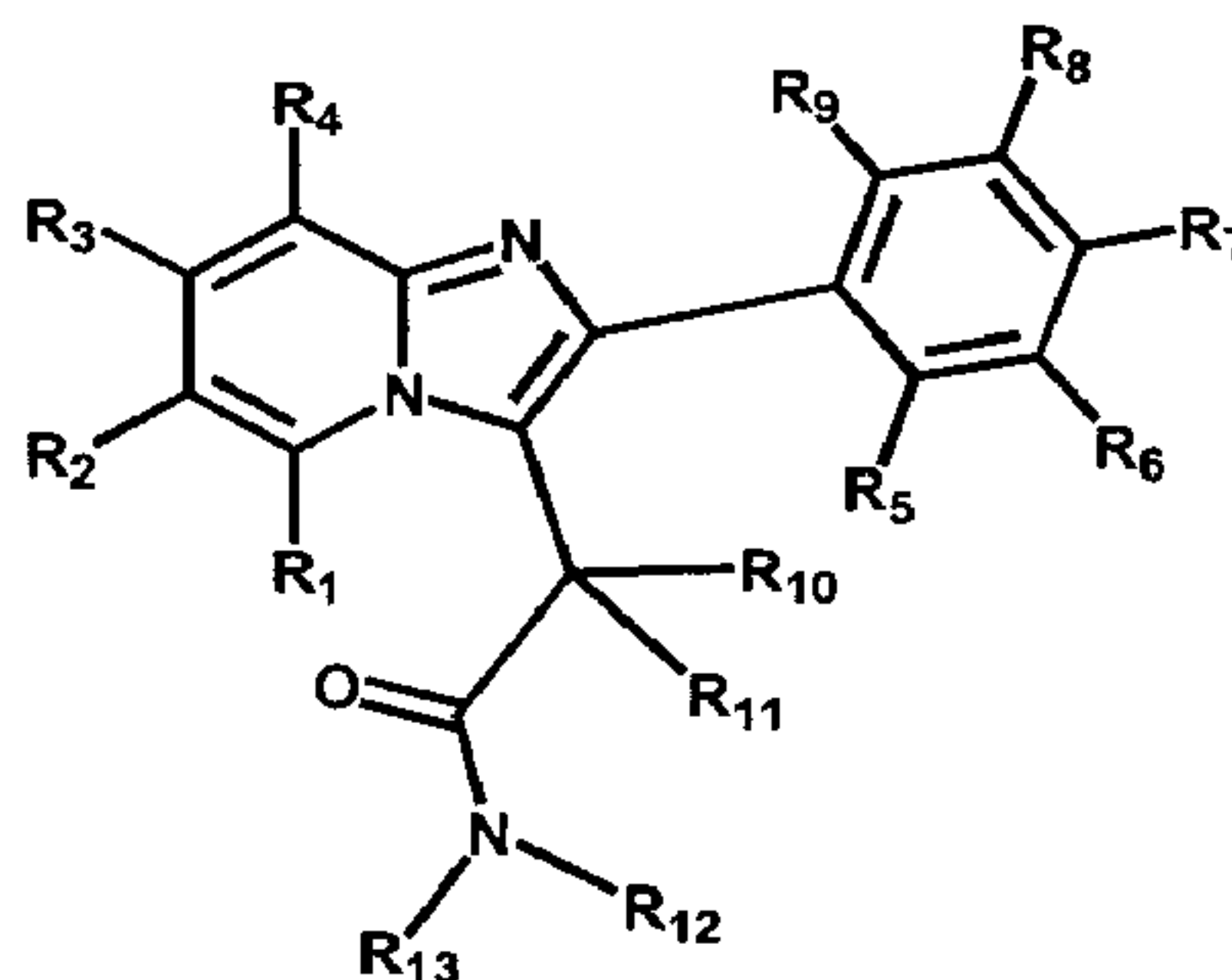
Formula 1
