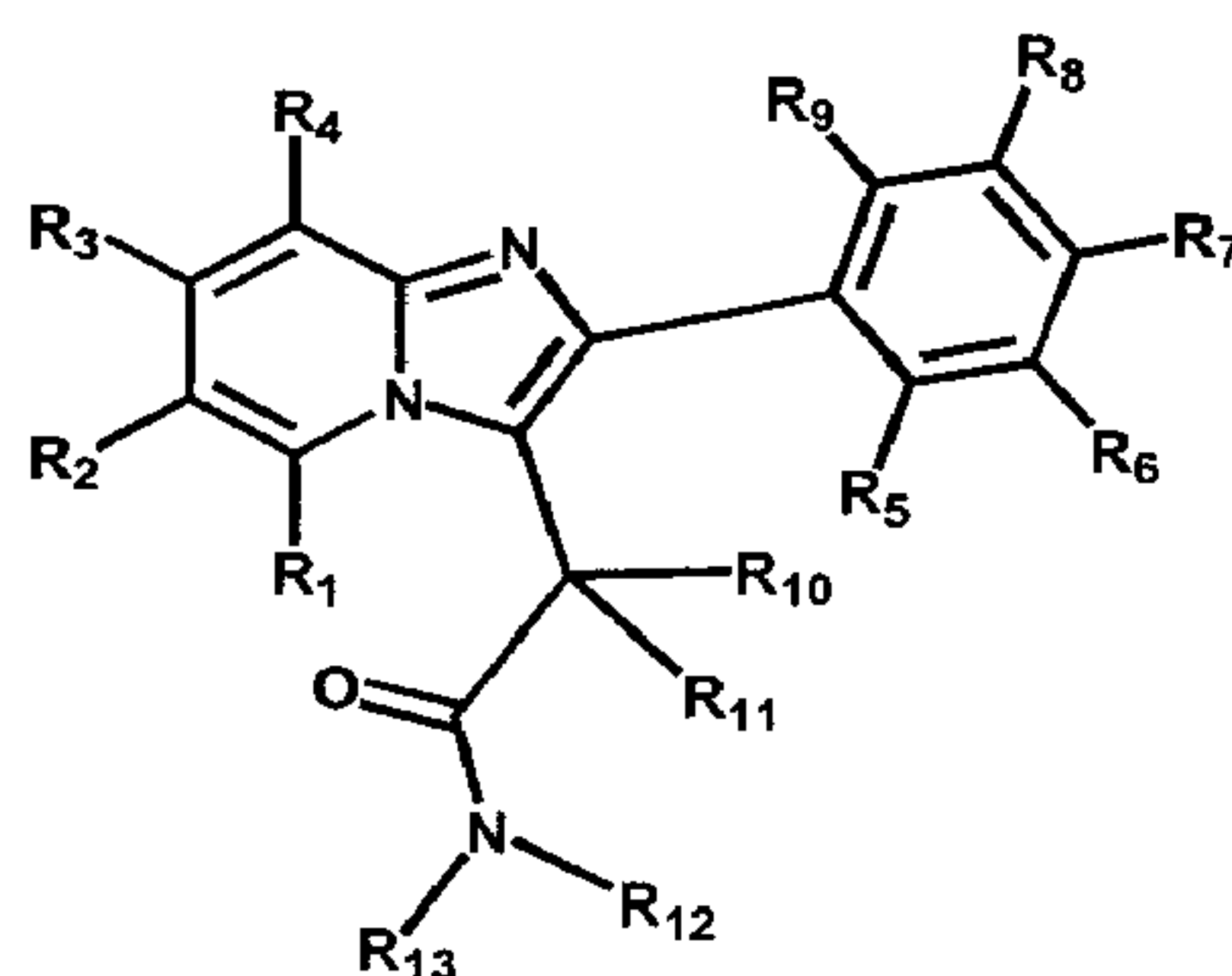
Formula 1
