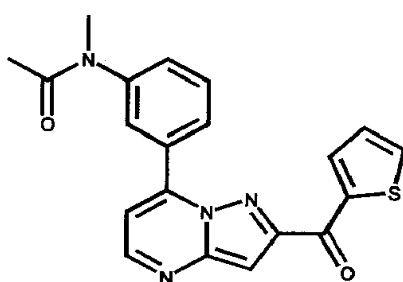
Indiplon
