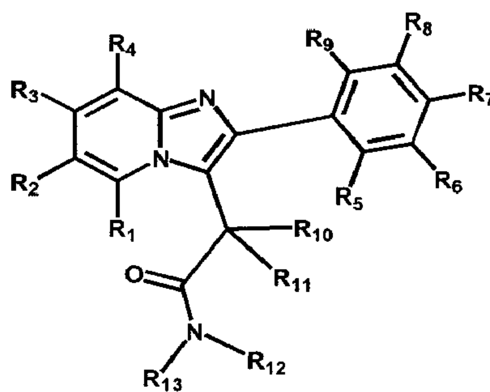
Formula 1
