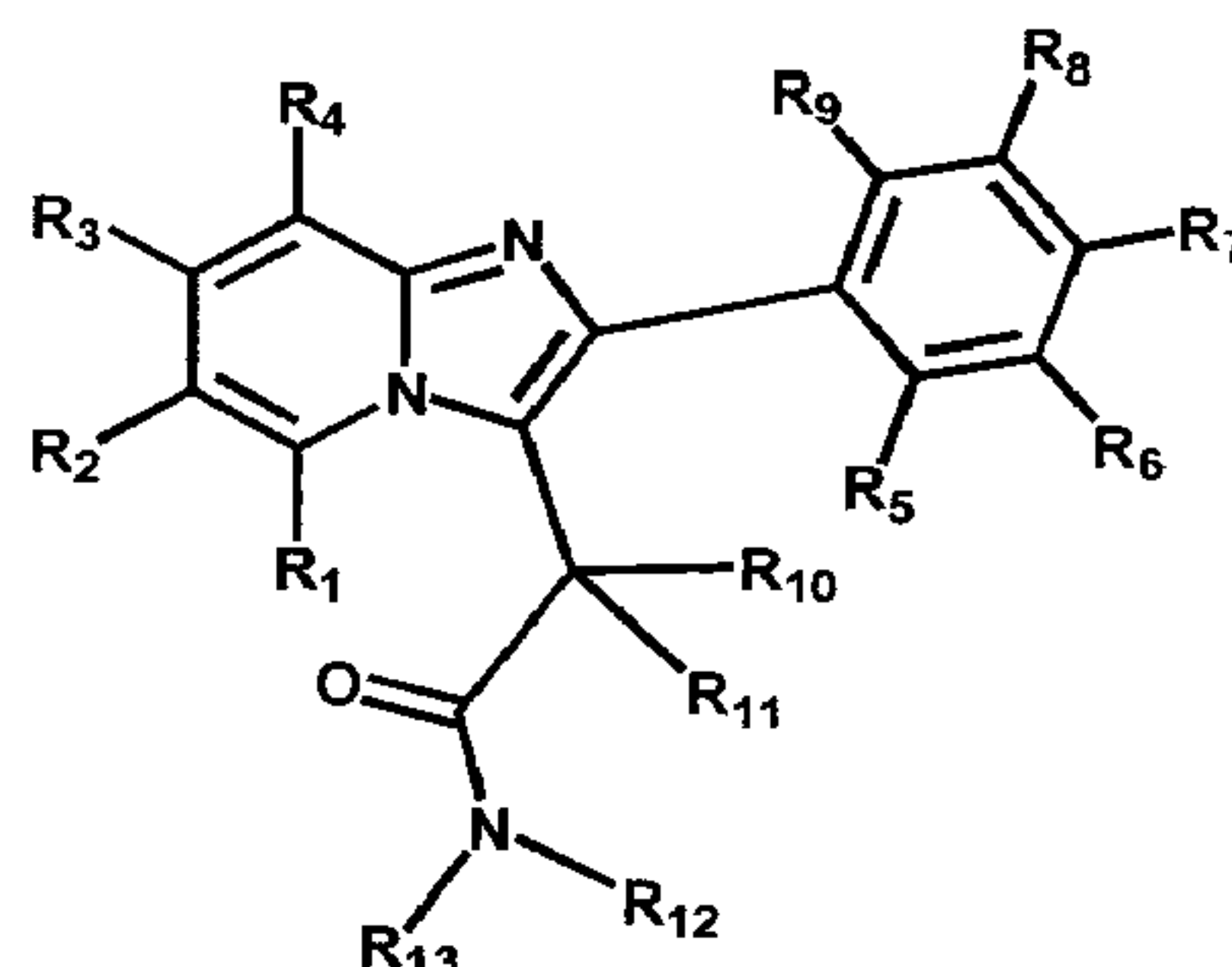
Formula 1
