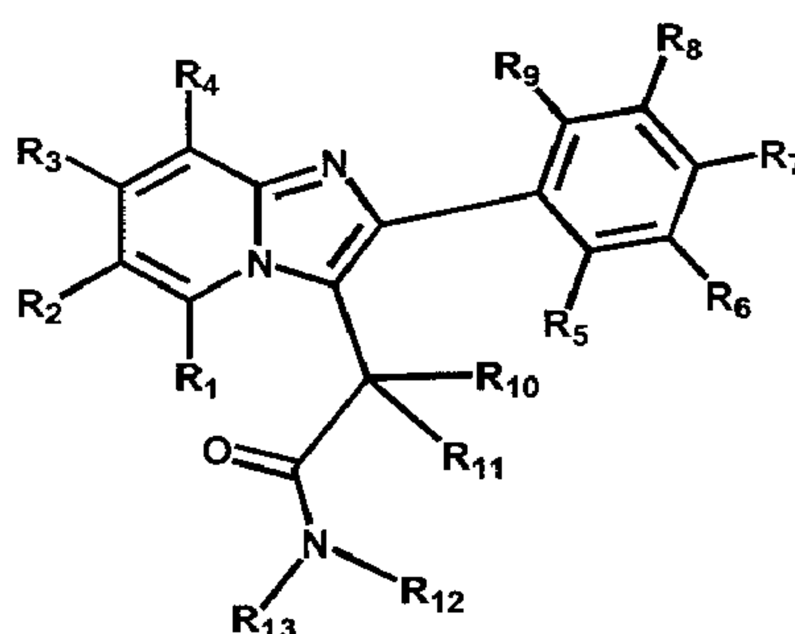
Formula 1
