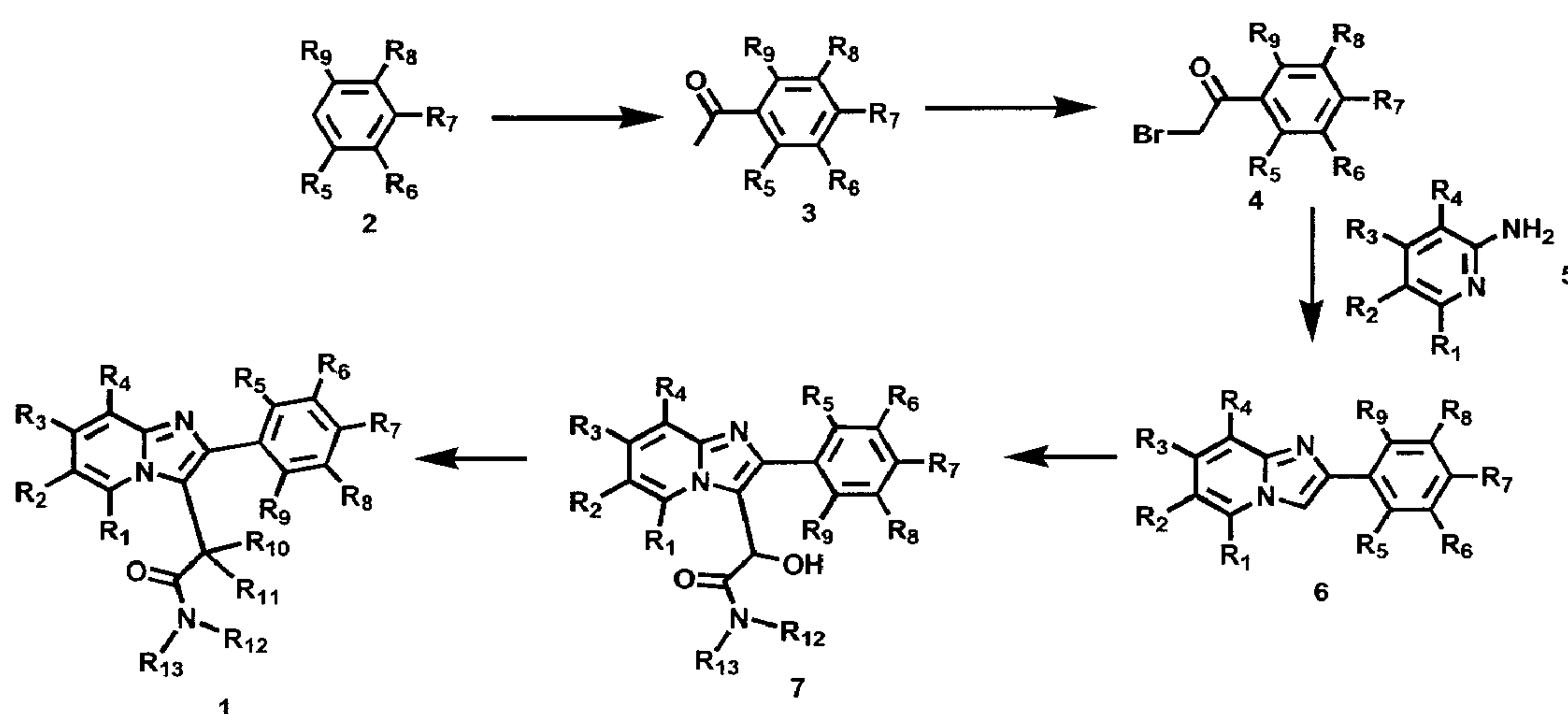
Scheme 1
