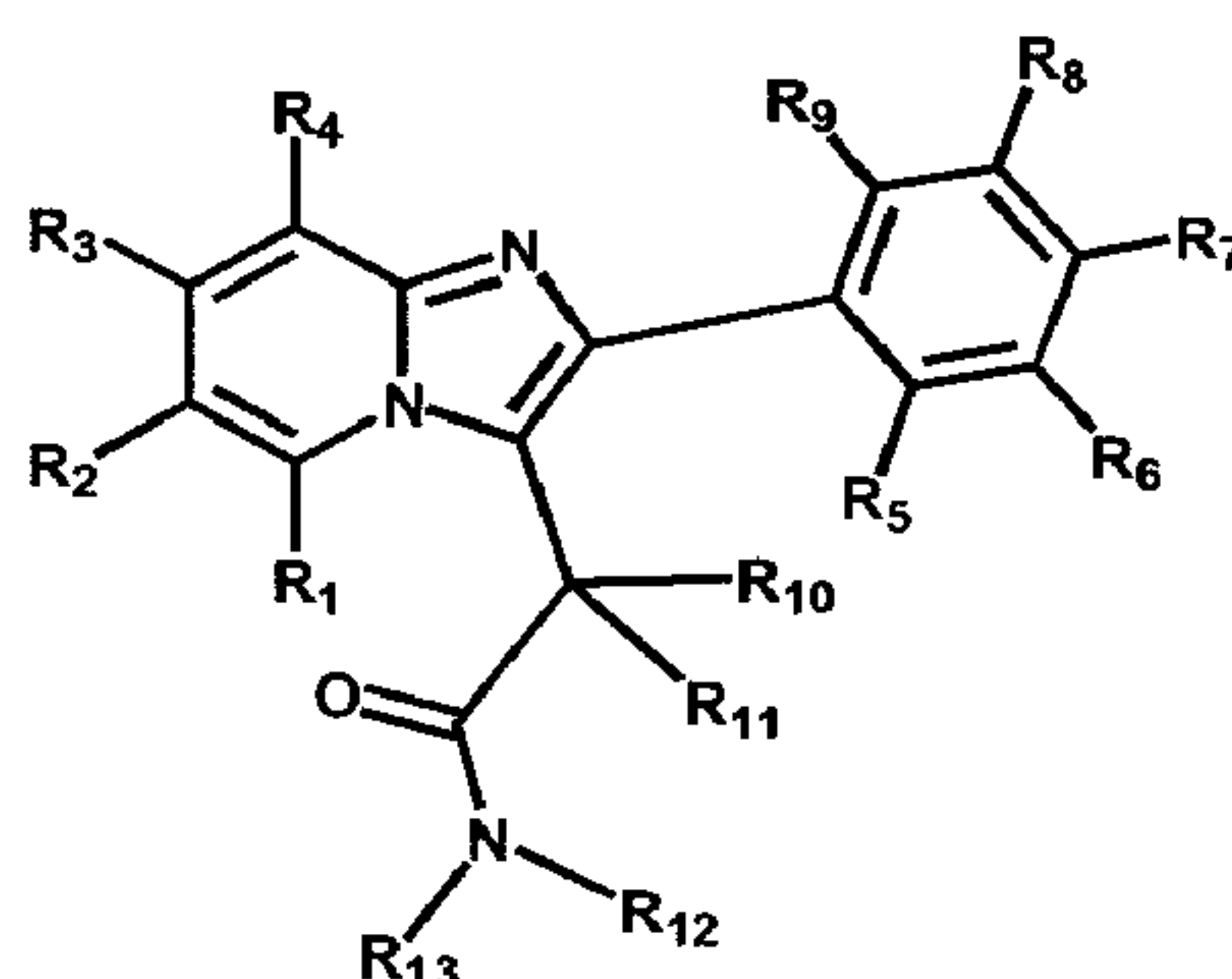
Formula 1
