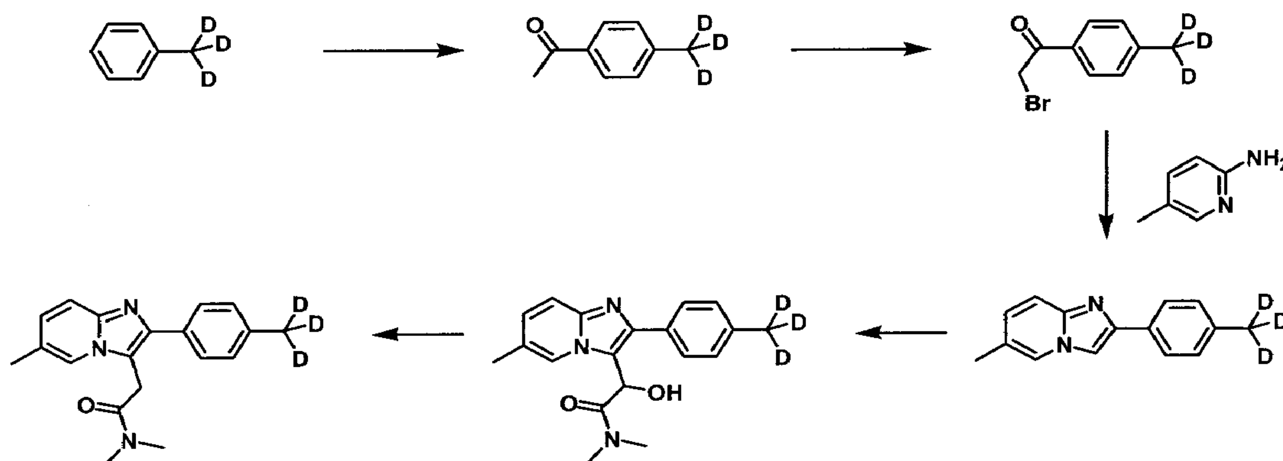
Scheme 1.
