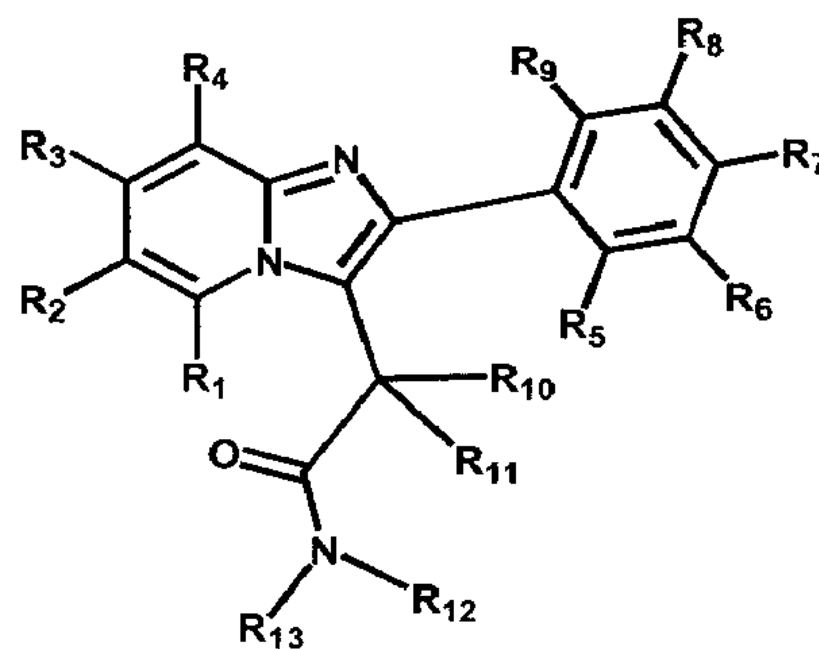
Formula 1
