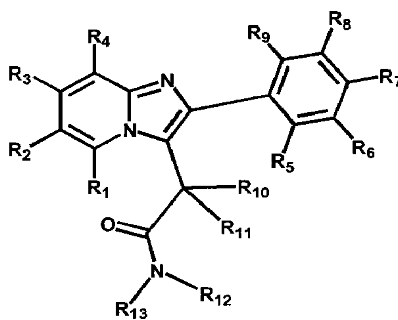
Formula 1
