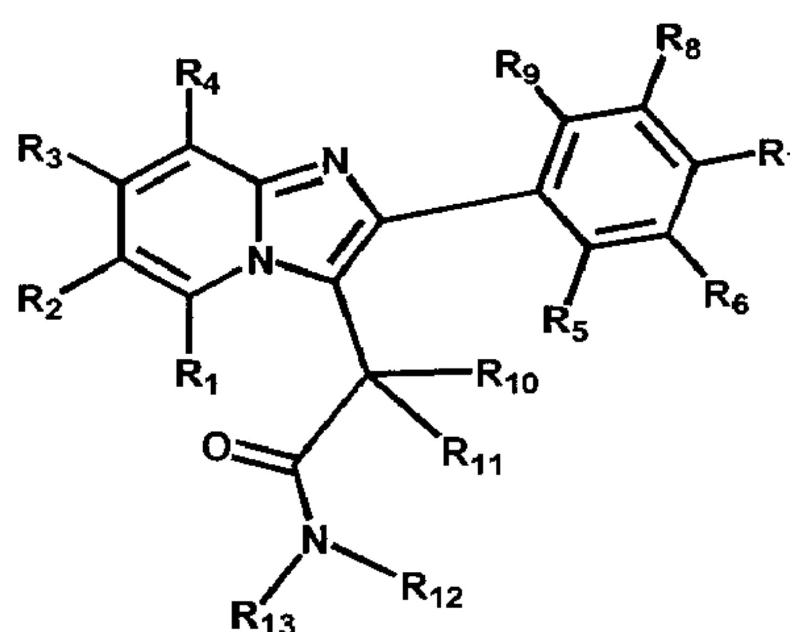
Formula 1
