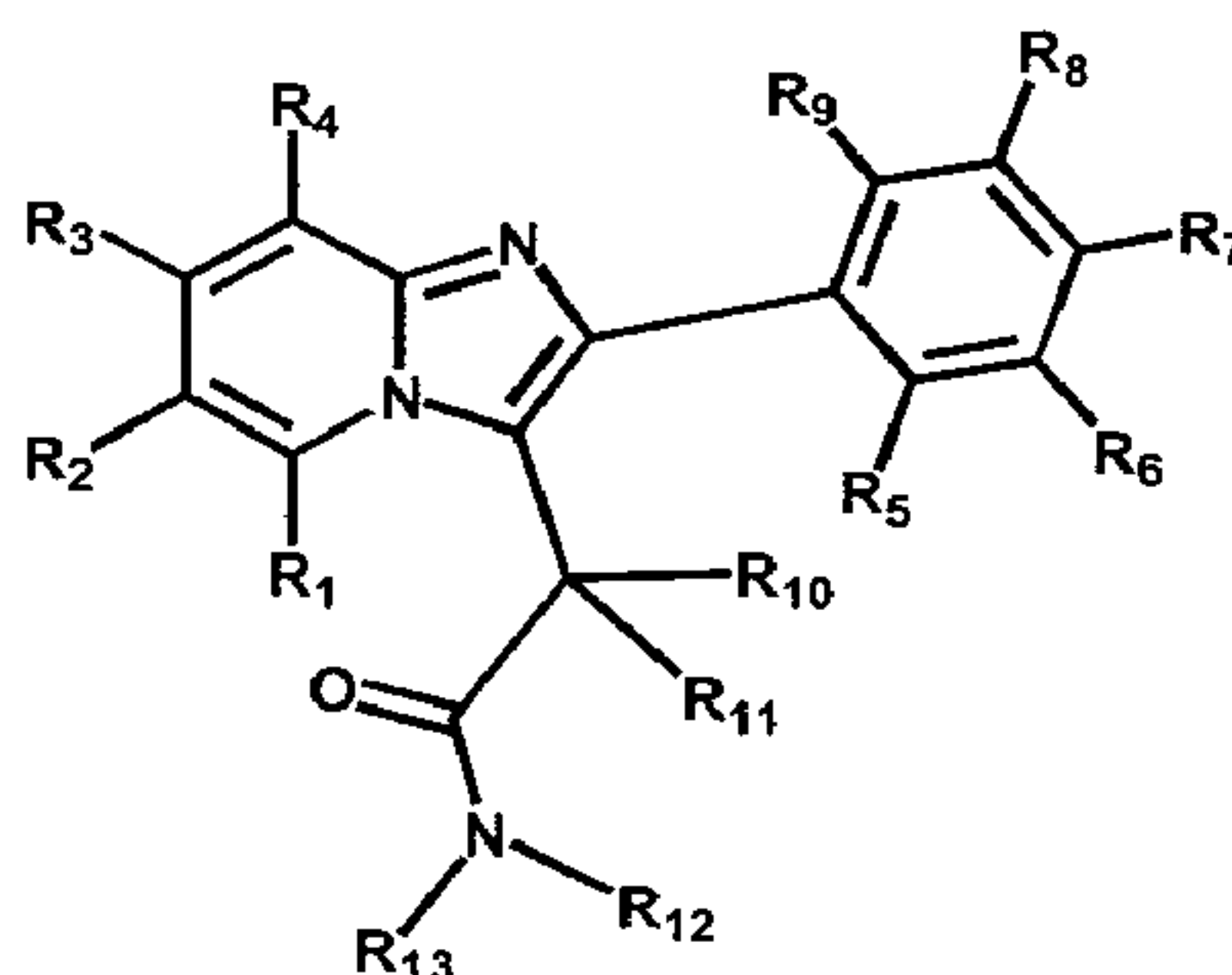
Formula 1
