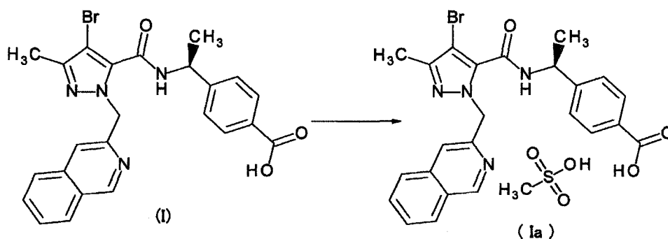
[Chem. 16]
