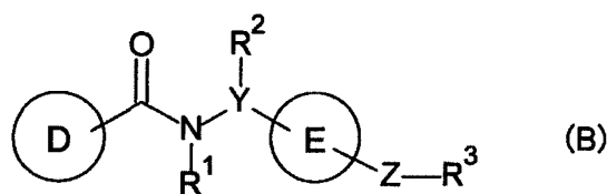
[Chem. 1]
