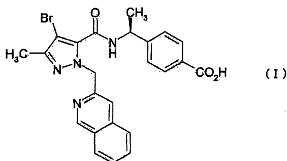
[Chem. 9]
