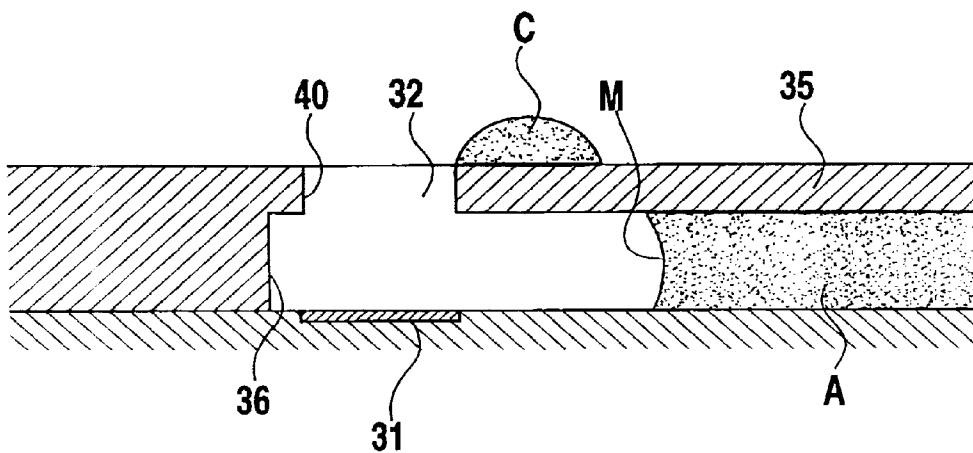
FIG. 19 PRIOR ART
