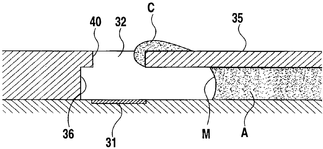
FIG. 20 PRIOR ART
