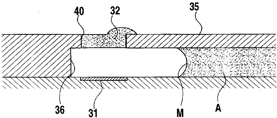
FIG. 21 PRIOR ART
