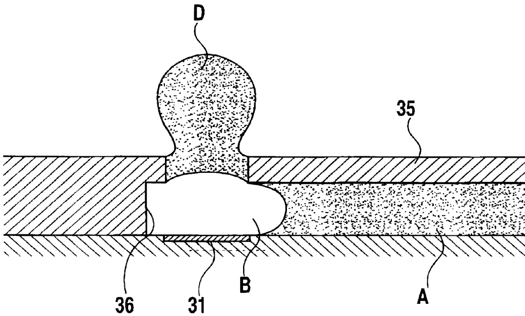
FIG. 17 PRIOR ART
