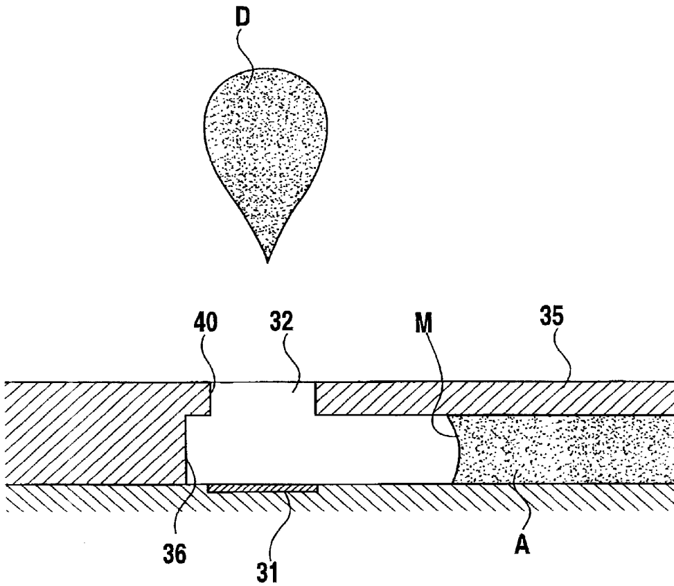
FIG. 18 PRIOR ART
