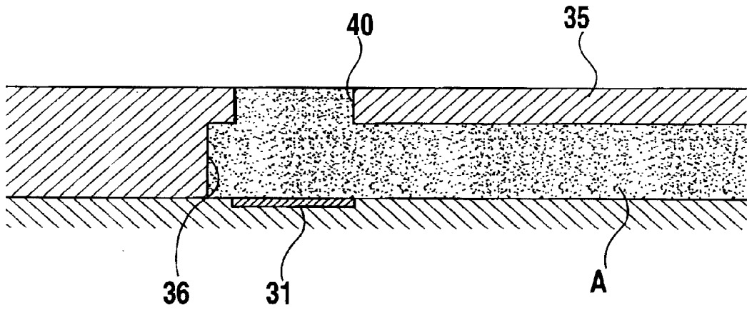
FIG. 16 PRIOR ART
