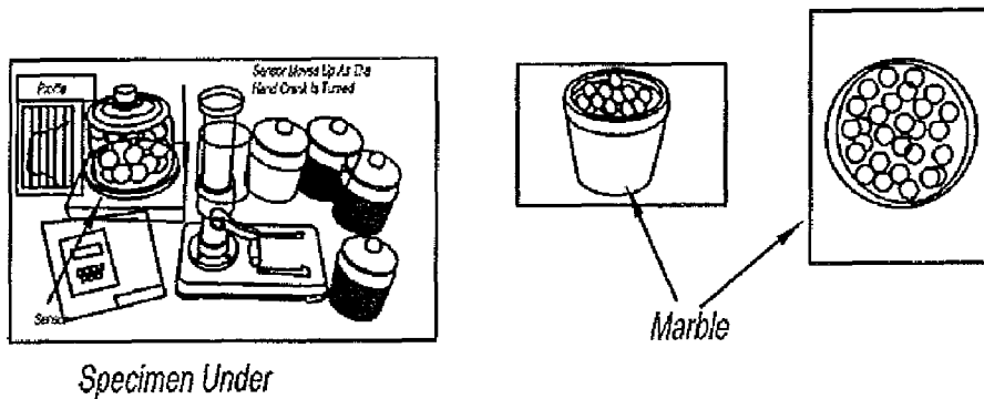
The laboratory equipment used to inspect the gelatin specimens. Each specimen is filled with a marble + gelatin + tagged material.
