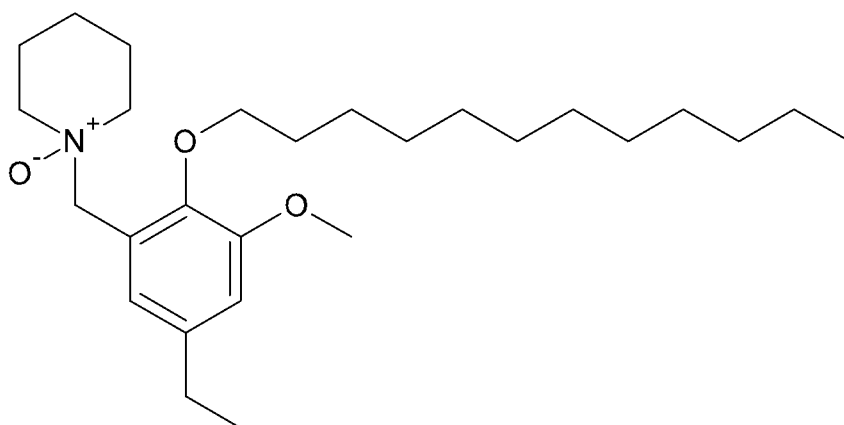
1-(2-dodecyloxy-5-ethyl-3-methoxybenzyl)piperidine-1-oxide (8)
