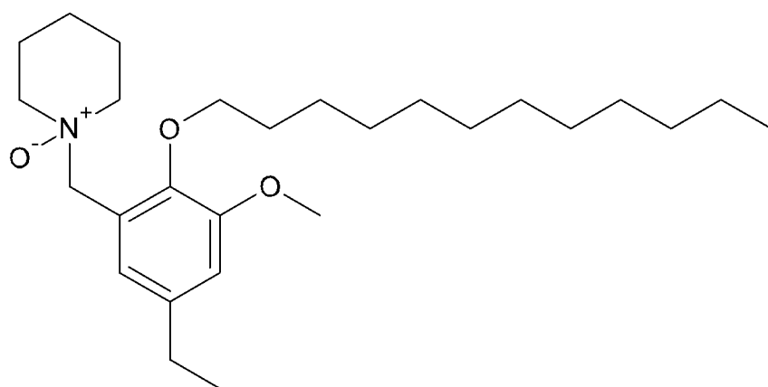
5 1-(2-dodecyloxy-5-ethyl-3-methoxybenzyl)piperidine-1-oxide (8)
