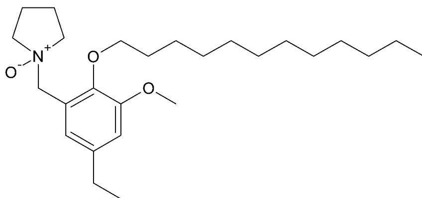
1-(2-dodecyloxy-5-ethyl-3-methoxybenzyl)pyrrolidine-1-oxide (7)
