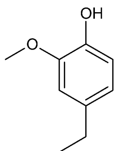
4-ethylguaiacol
