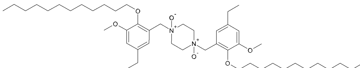
1,4-bis(2-dodecyloxy-5-ethyl-3-methoxybenzyl)piperazine-1,4-dioxide (17)
