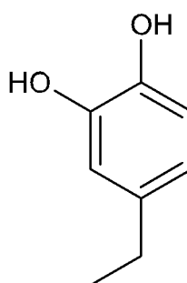
4-ethylcatechol
