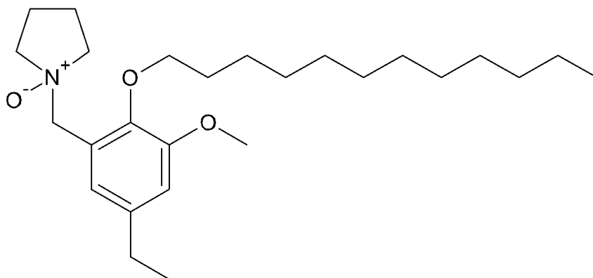
5 1-(2-dodecyloxy-5-ethyl-3-methoxybenzyl)pyrrolidine-1-oxide (7)
