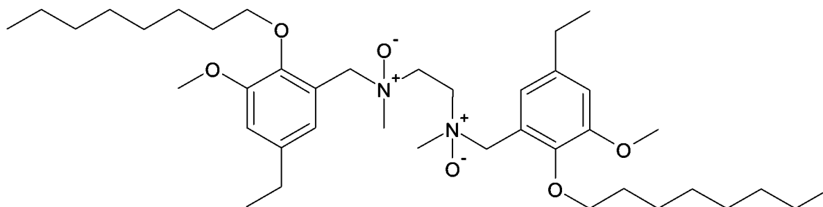
10 N,N'-bis(5-ethyl-3-methoxy-2-octyloxybenzyl)-N,N'-dimethylethane-1,2-diamine di-N-oxide (18)
