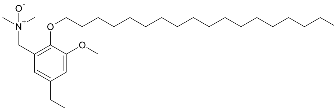
N,N-dimethyl-1-(5-ethyl-3-methoxy-2-octadecyloxyphenyl)methanamine N-oxide (6)
