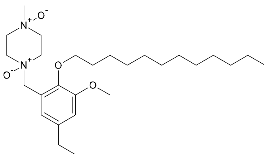
1-(2-dodecyloxy-5-ethyl-3-methoxybenzyl)-4-methylpiperazine-1,4-dioxide (9)
