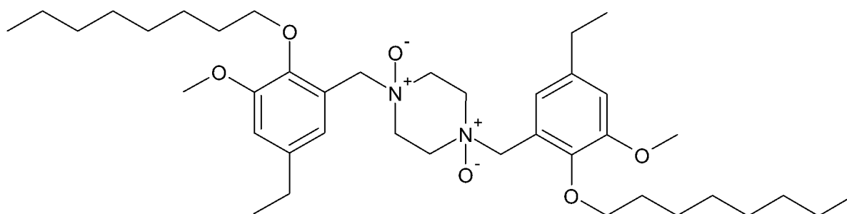
1,4-bis(5-ethyl-3-methoxy-2-octyloxybenzyl)piperazine-1,4-dioxide (16)
