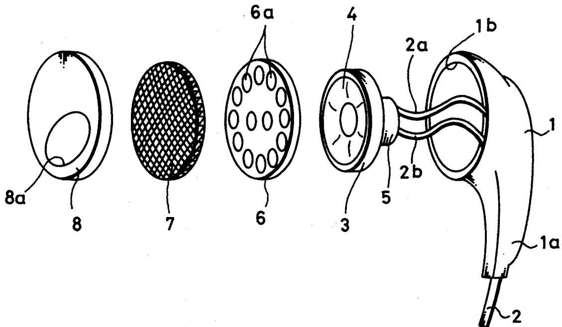
FIGURE 2 (PRIOR ART)
