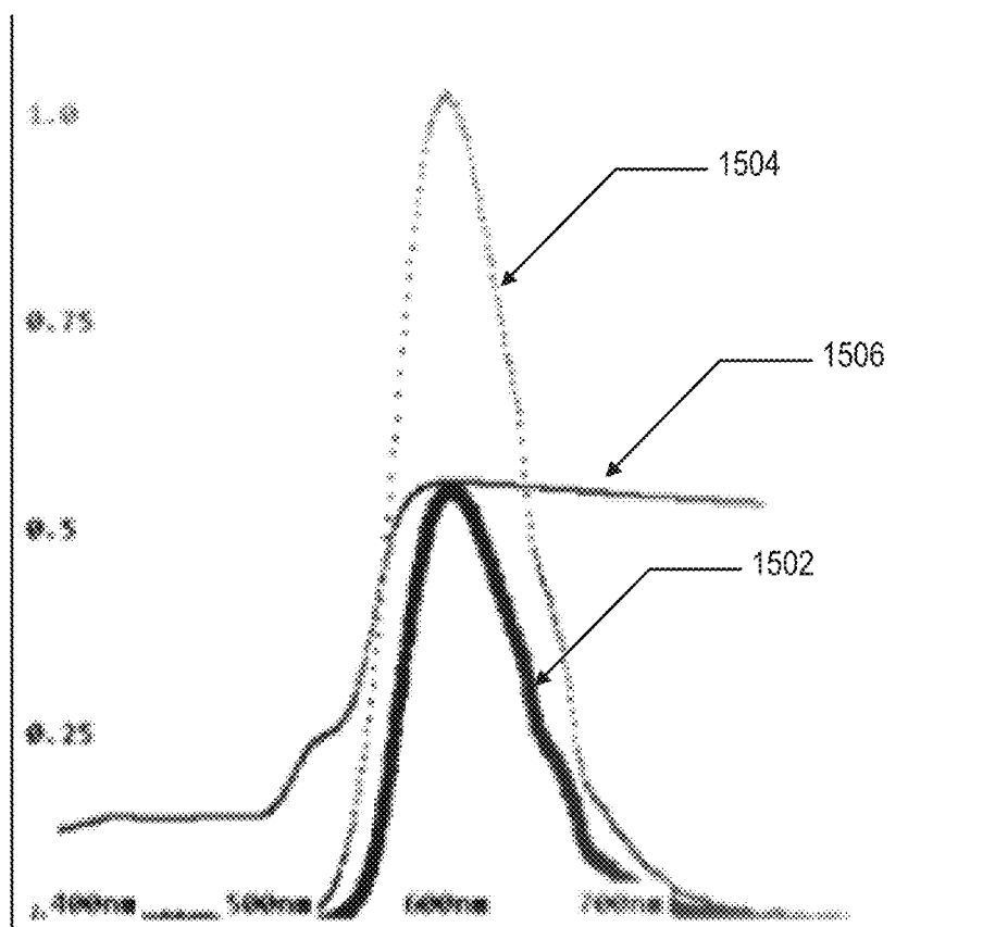
Integrating Response Profile Over Visible Spectrum (~400-700 nm)
