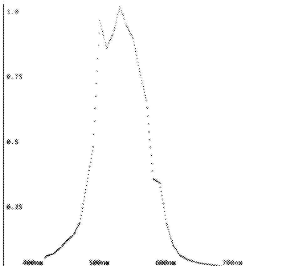
Sensor Response Over Visible Spectrum (~400-700 nm)
