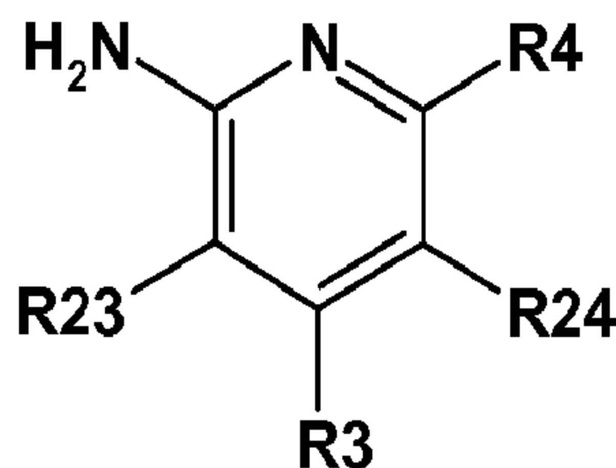
Formula (12).
