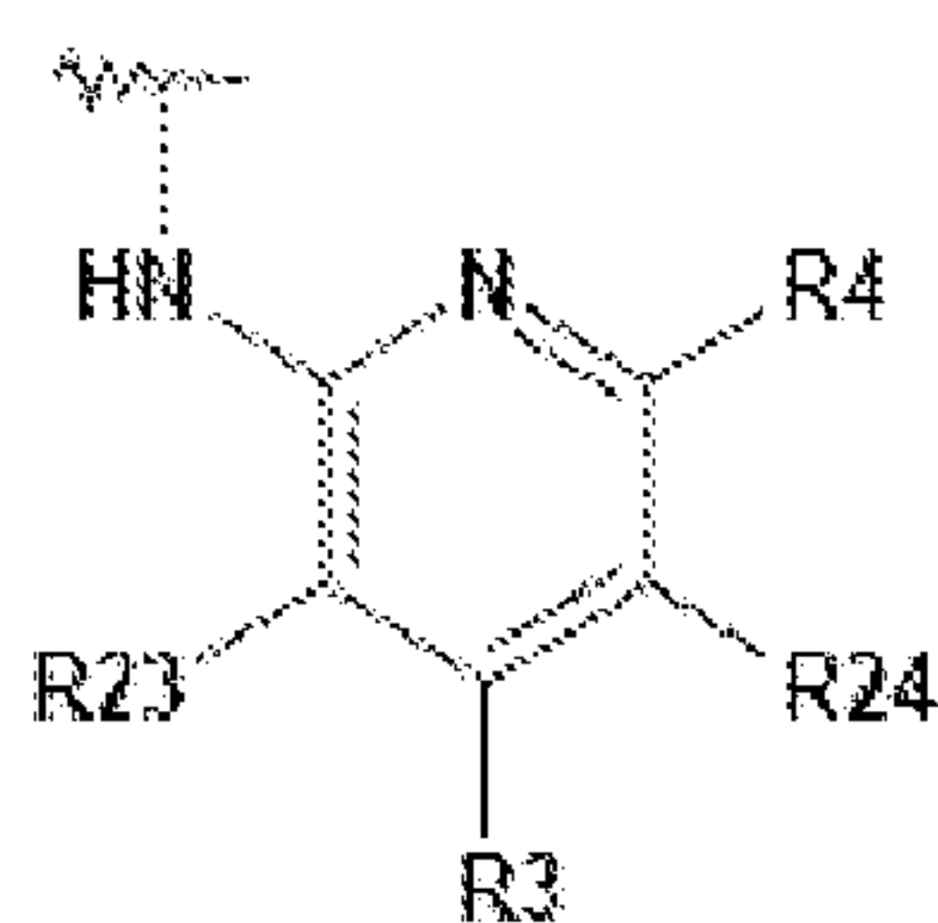
Formula (3)
