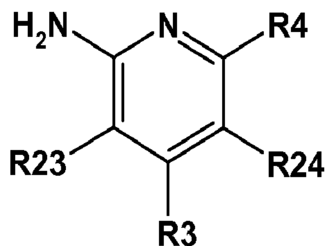
Formula (12)
