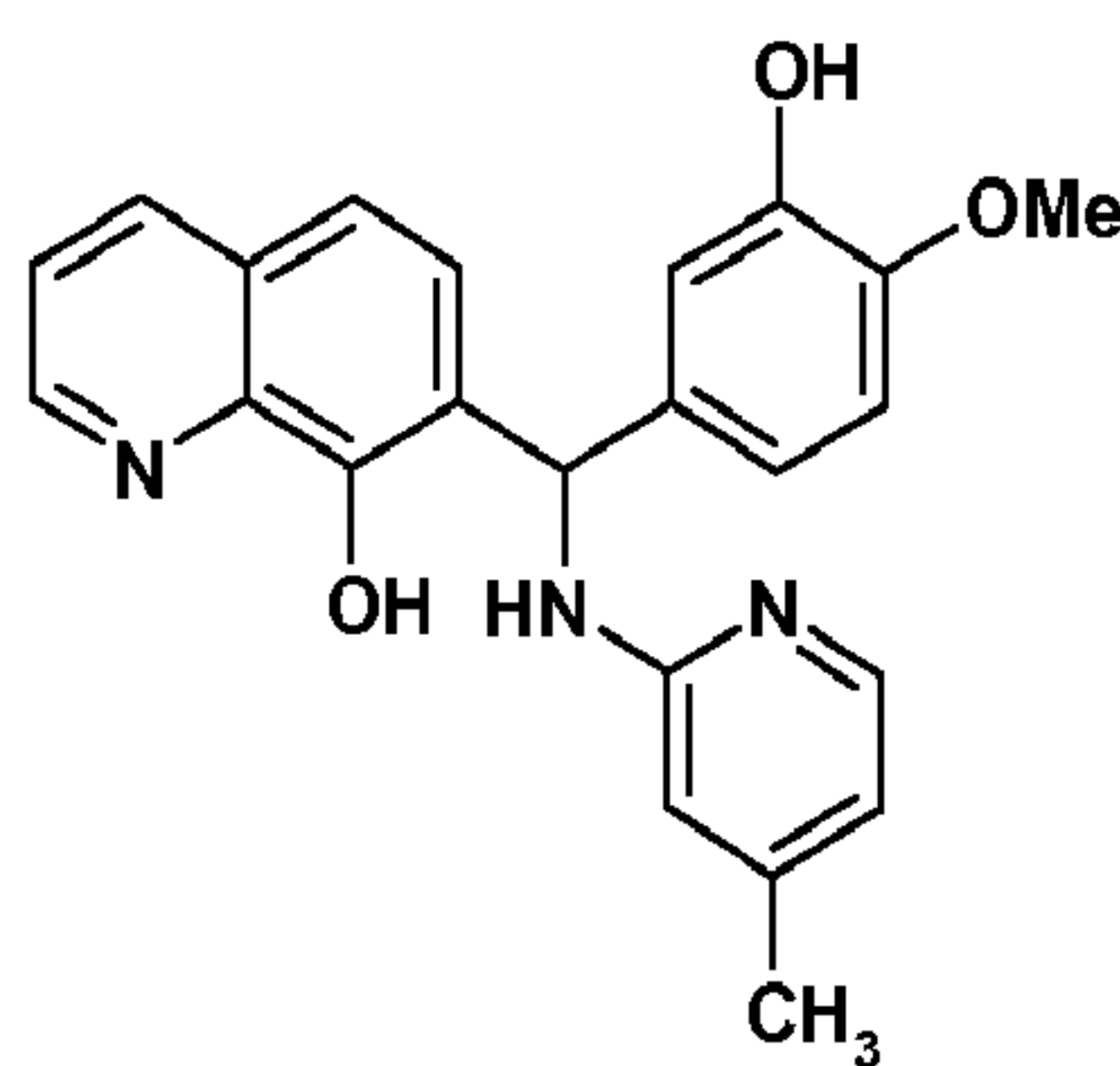
Formula (1).
