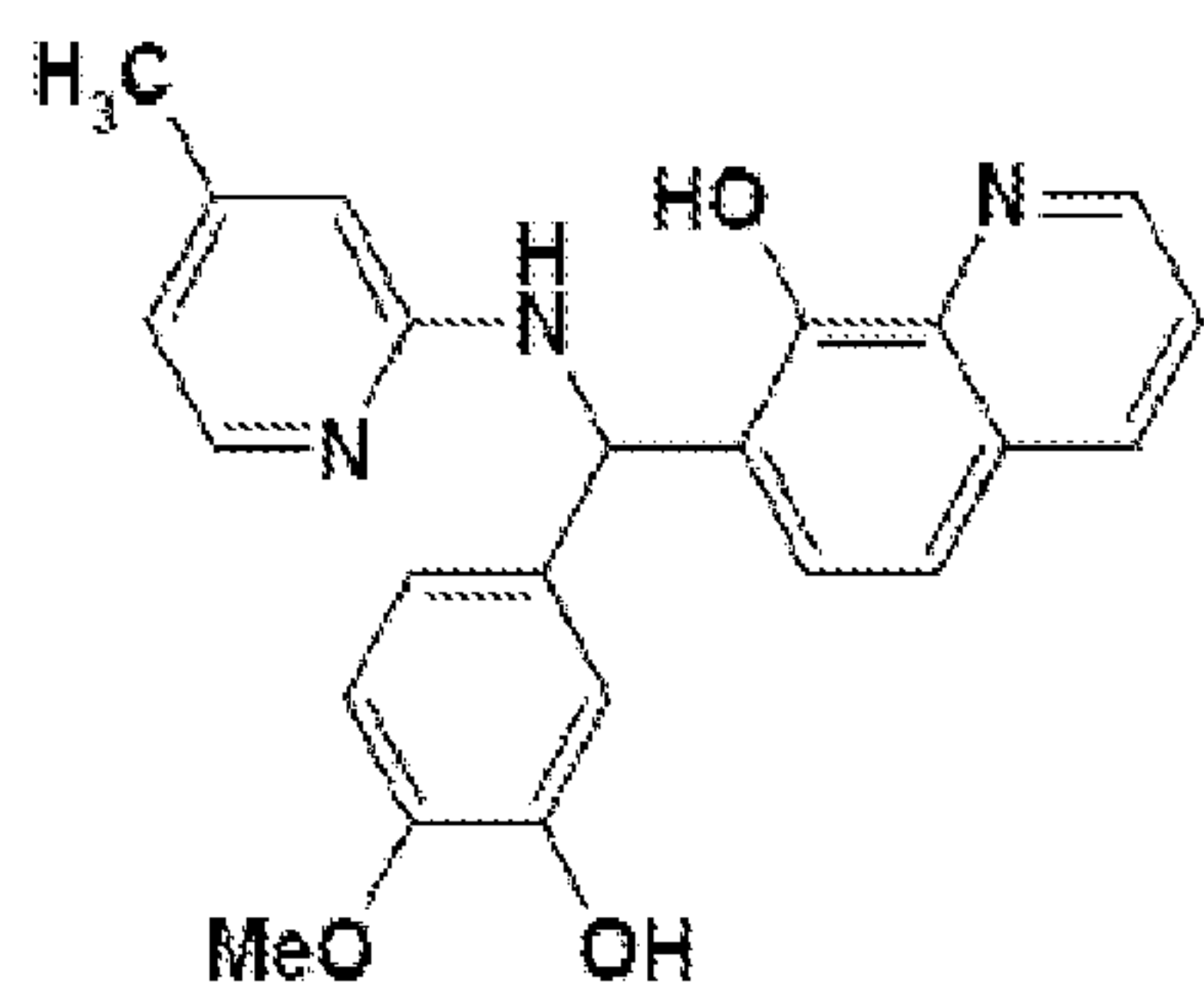
AD4-1505, Formula (1)
