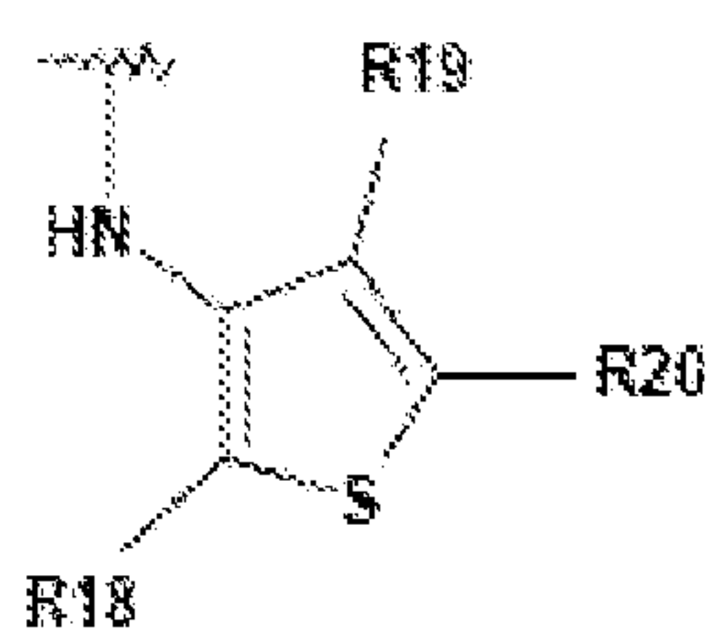
Formula (9);
