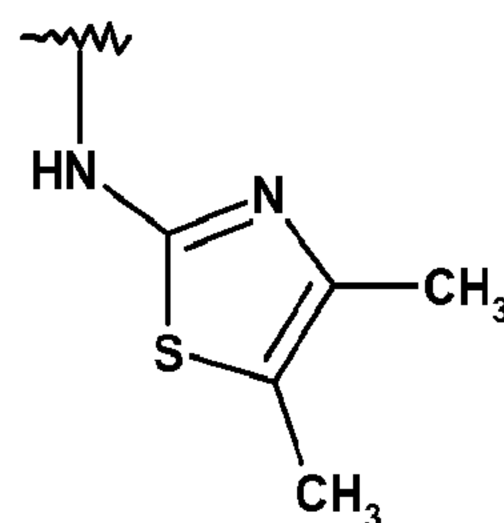
2-(4,5-DIMETHYL-1,3-THIAZOYL) GROUP
