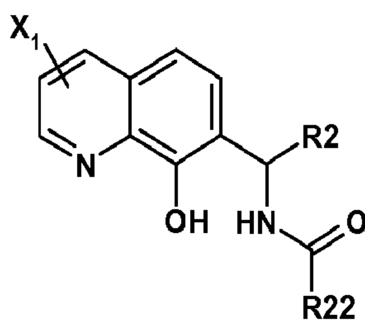
Formula (11)
