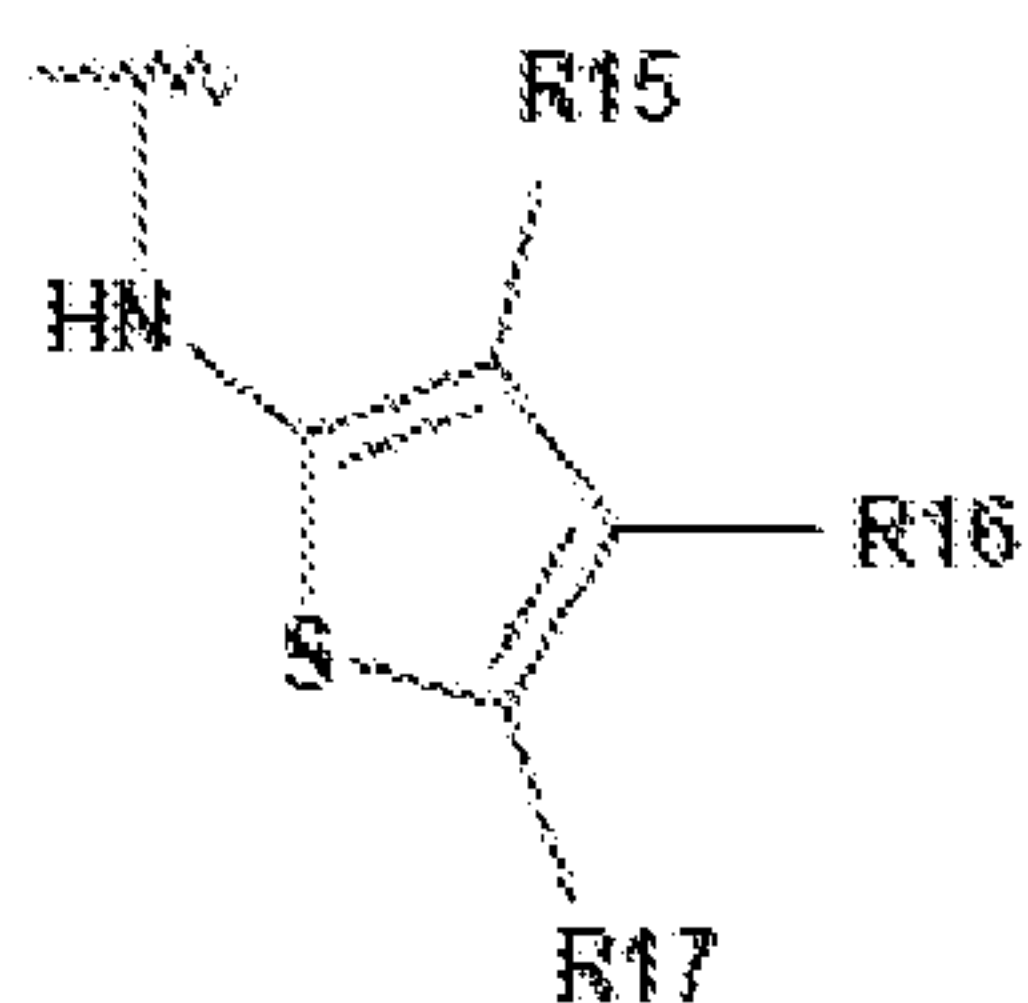
Formula (8);
