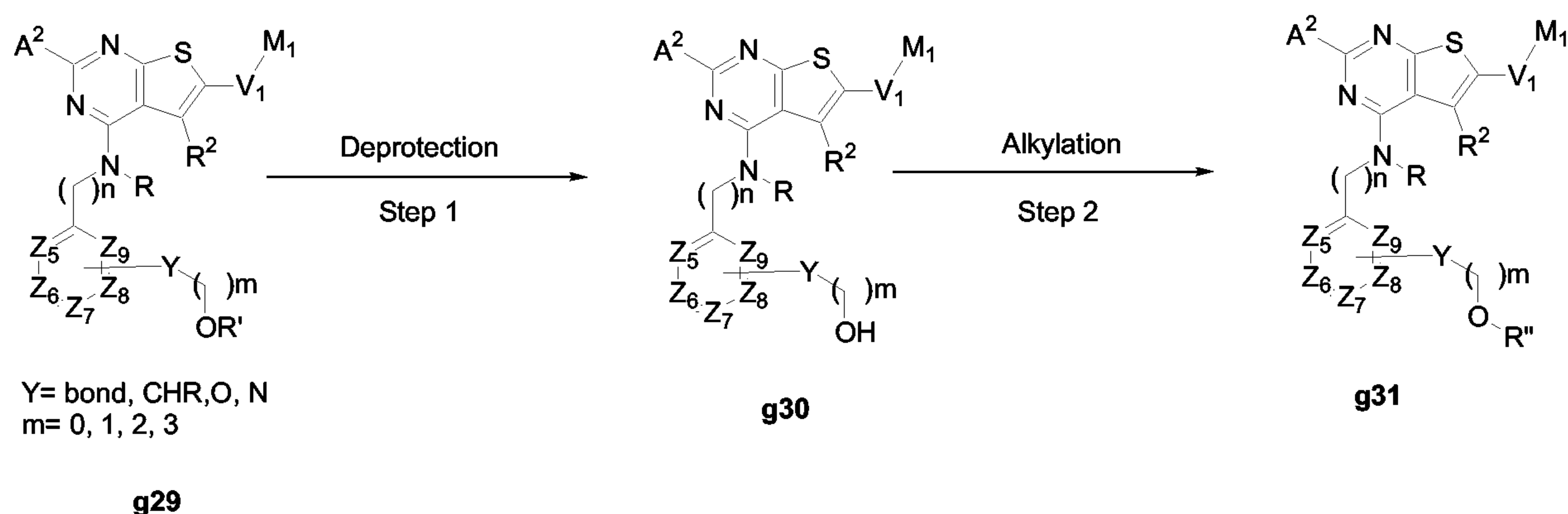
Scheme 13
