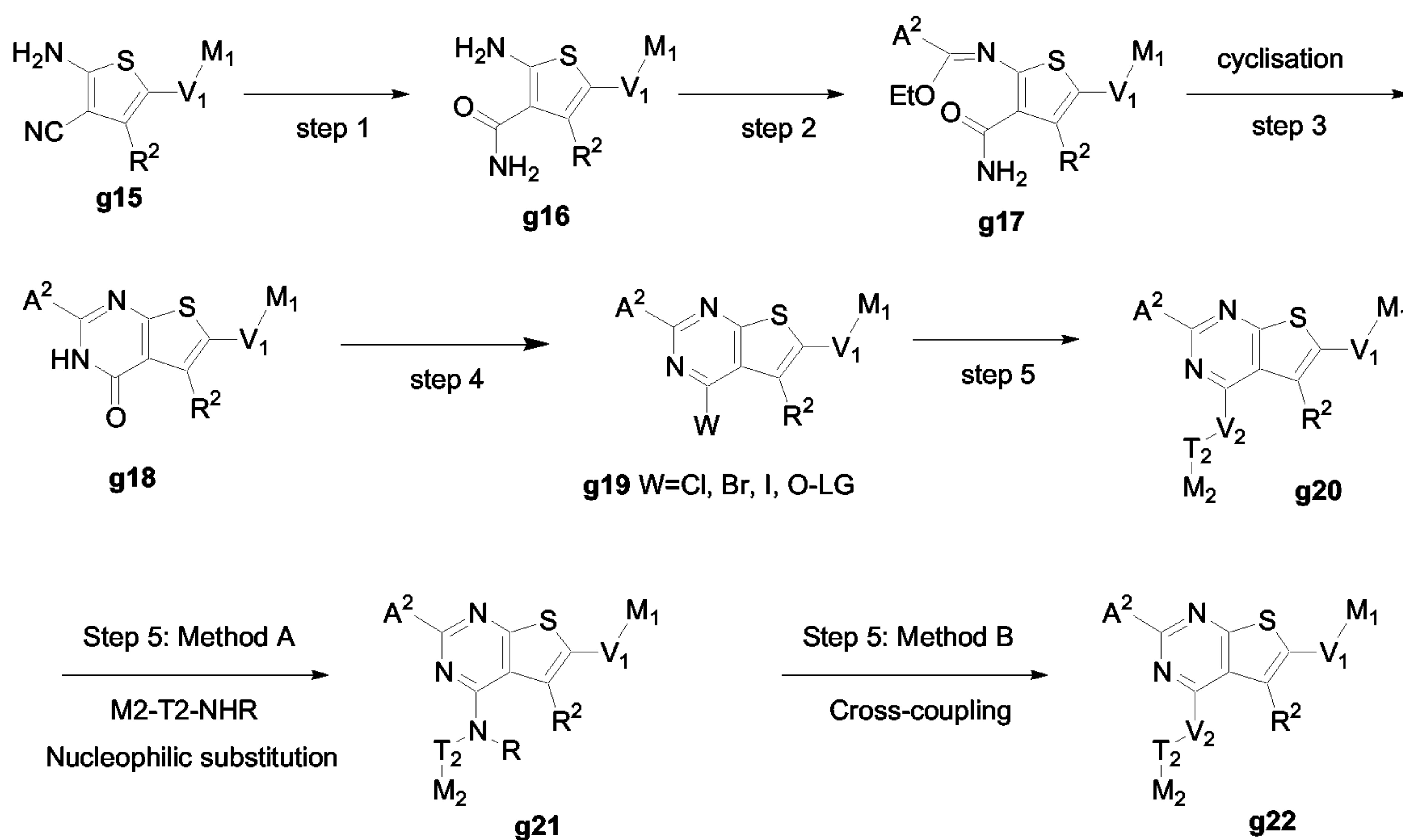
Scheme 5
