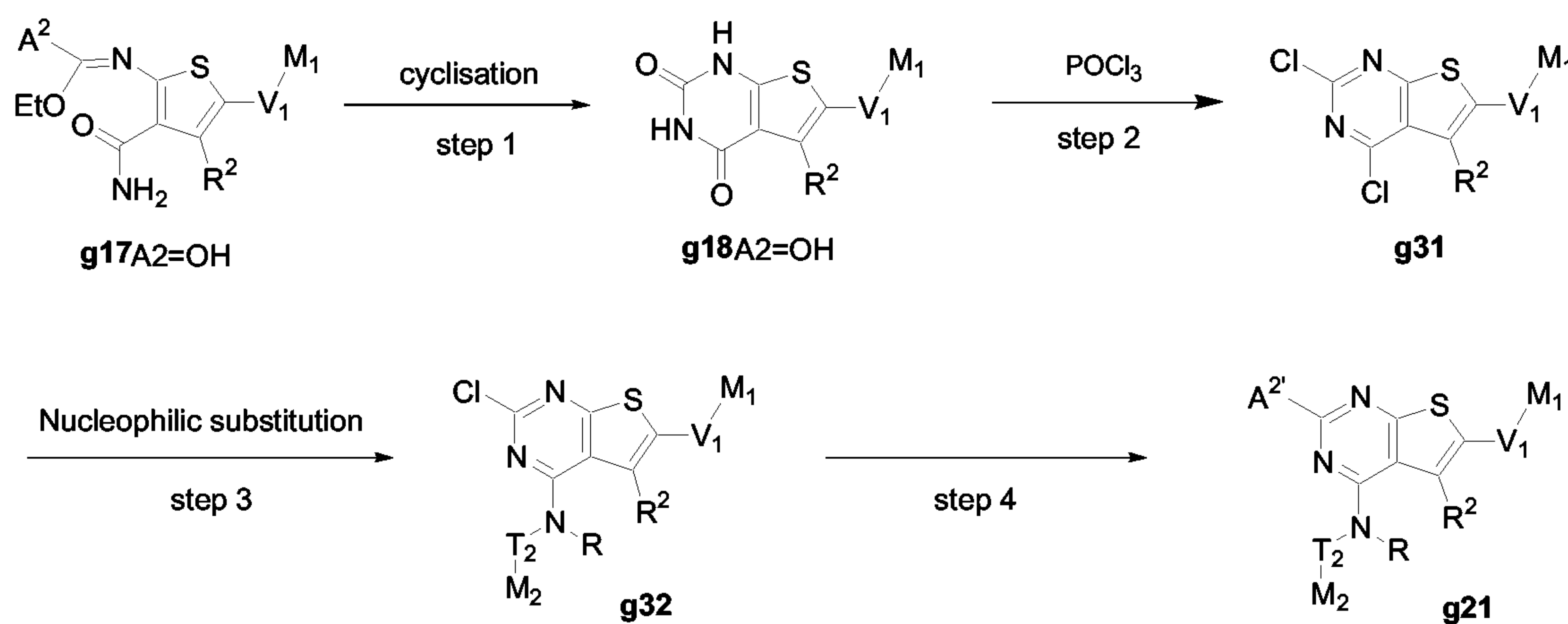
Scheme 10
