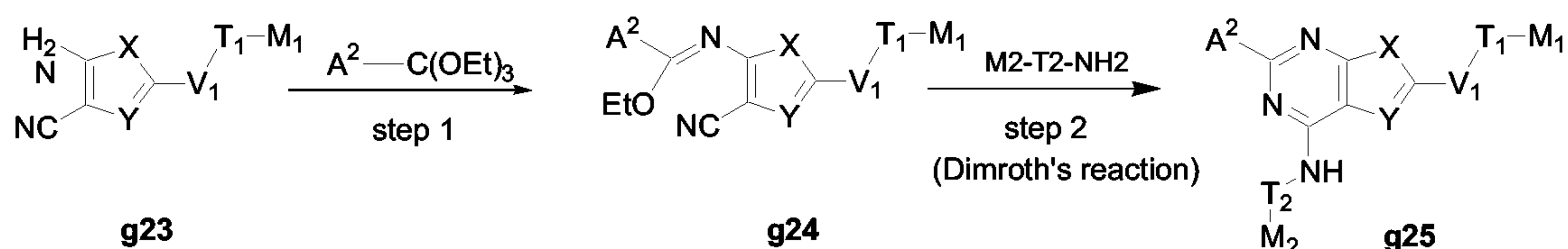
Scheme 6
