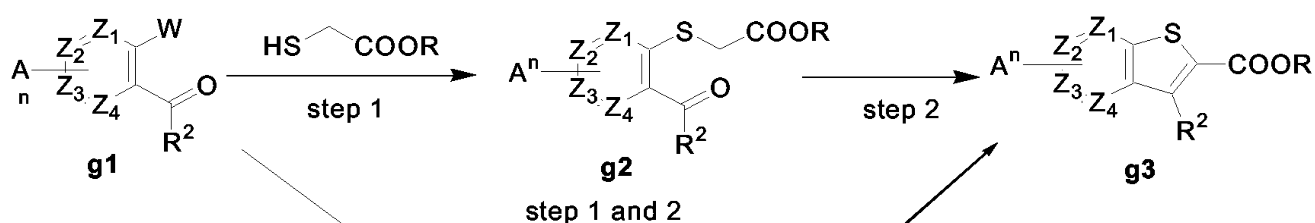
Scheme 1
