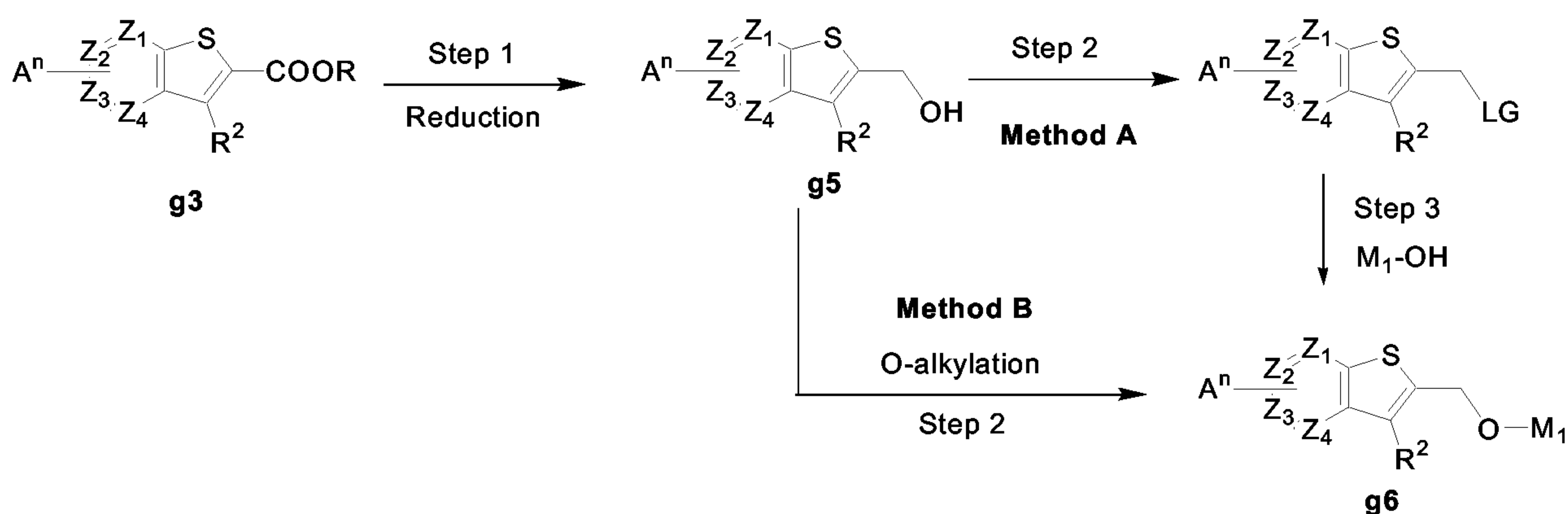
Scheme 2
