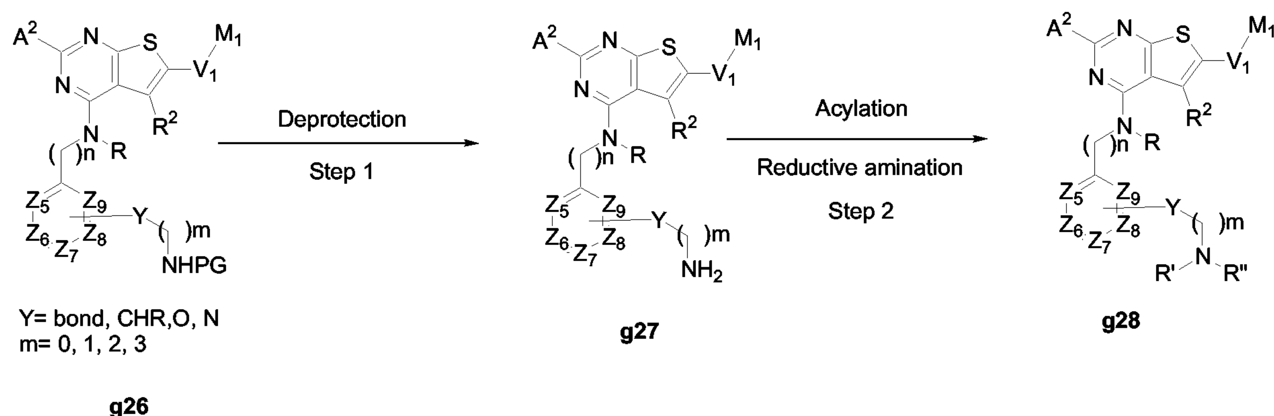
Scheme 12
