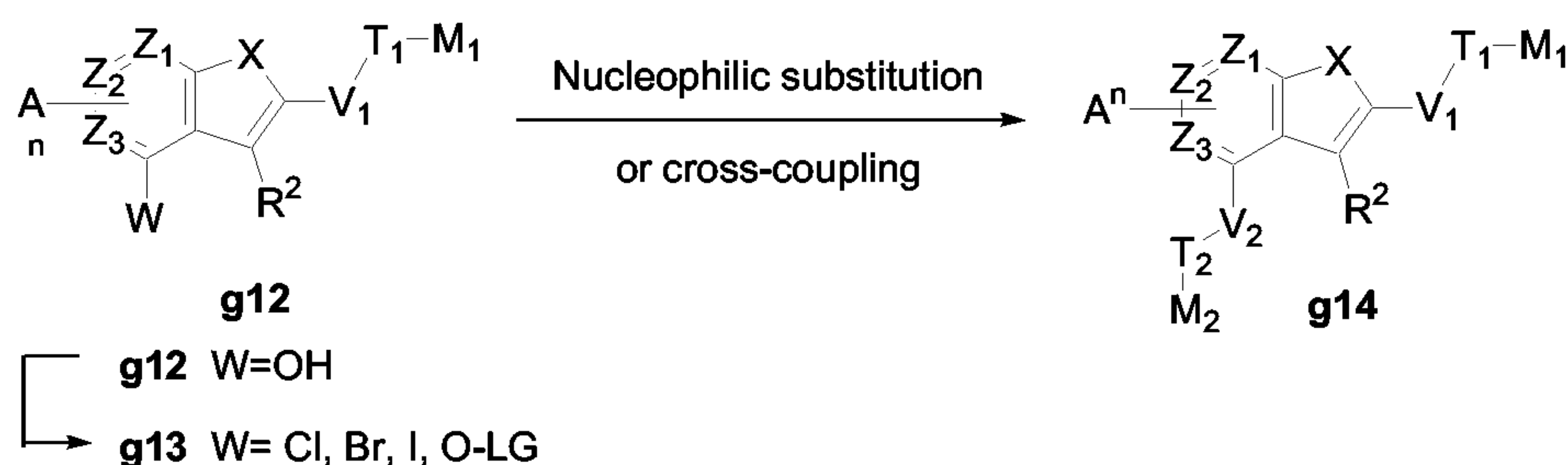
Scheme 4
