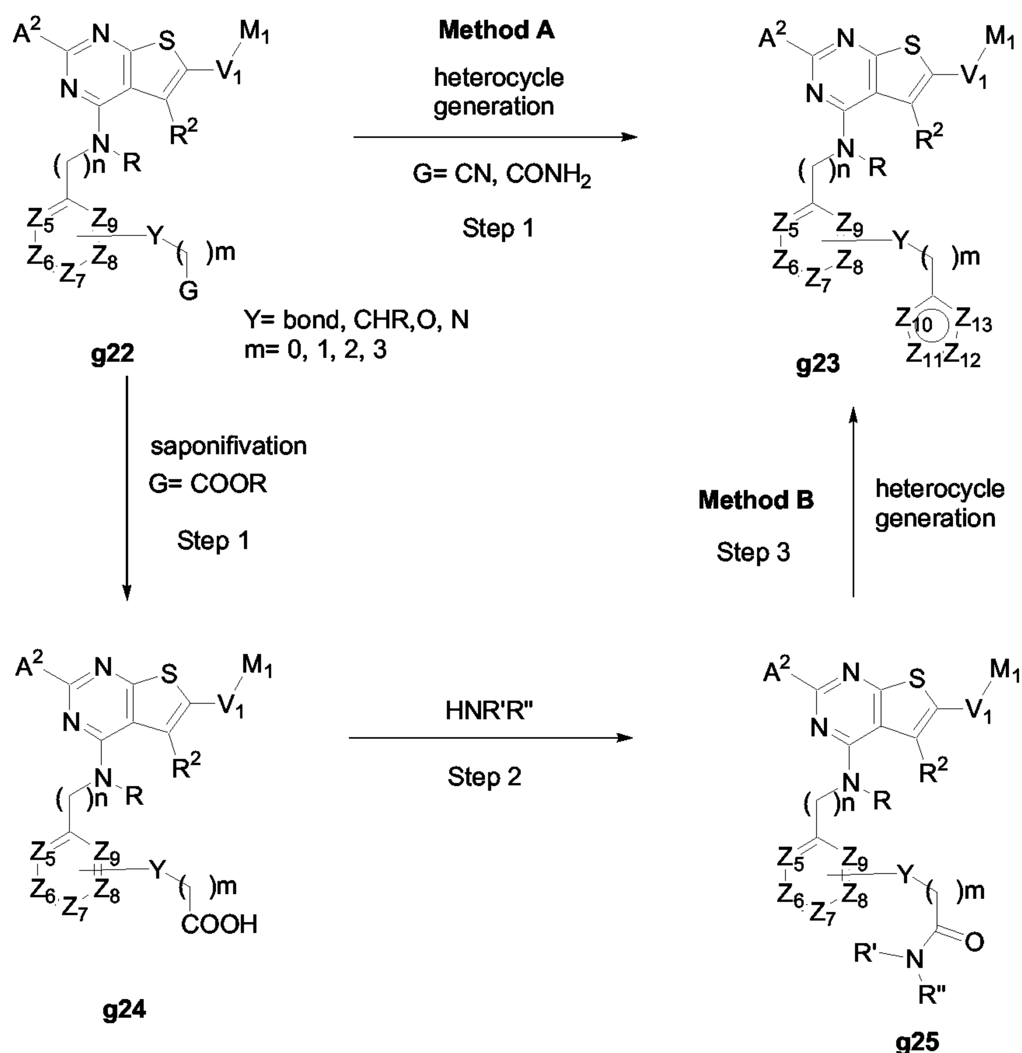
Scheme 11
