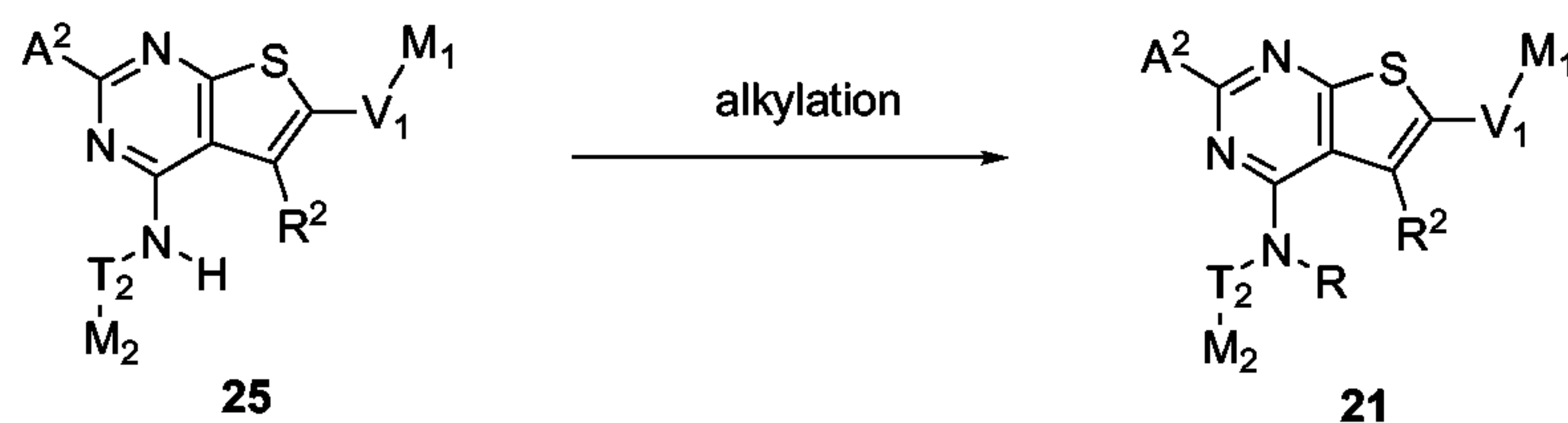
Scheme 14
