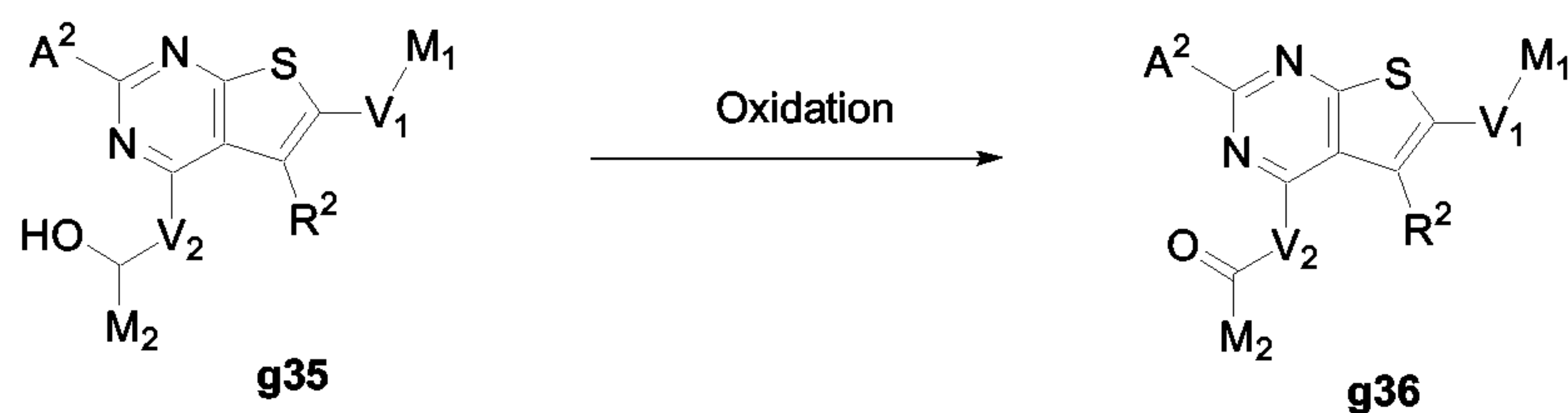
Scheme 16
