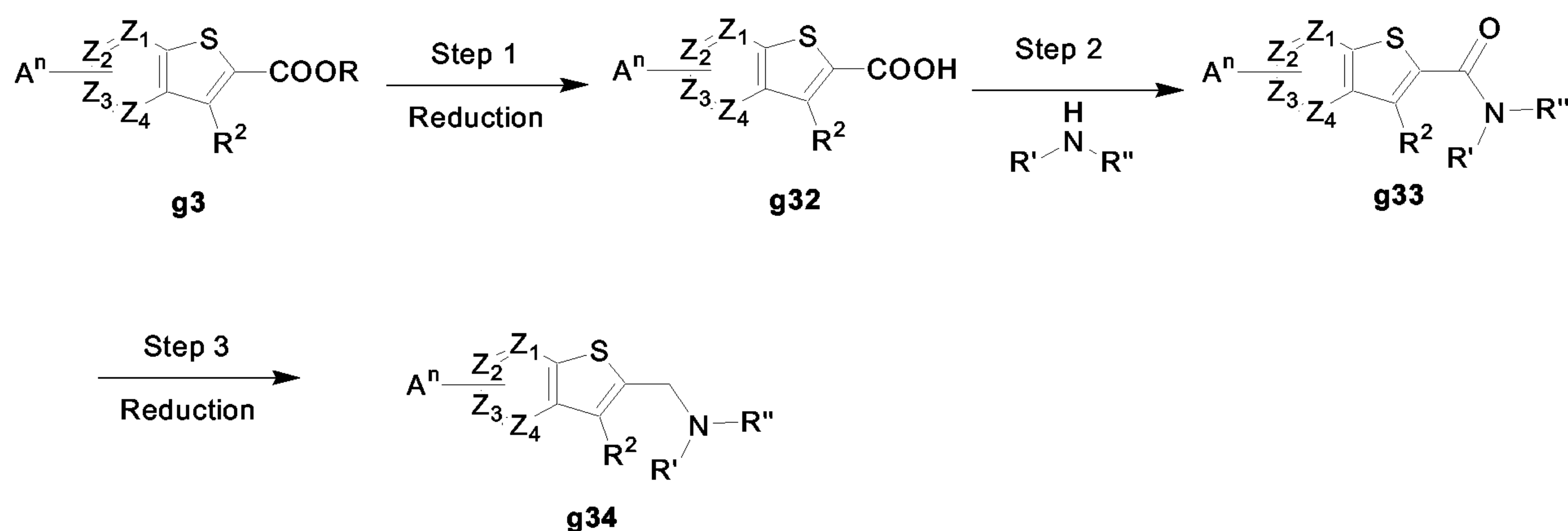
Scheme 15
