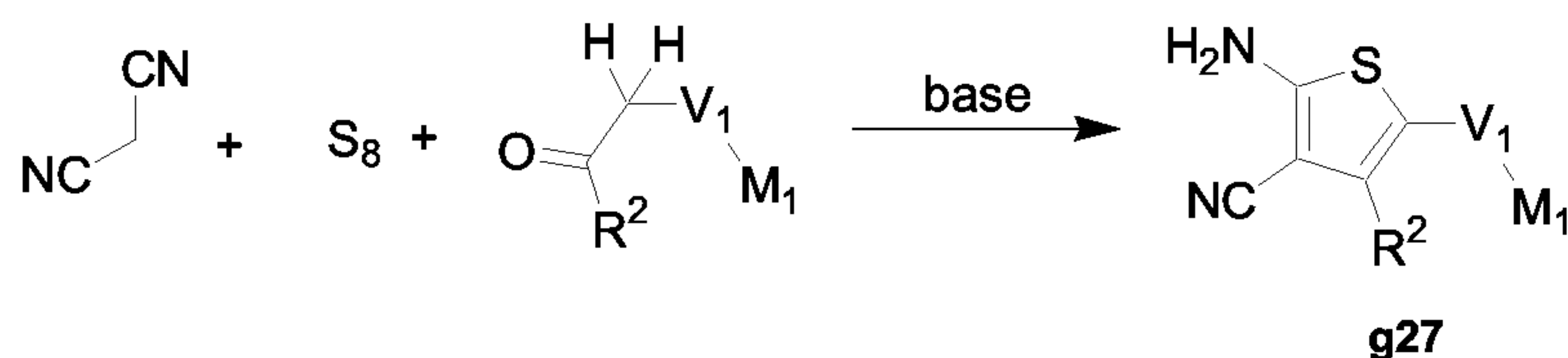
Scheme 8
