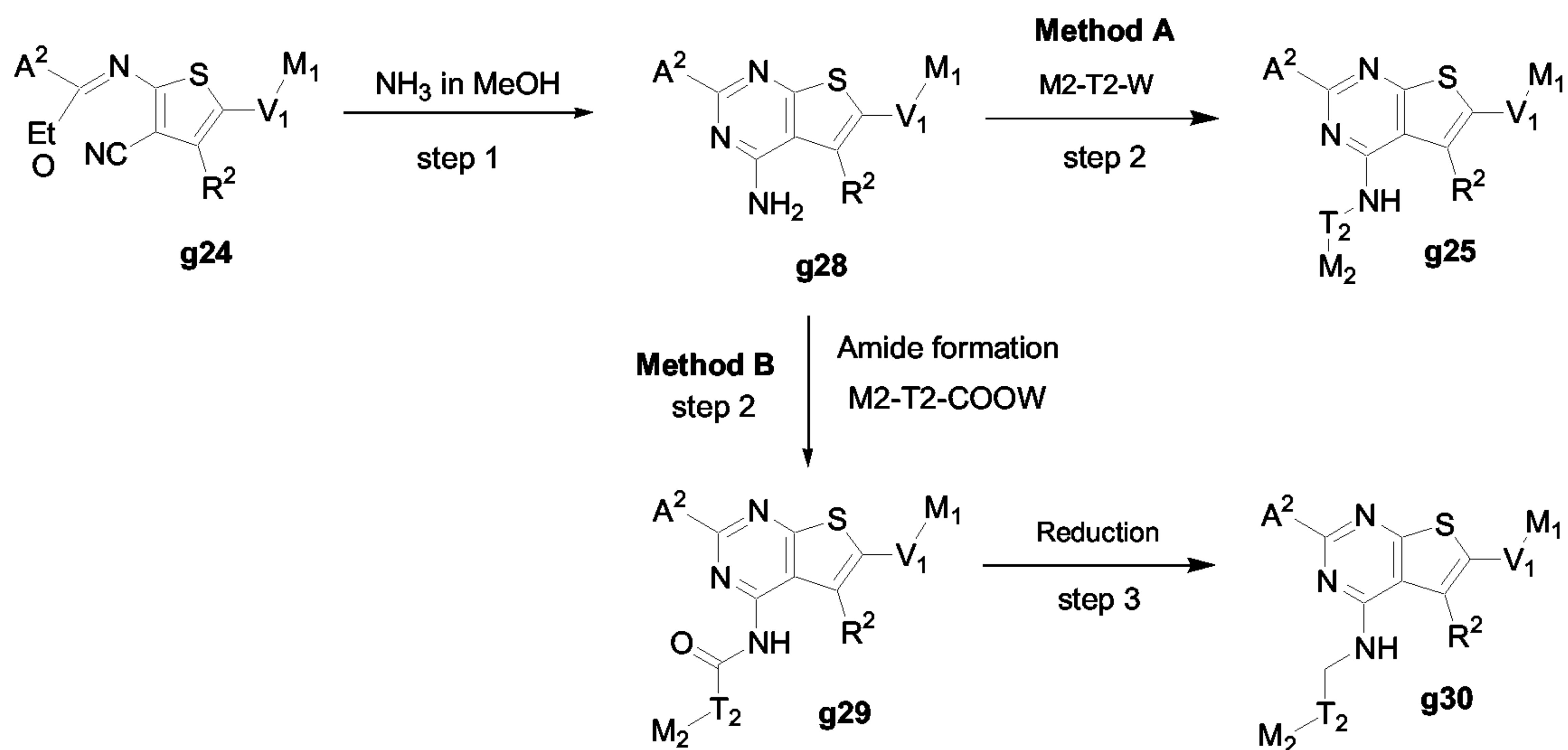
Scheme 9
