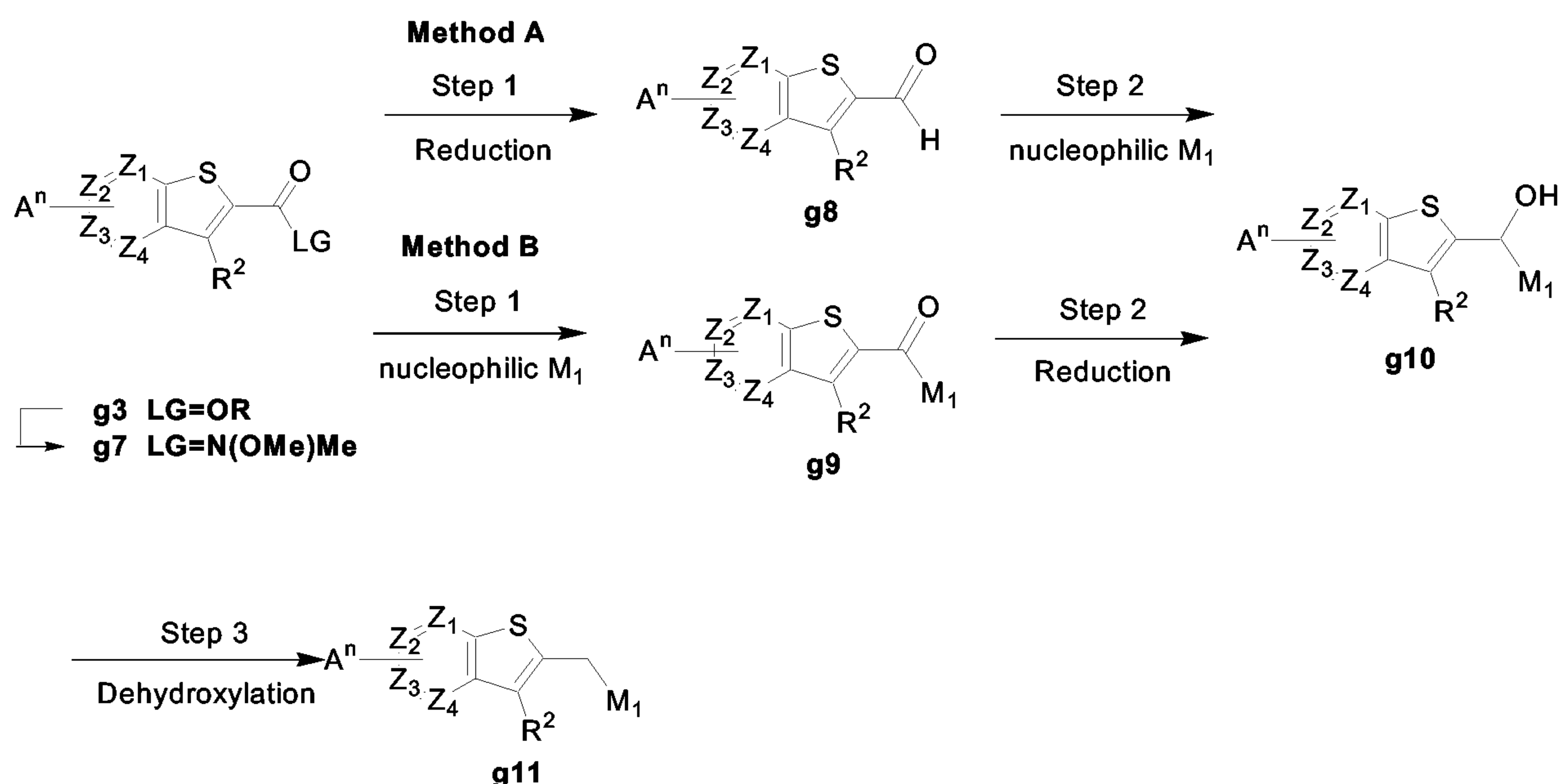
Scheme 3
