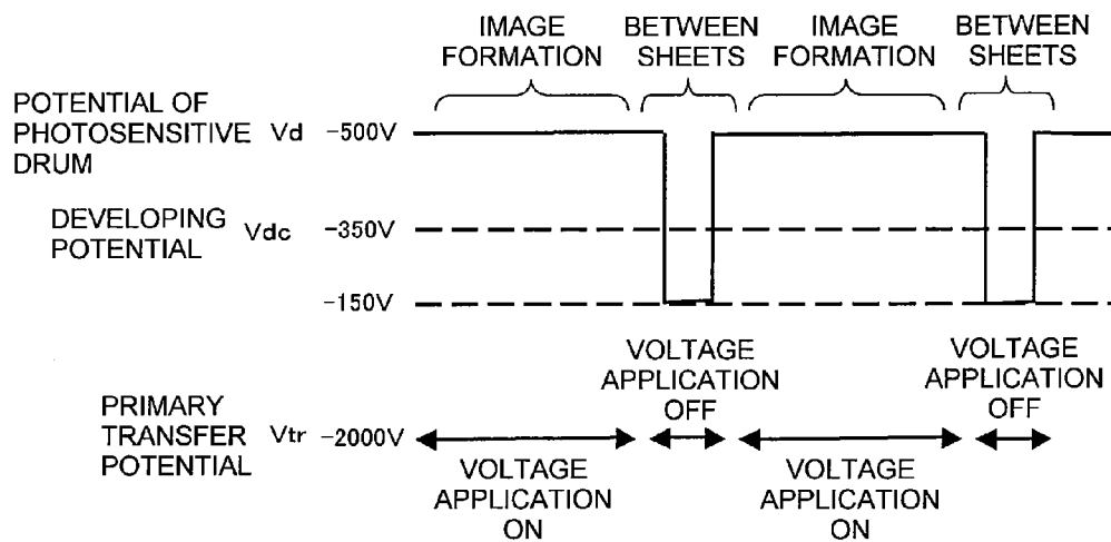
FIG. 5B WHEN OPERATION FOR REMOVING ABRASIVE PARTICLES IS SET BETWEEN SHEETS
