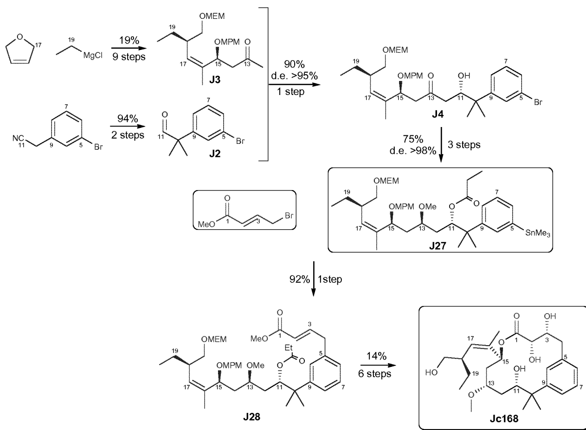
Scheme 1: New synthesis route for JC168
