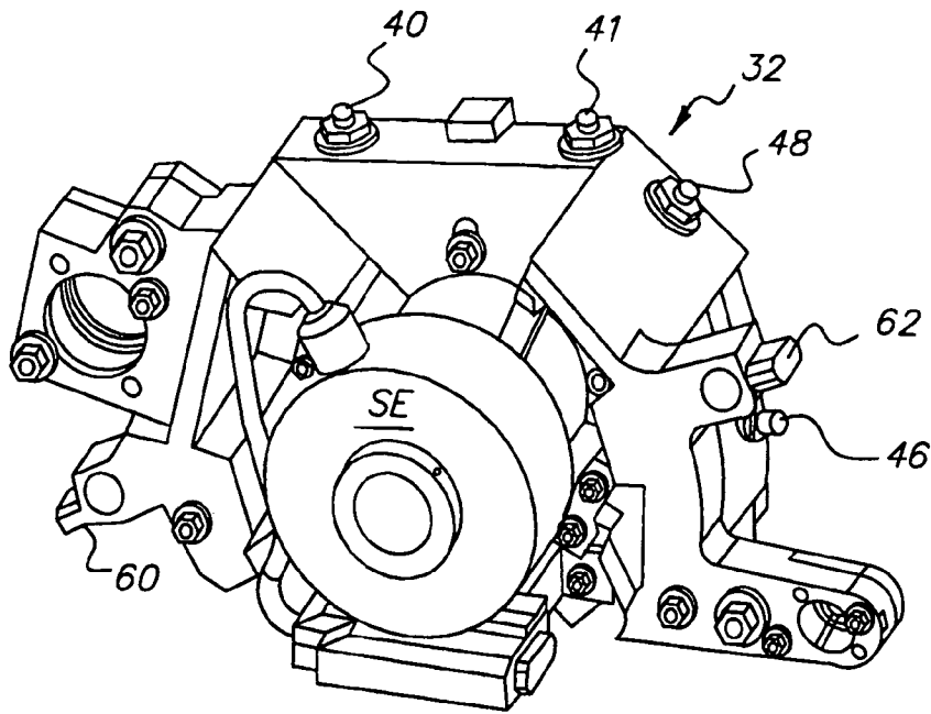
(PRIOR ART) FIG. 3A
