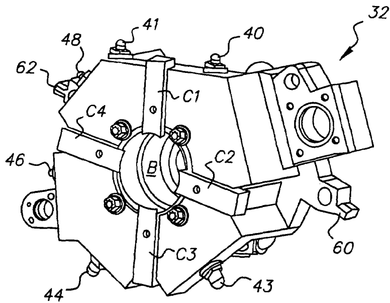
(PRIOR ART) FIG. 4A
