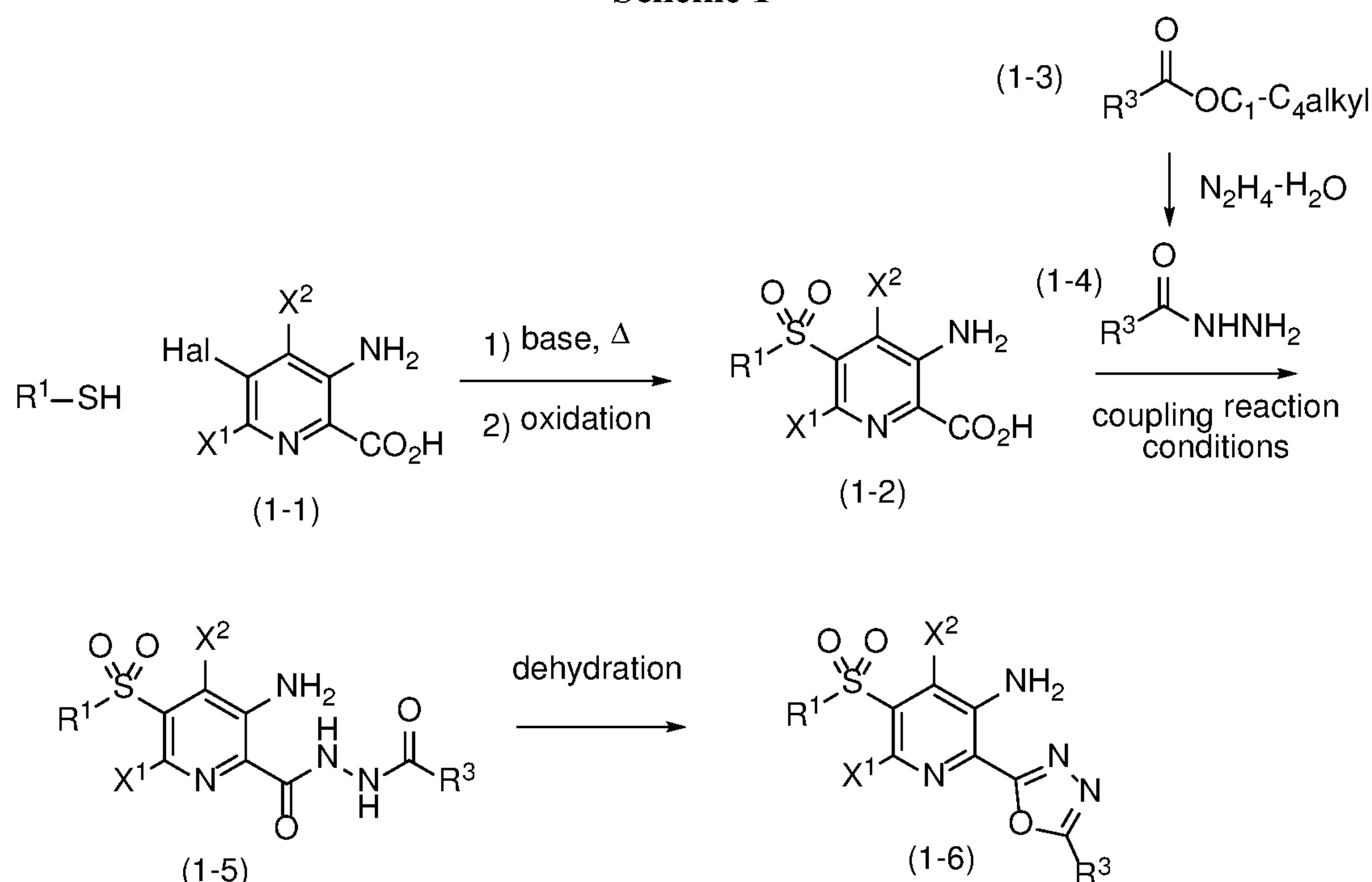
Scheme 1
