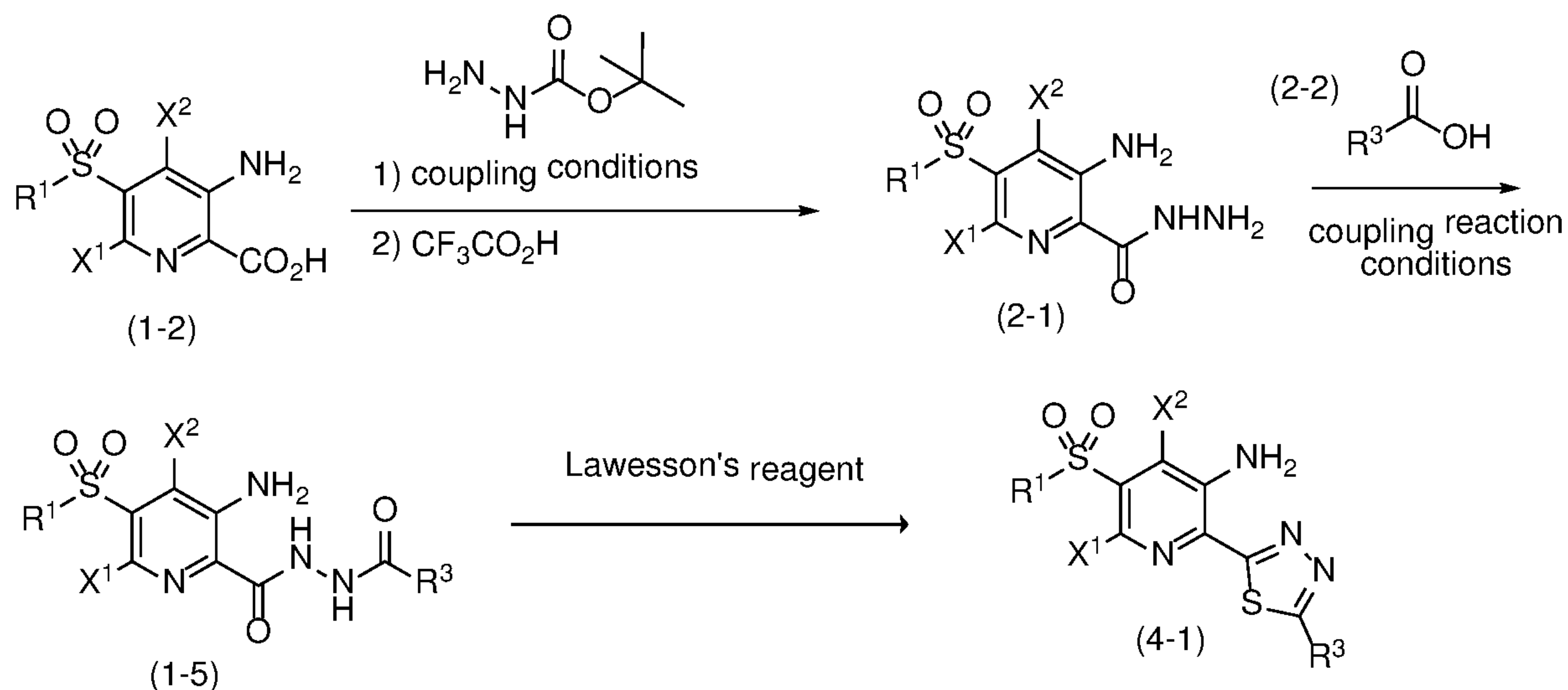
Scheme 4
