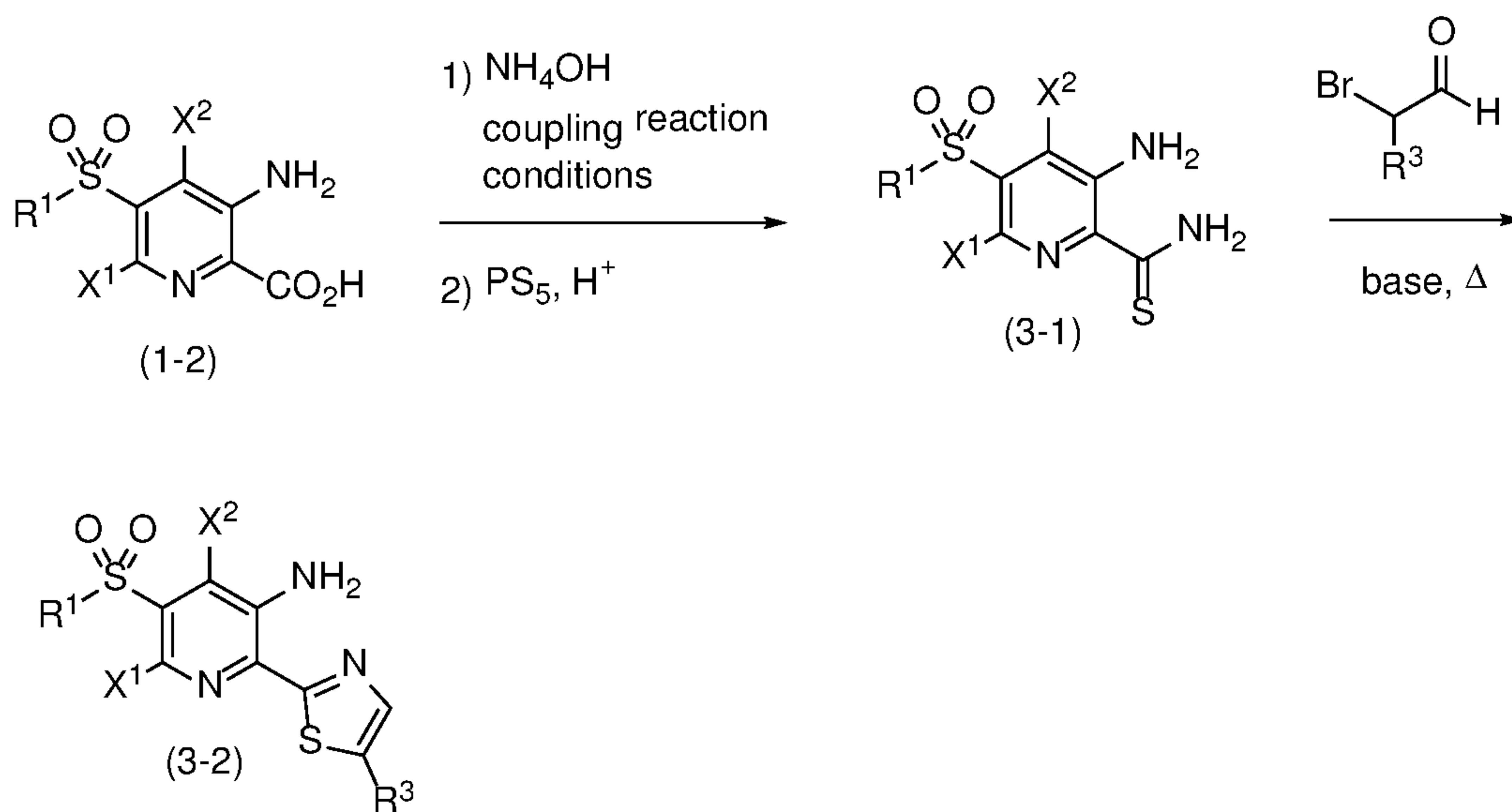
Scheme 3
