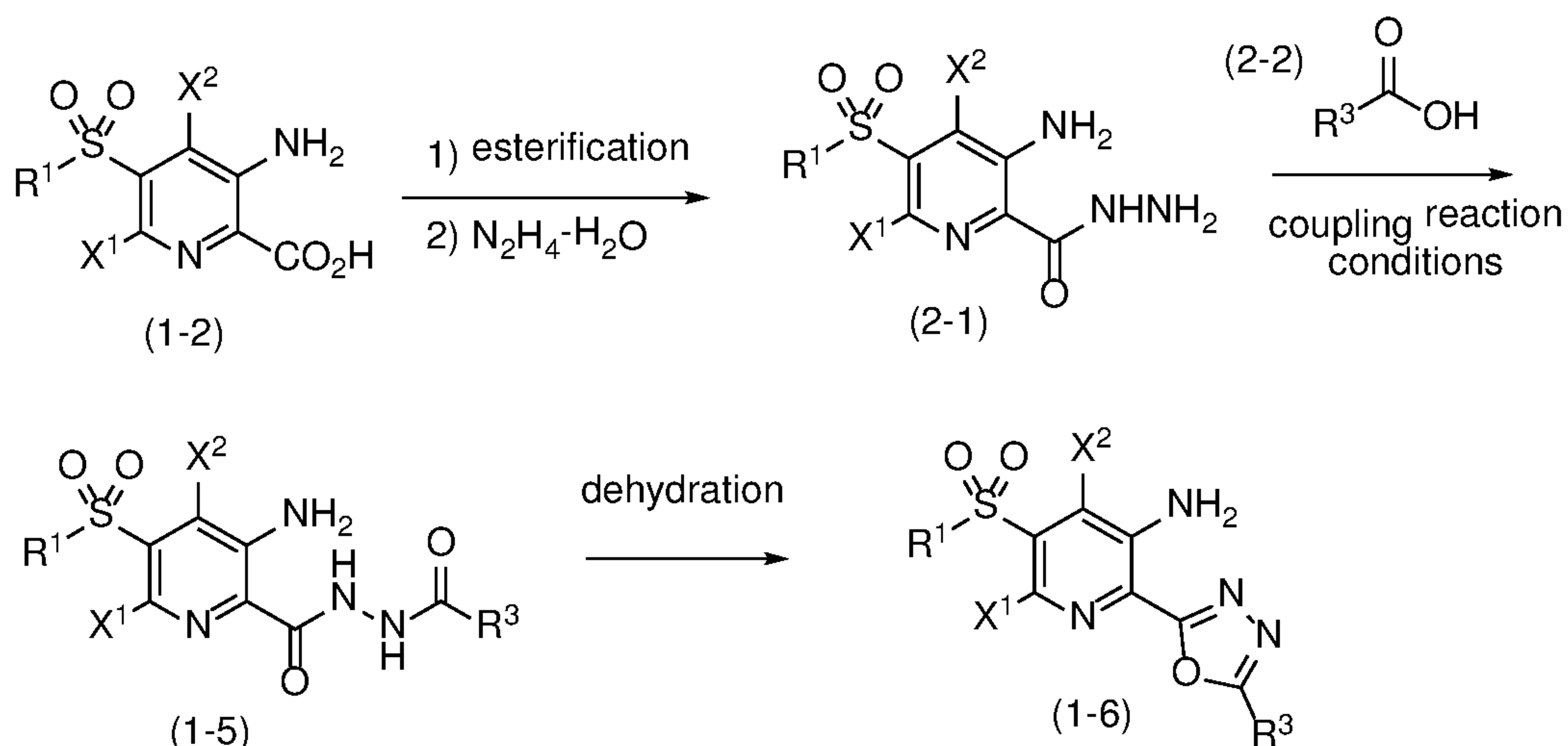
Scheme 2
