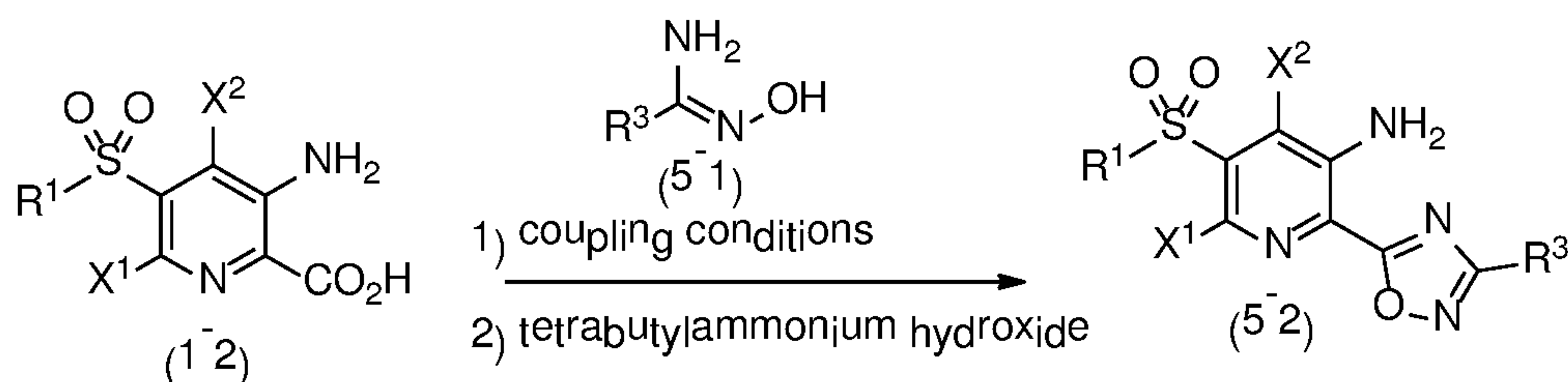
Scheme 5
