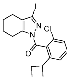
(2-chloro-6-cyclobutylphenyl)(3-iodo-4,5,6,7-tetrahydro-1H-indazol-1-yl)methanone
