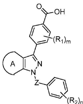
(I-1)
