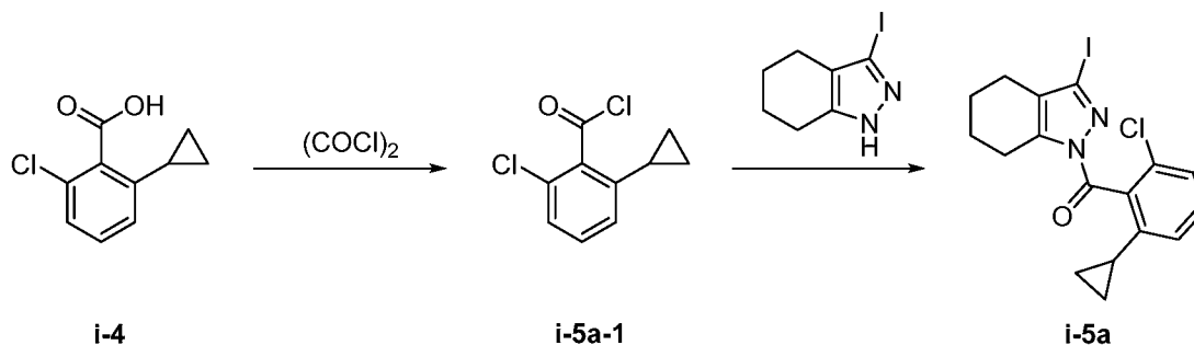
Intermediate i-5a
