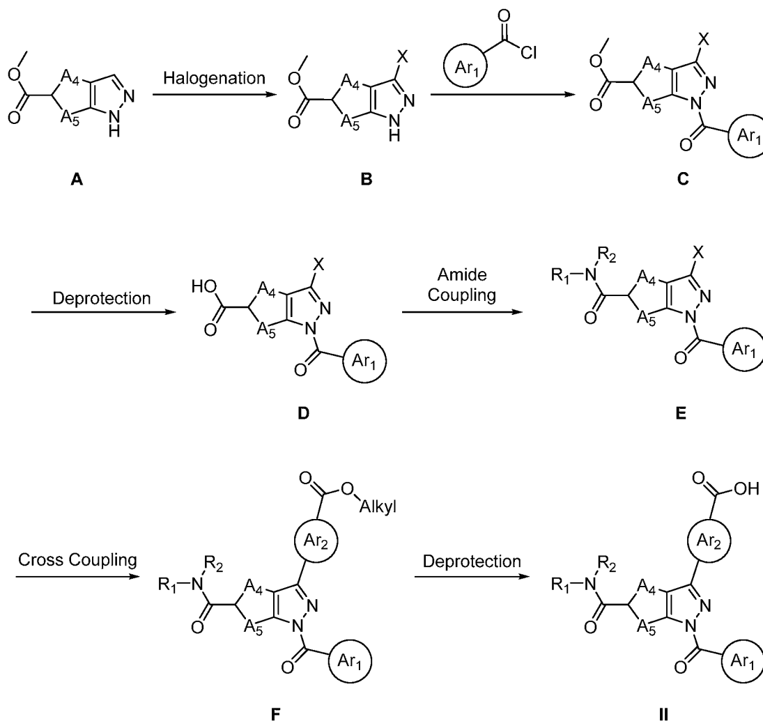
Scheme 2
