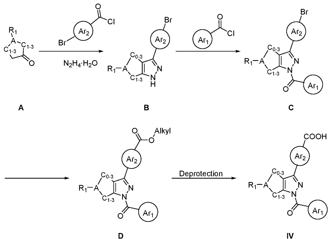
Scheme 4
