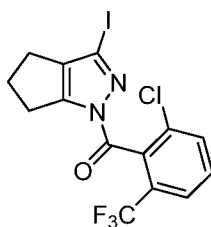
Intermediate i-2a
