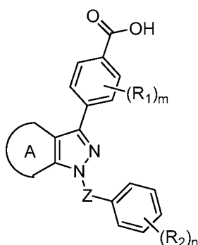
(I-2)
