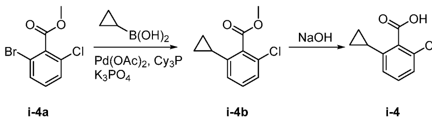
Intermediate i-4
