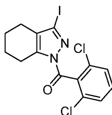
(2,6-dichlorophenyl)(3-iodo-4,5,6,7-tetrahydro-1H-indazol-1-yl)methanone
