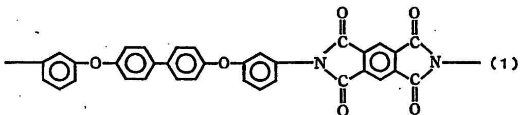
Chemical formula 1
