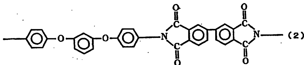
Chemical formula 2
