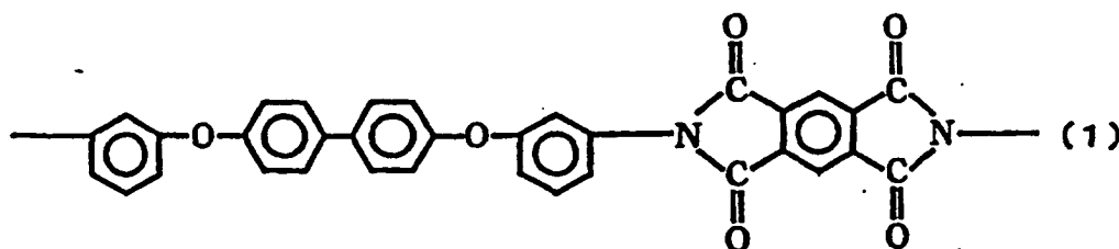
Chemical formula 2
