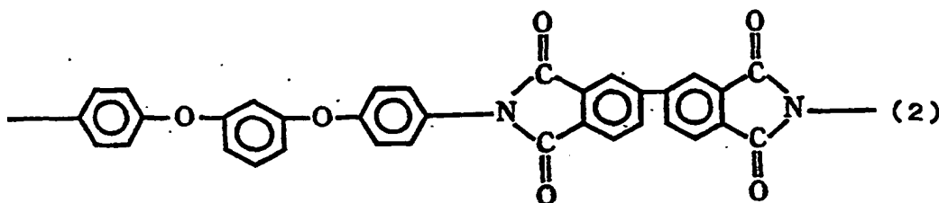
Chemical formula 2
