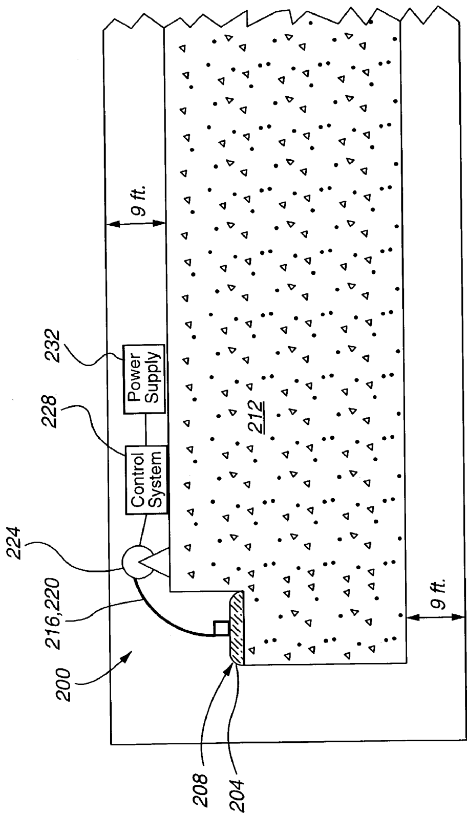
Fig. 2 SIDE VIEW
