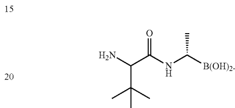
FIG. 19 is an NMR spectra for t-butylglycine-boroAla-nine,
