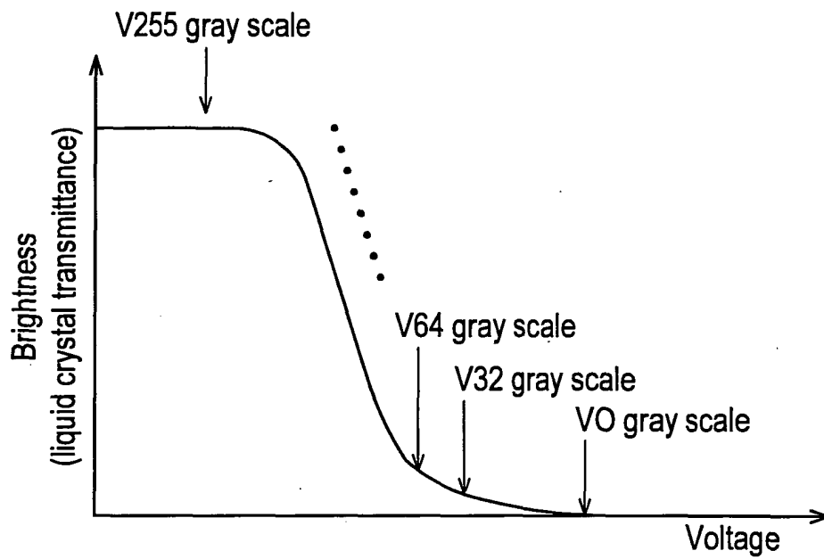
V-T characteristic voltage of a LCD panel
