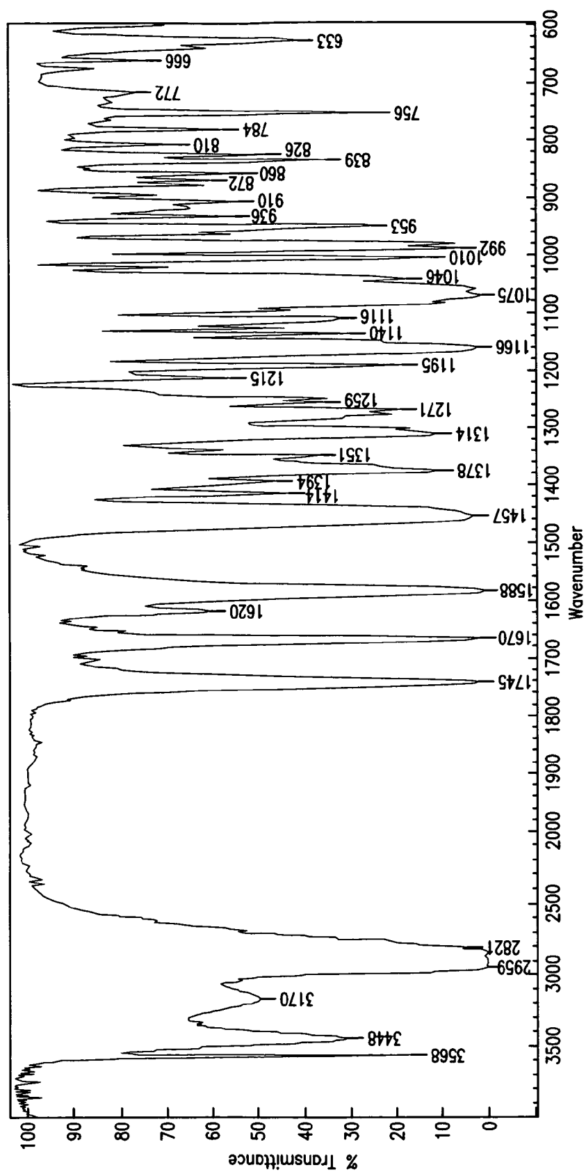
FIGURE 25/40 IR Spectrum for a Form IV Polymorph Sample in a Nujol Suspension
