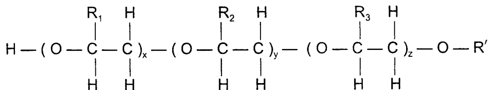
General Chemical Structure A
