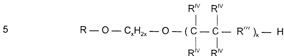
General Chemical Structure F
