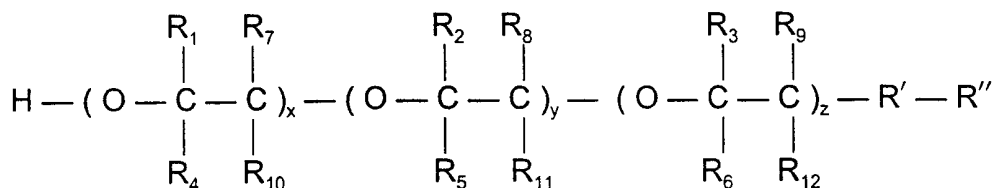
General Chemical Structure B
