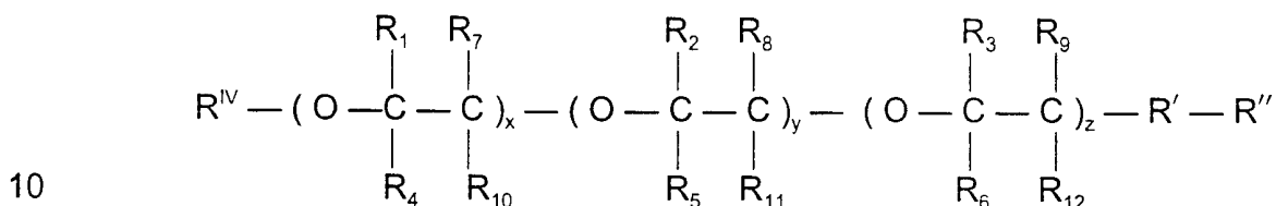
General Chemical Structure C
