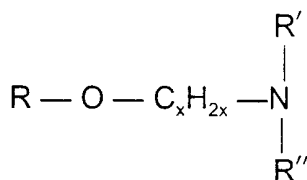
General Chemical Structure E
