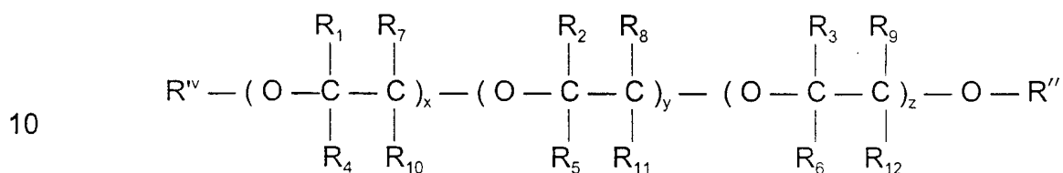
General Chemical Structure D
