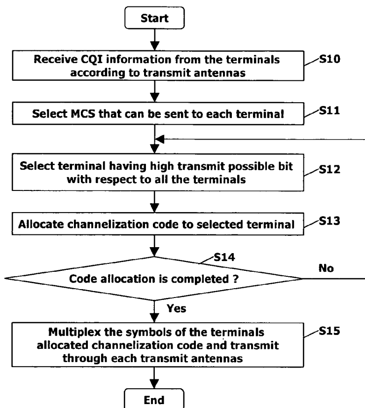
FIG.4 Related Art
