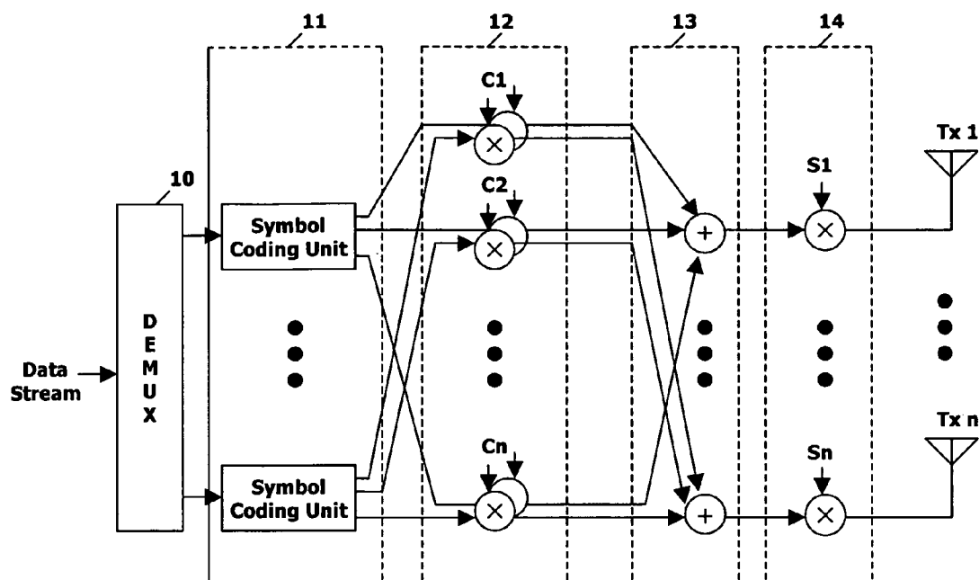
FIG.1 Related Art
