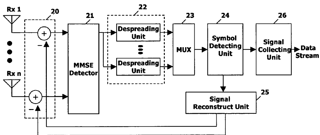
FIG.2 Related Art
