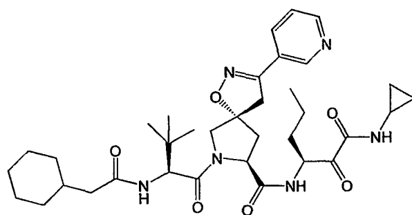
Compound No. 303
