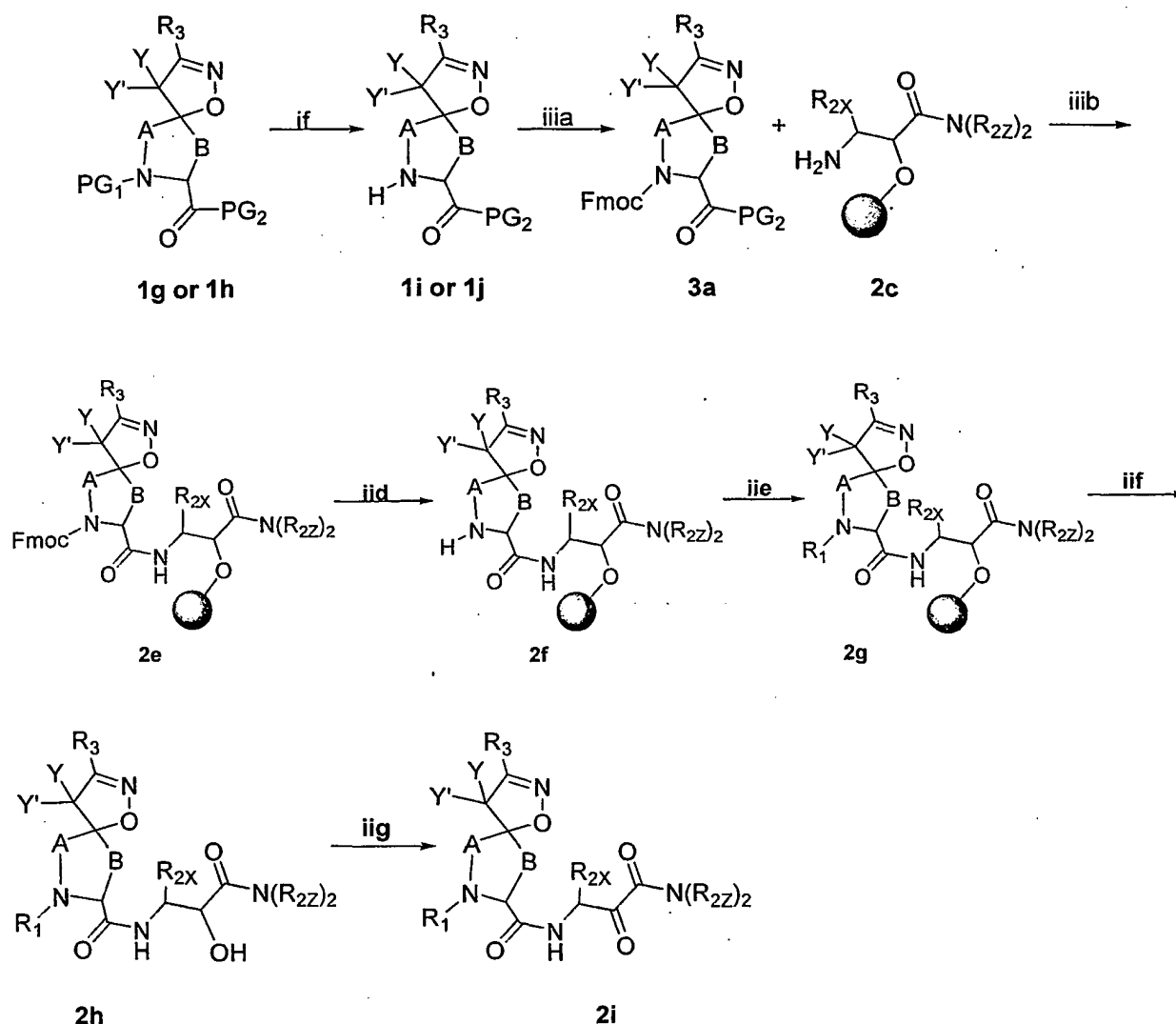
Scheme 3
