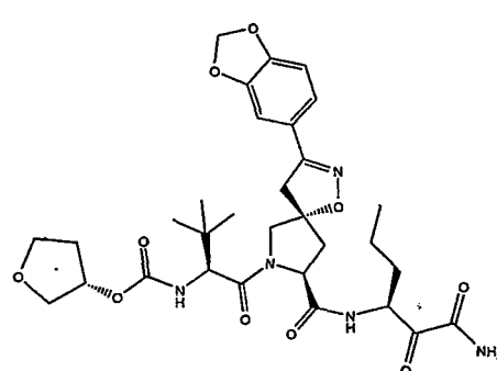
Compound No. 422
