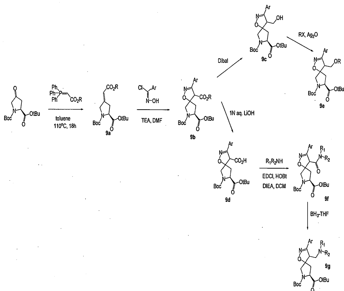
Scheme 9:
