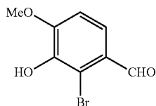
2-Bromo-3-Hydroxy-4-Methoxy-Benzaldehyde (8)
