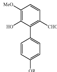
(R = TIPS, 96%)
