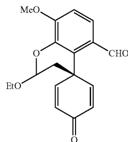
Cross-Conjugated Cyclohexadienone (14)
