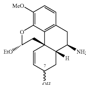
12-Amino-6-Ethoxy-8-Methoxy-1,5,6,11,12,12a-Hexahydro-2H-Naphtho[8a,1,2-de]Chromen-2-Ol (17/17a)
