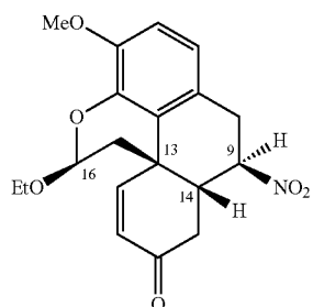
6-Ethoxy-8-Methoxy-12-Nitro-1,5,6,11,12,12a-Hexahydro-Naphtho[8a,1,2-de]Chromen-2-One (16)
