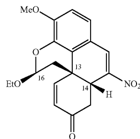
6-Ethoxy-8-Methoxy-12-Nitro-1,5,6,12a-Tetrahydro-Naphtho[8a,1,2-de]Chromen-2-One (15)
