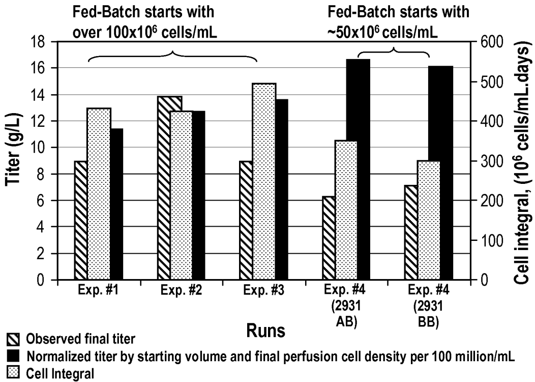
Summary of Productivity as a Function of Cell Integral
