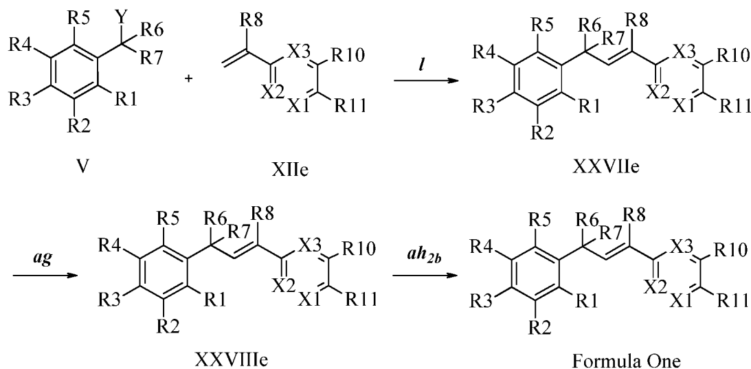
Scheme XXIV
