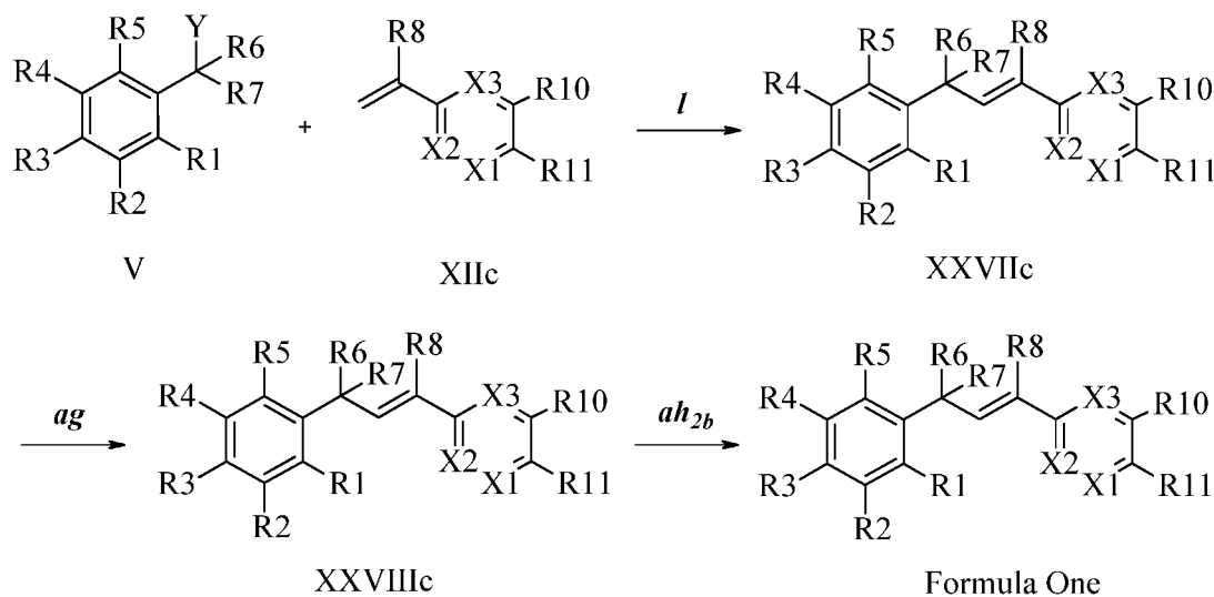
Scheme XXII
