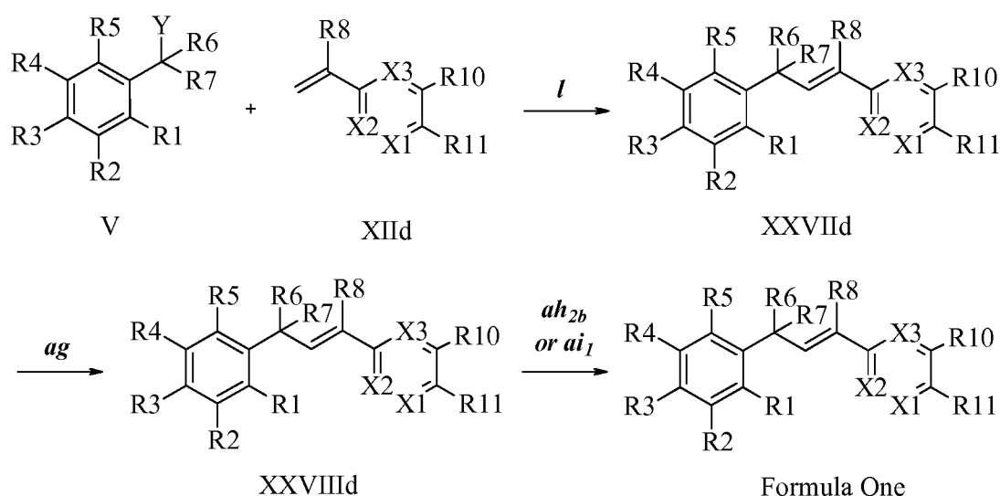
Scheme XXIII
