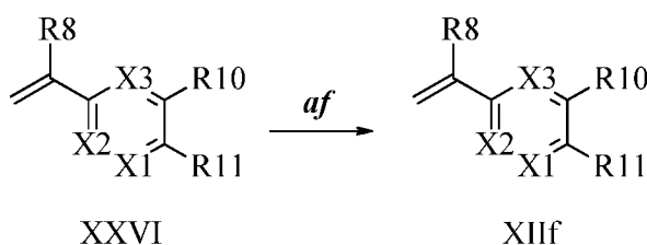
Scheme XIX
