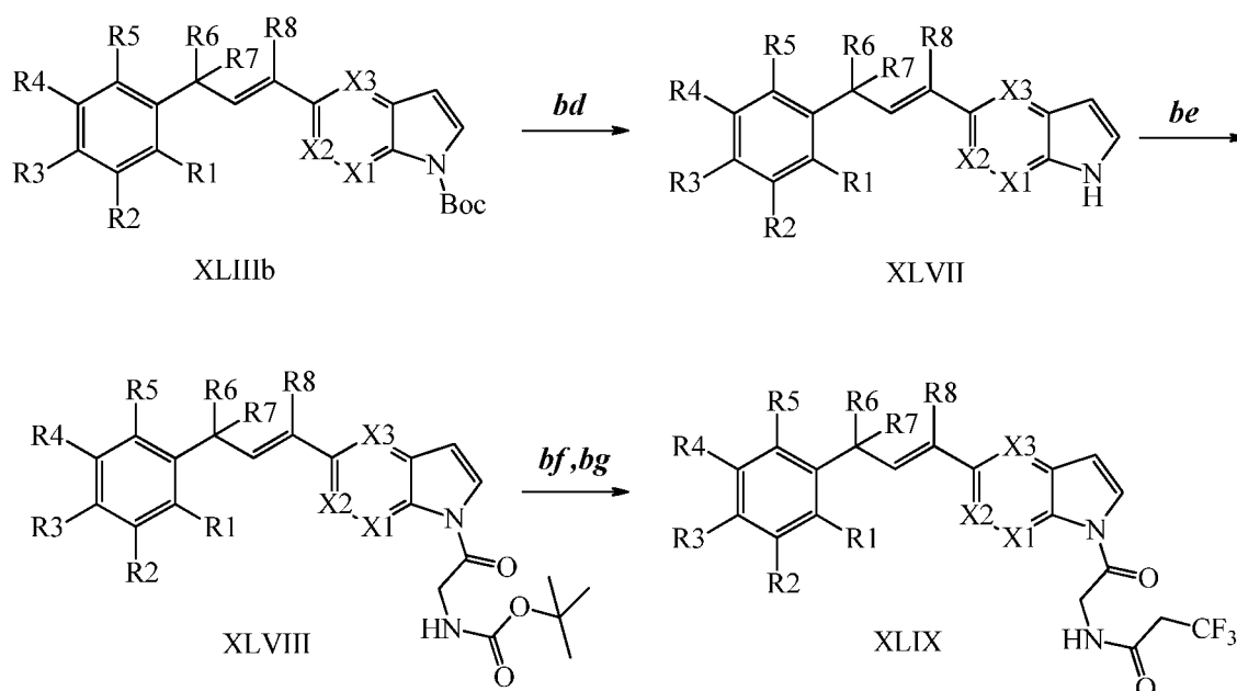
Scheme XXXVII
