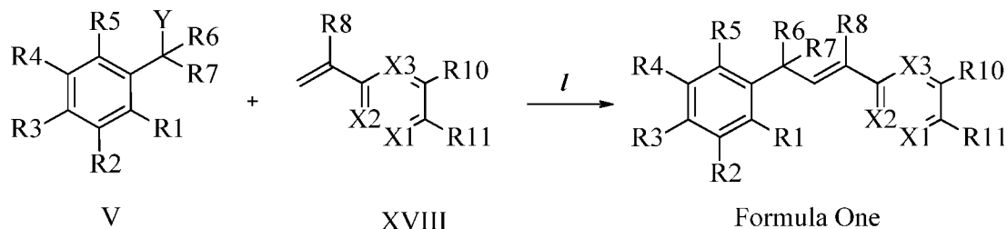
Scheme XXVI
