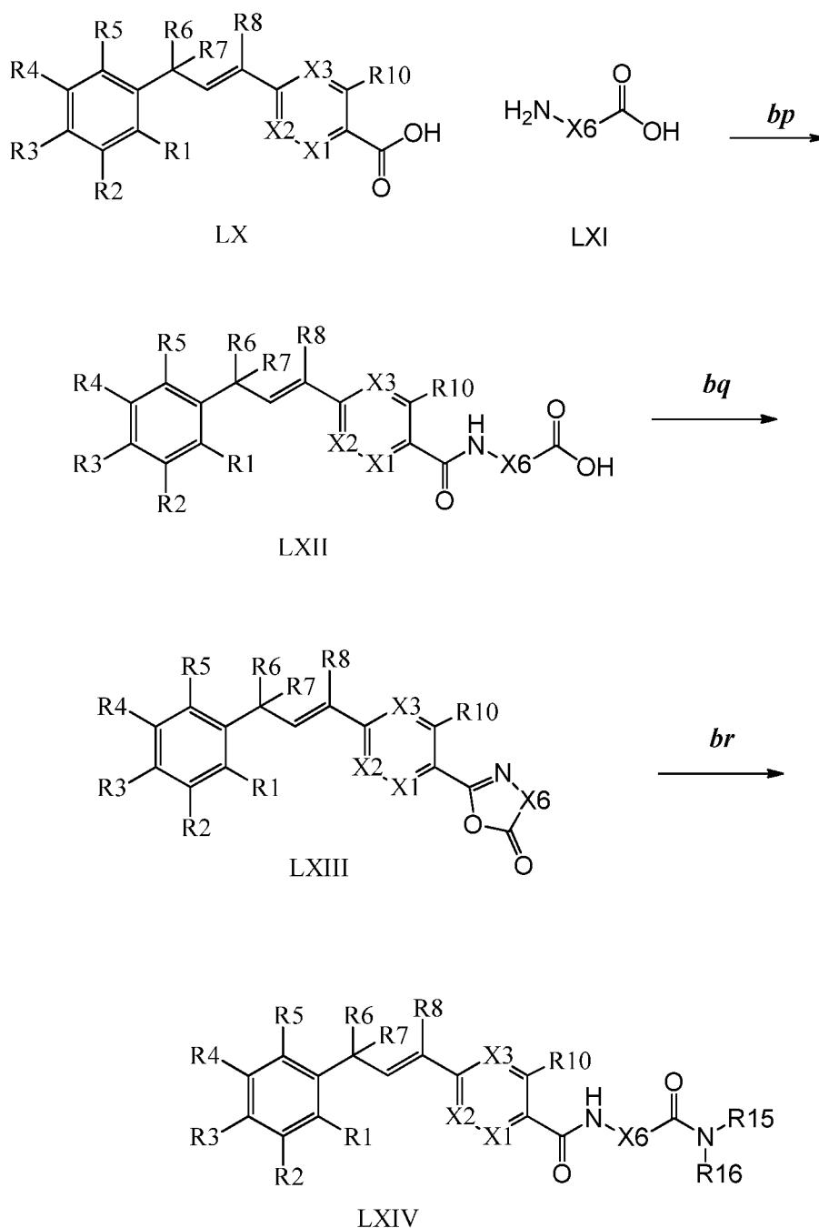
Scheme XLI
