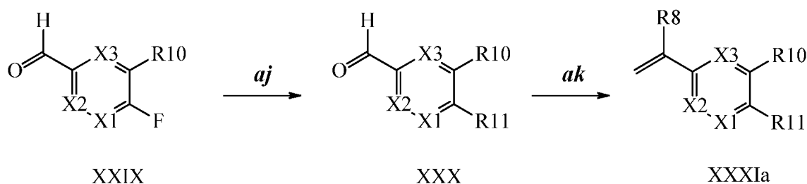
Scheme XXVII
