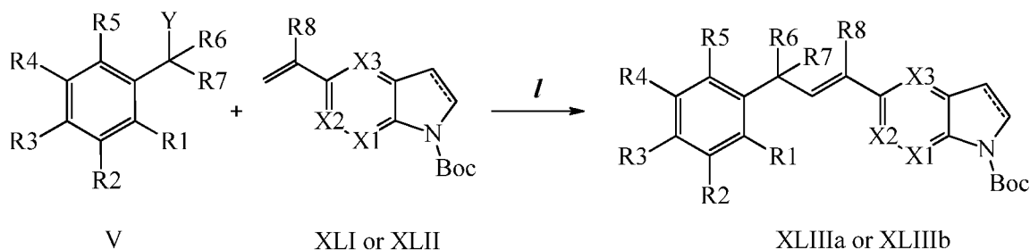
Scheme XXXV
