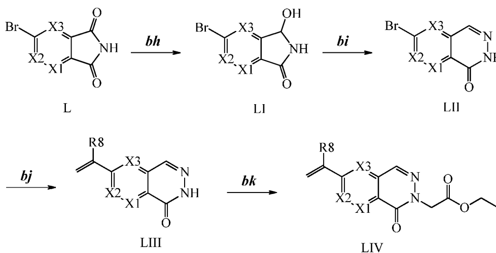
Scheme XXXVIII
