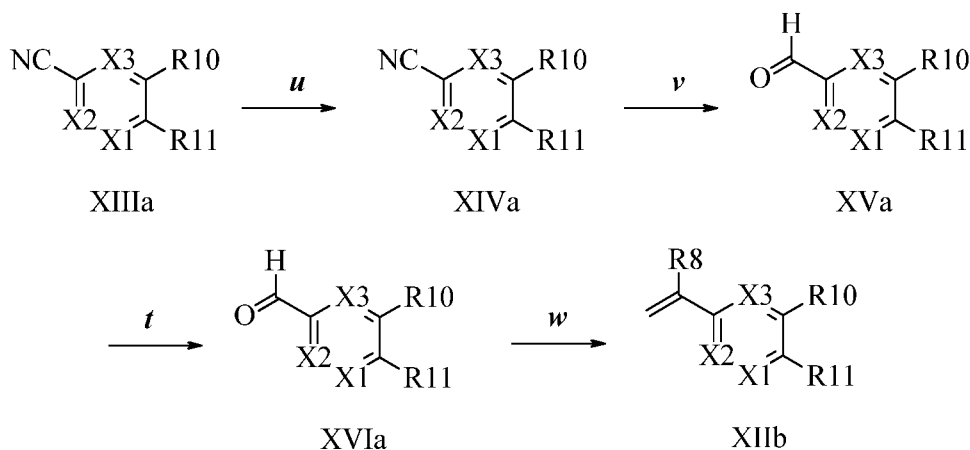
Scheme XIV
