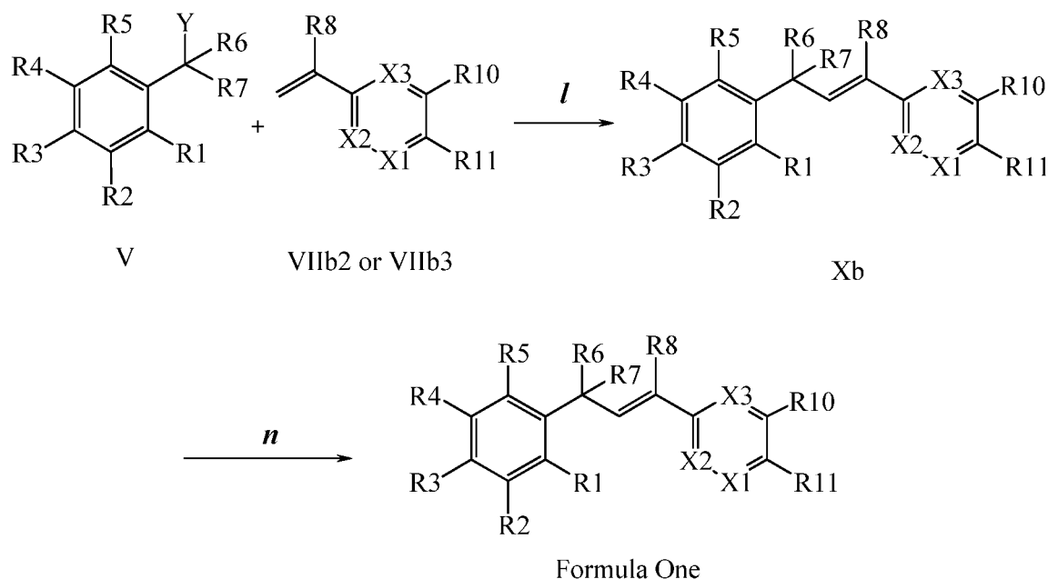
Scheme VIII
