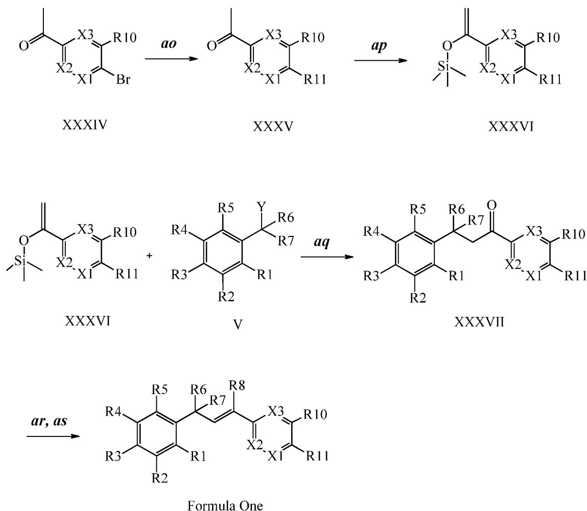
Scheme XXXI
