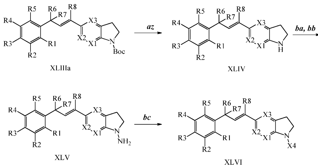
Scheme XXXVI
