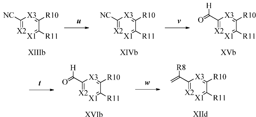
Scheme XVII
