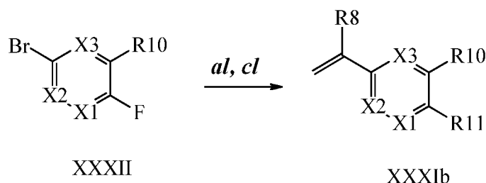
Scheme XXVIII
