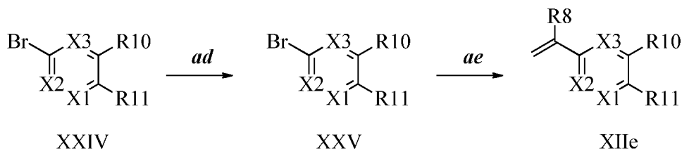
Scheme XVIII
