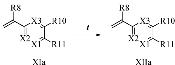
Scheme XIII
