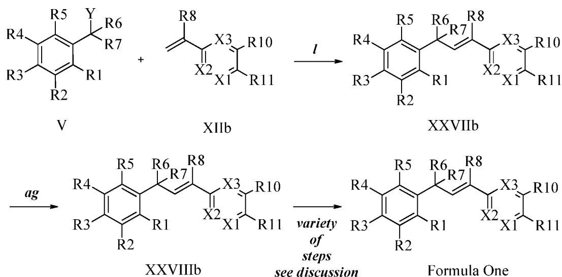
Scheme XXI
