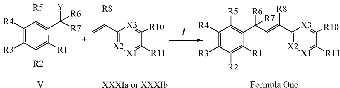
Scheme XXIX
