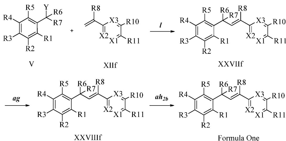
Scheme XXV
