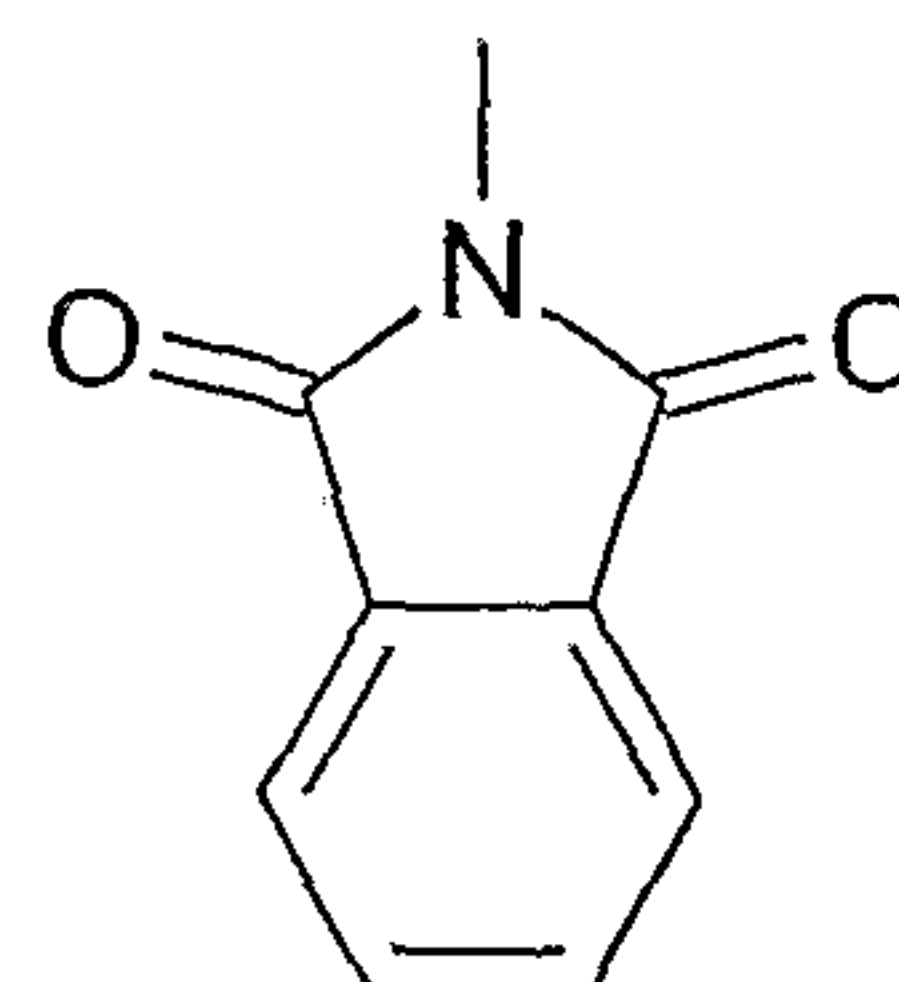
phthalimidyl
