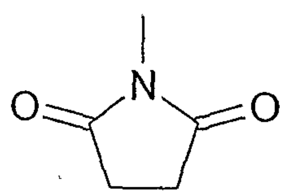
succinimidyl
