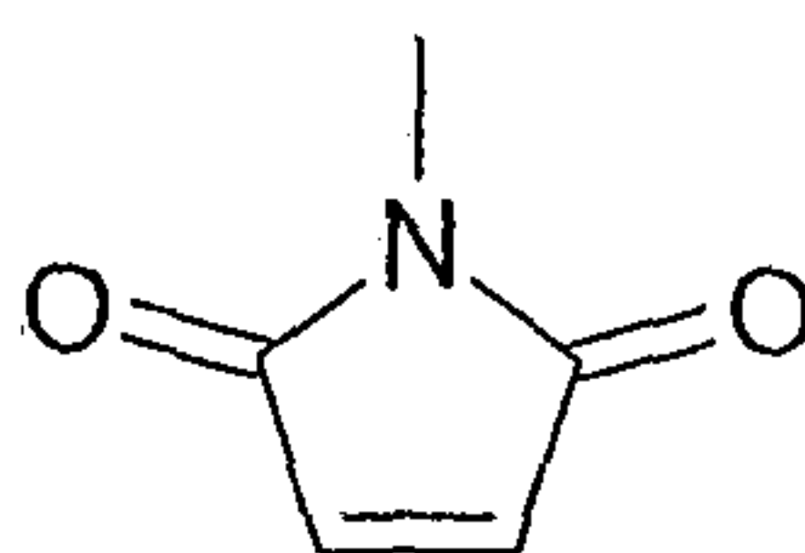
maleimidyl
