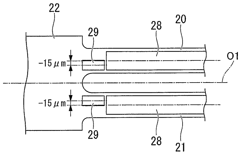
FIG.21C
