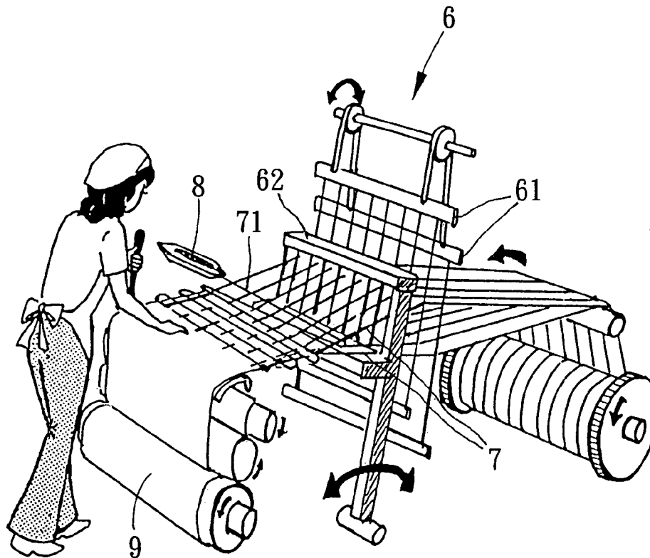
PRIOR ART Fig. 14
