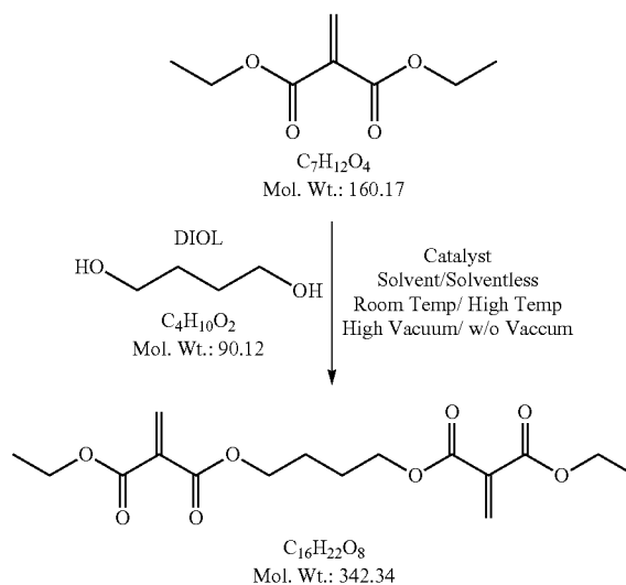
SCHEME 2A: Formation of MMM by Transesterification with diol
