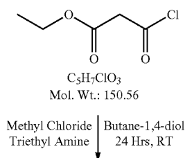
SCHEME 2: Transesterification
