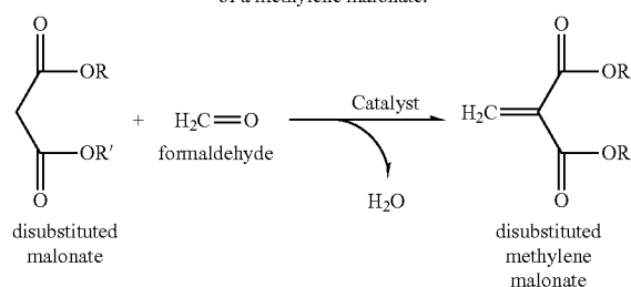
SCHEME 1: Modified Knoevenagel Reaction
