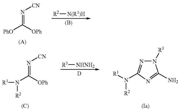
REACTION SCHEME 1
