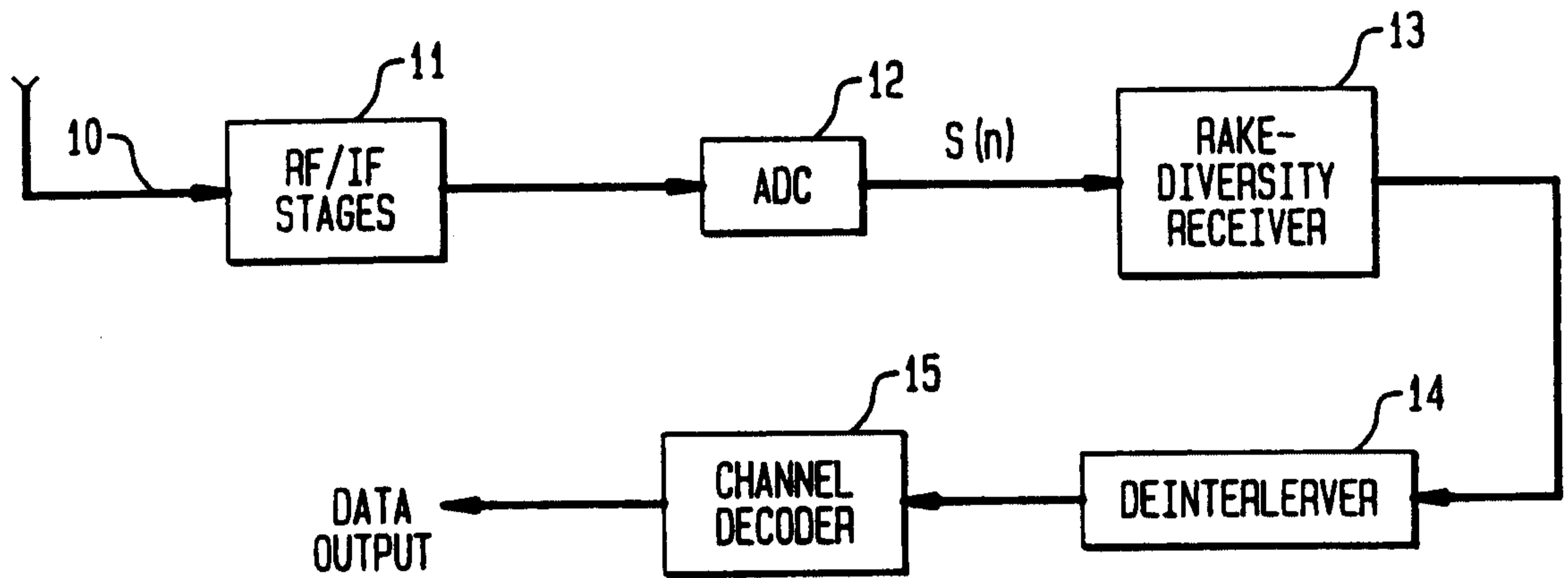
FIG. 1 (PRIOR ART)
