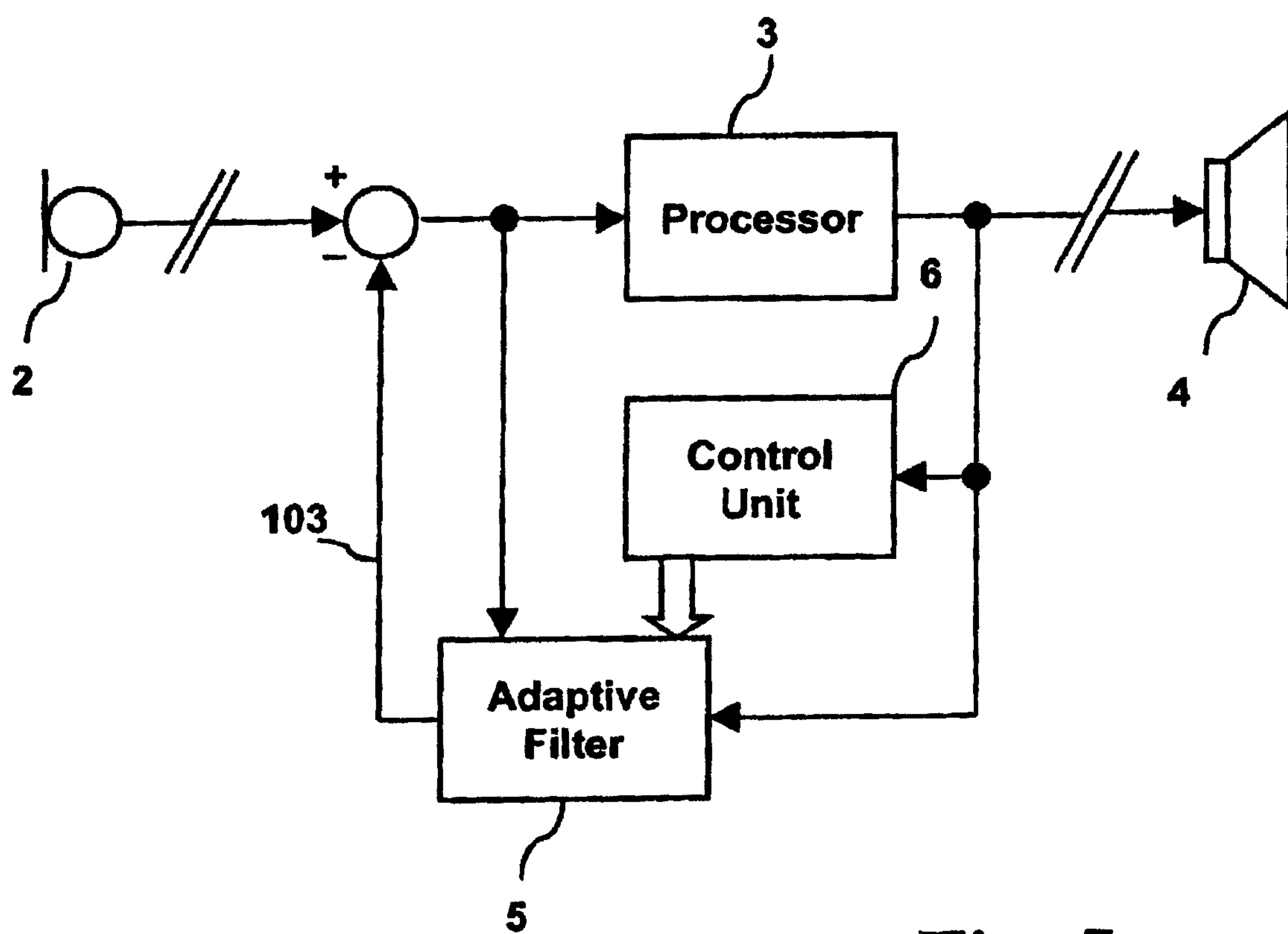
Fig. 5 (Prior Art)
