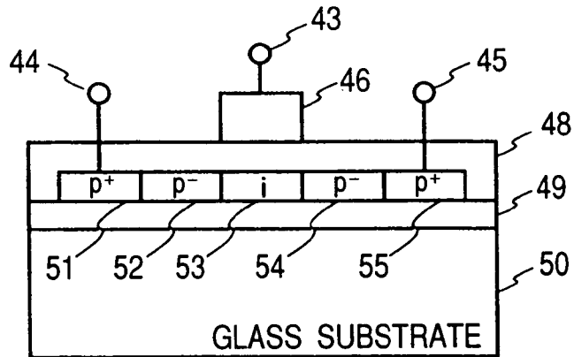
FIG. 5(a) STRUCTURE OF RESET TFT SWITCH 41
