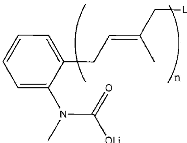
[Formula 1a]
