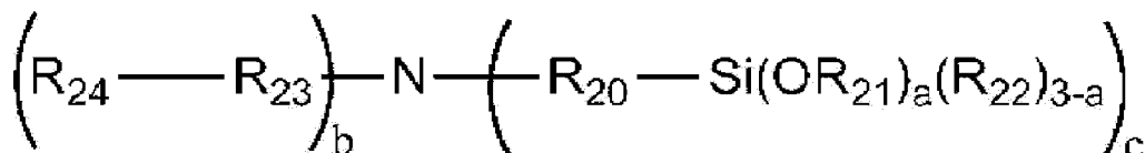
[Formula 2]
