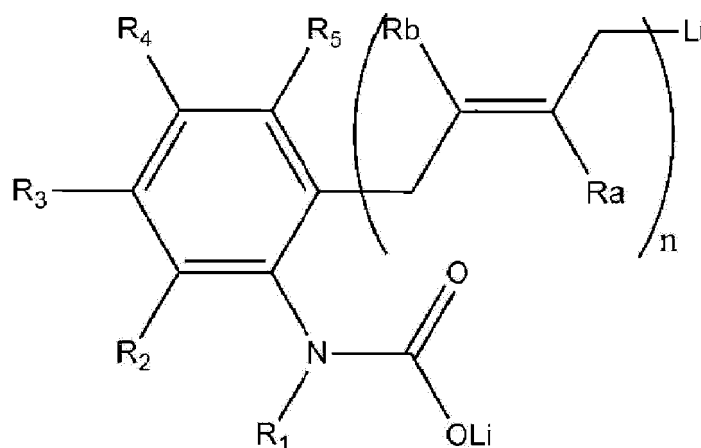
[Formula 2]
