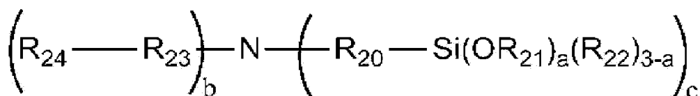
[Formula 2]
