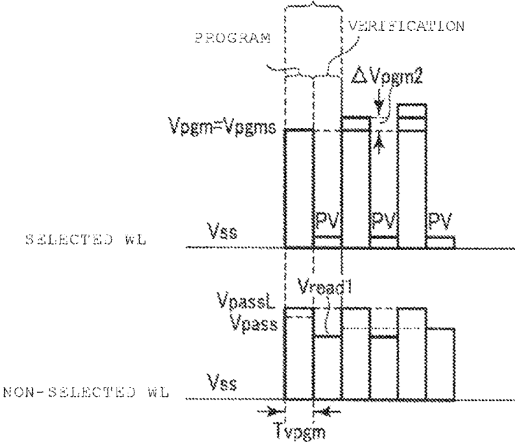
PROGRAM LOOP
