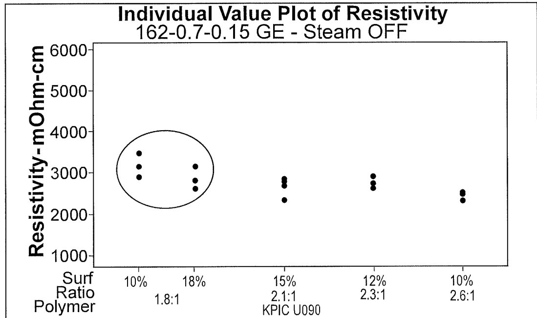
Fig. 9. Slightly higher electrical resistivity was observed at \text{SiO}_2/\text{PE} = 1.8 , and surfactant amount impacted average ER
