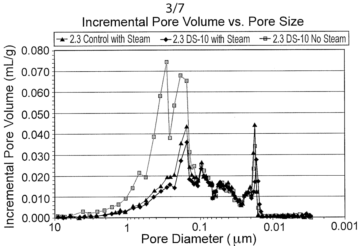
Fig. 3. Separator porosity and pore size distributions as determined with Hg porosimetry
