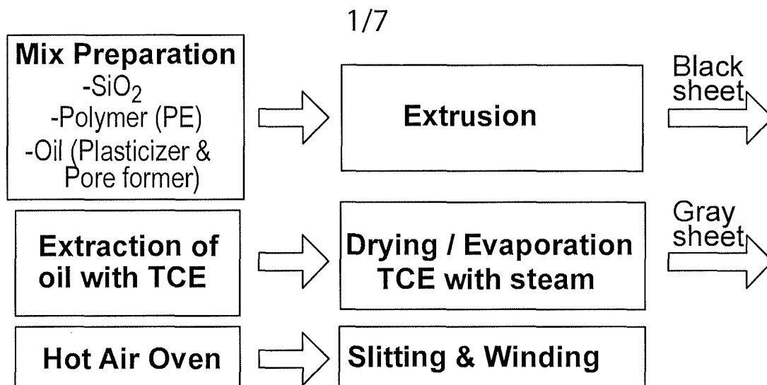
Fig. 1. Representative process flow diagram for separator manufacturing
