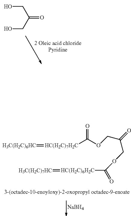
Reaction Scheme 9: Synthesis of 1,3-dioleoyl-2-glycerol ester
