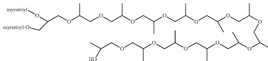
Chemical Structure 20: 1,2-dimyristoyl-rac-3-dodecapropylene glycol (mPPG-12)-glycerol
