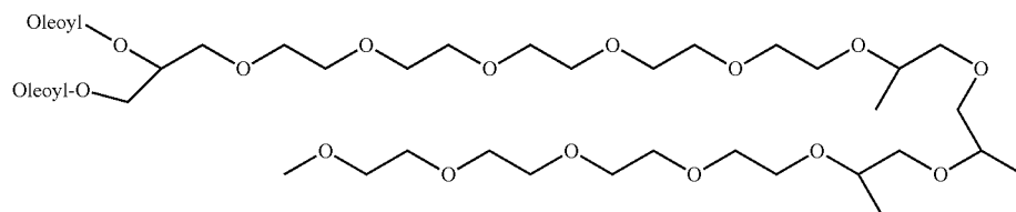
Chemical Structure 21: 1,2-dioleoyl-rac-3-monometoxyl tetraethylene glycol-tripropylene glycol-tetraethylene glycol glycerol ether
