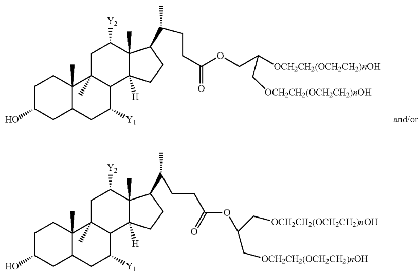
Chemical Structure 8
