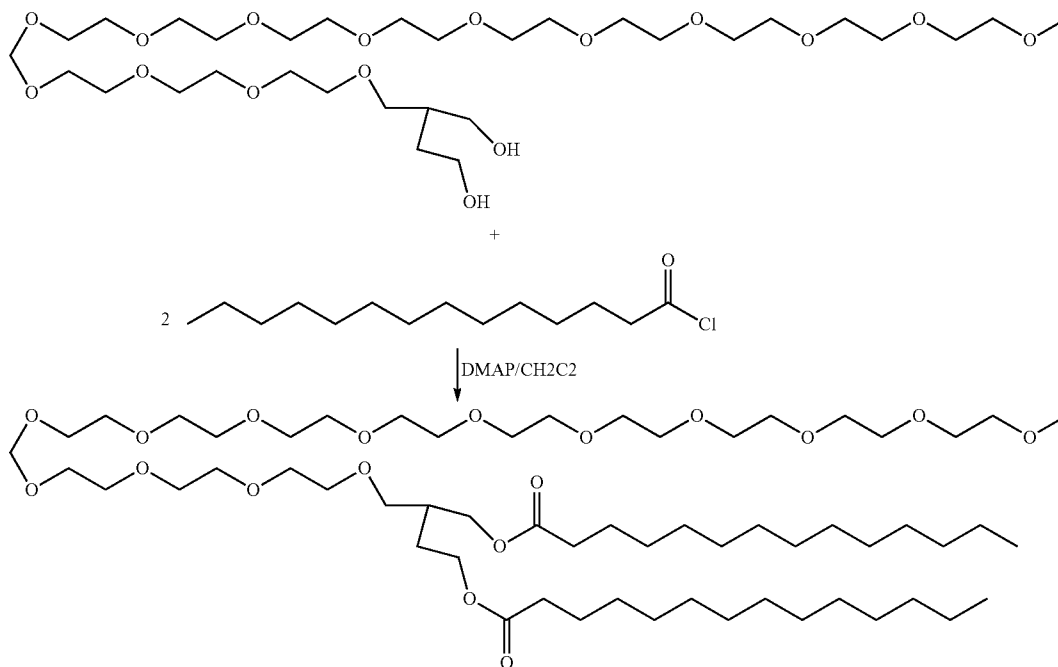
Reaction Scheme 2: Synthesis of 1,2-dimyristoyl-rac-3-PEG 12-glycerol
