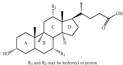
Chemical Structure 5
