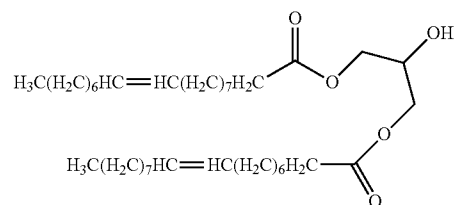
2-hydroxy-3-(octadec-10-enoyloxy)propyl octadec-9-enoate
