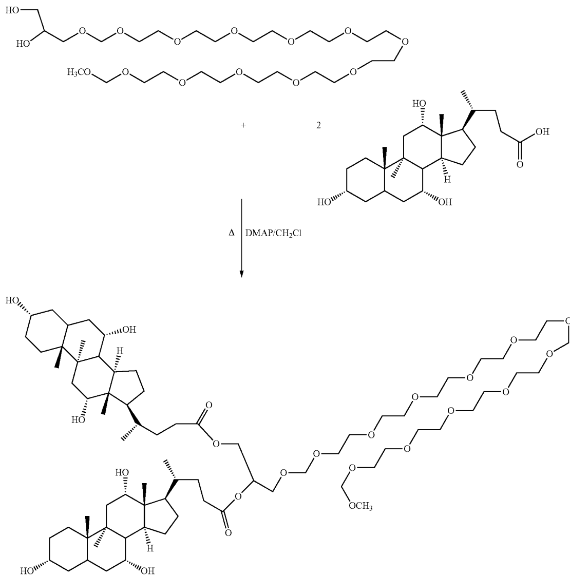
Reaction Scheme 4: Synthesis of 1, 2-dicholoyl-rac-3-mPEG 12-glycerol
