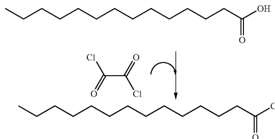
Reaction Scheme 3: Formation of Myristoyl Chloride
