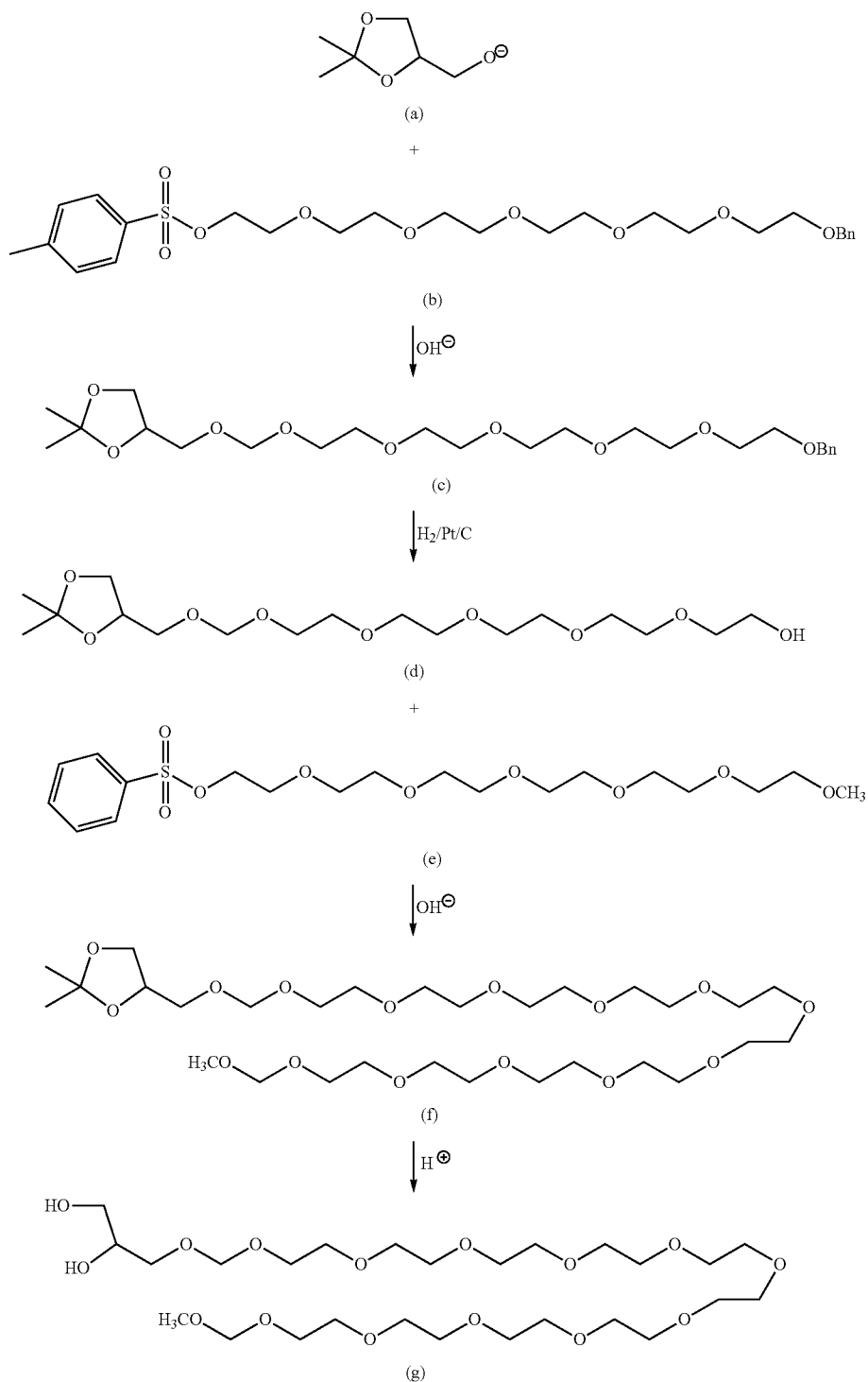
Reaction Scheme 1: Synthesis of 3-monomethoxyDodecaethylene glycol (mPEG-12)-glycerol
