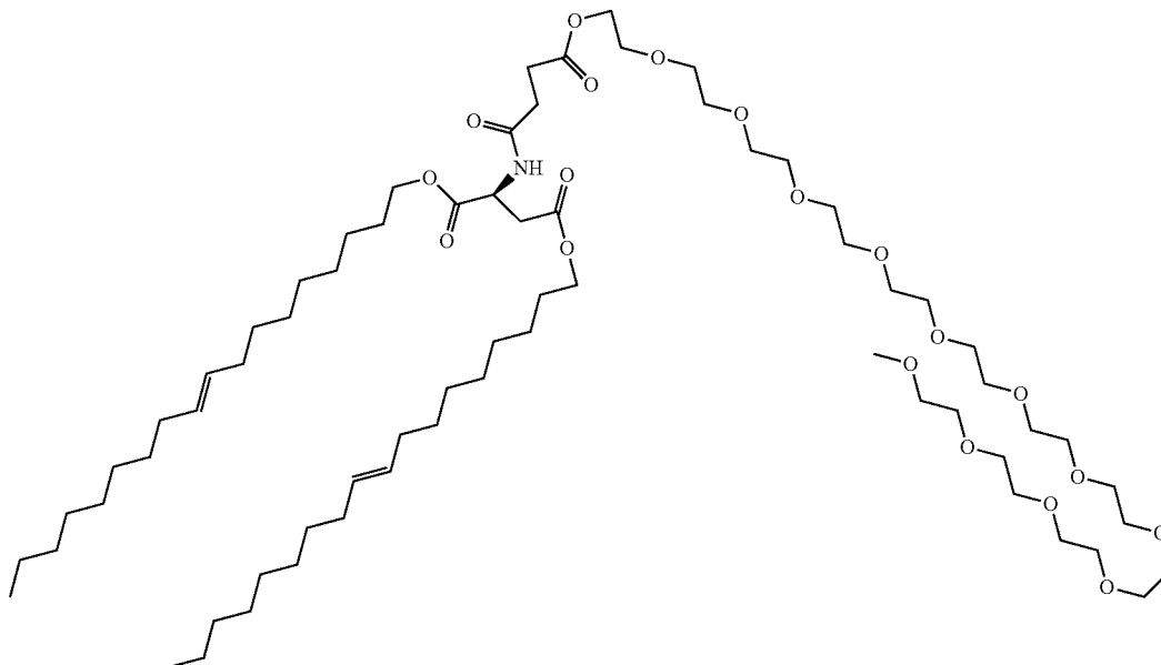
Chemical Structure 14: 1,4-dioleoyl-2-(m-PEG-12-succinylamino)-aspartate
