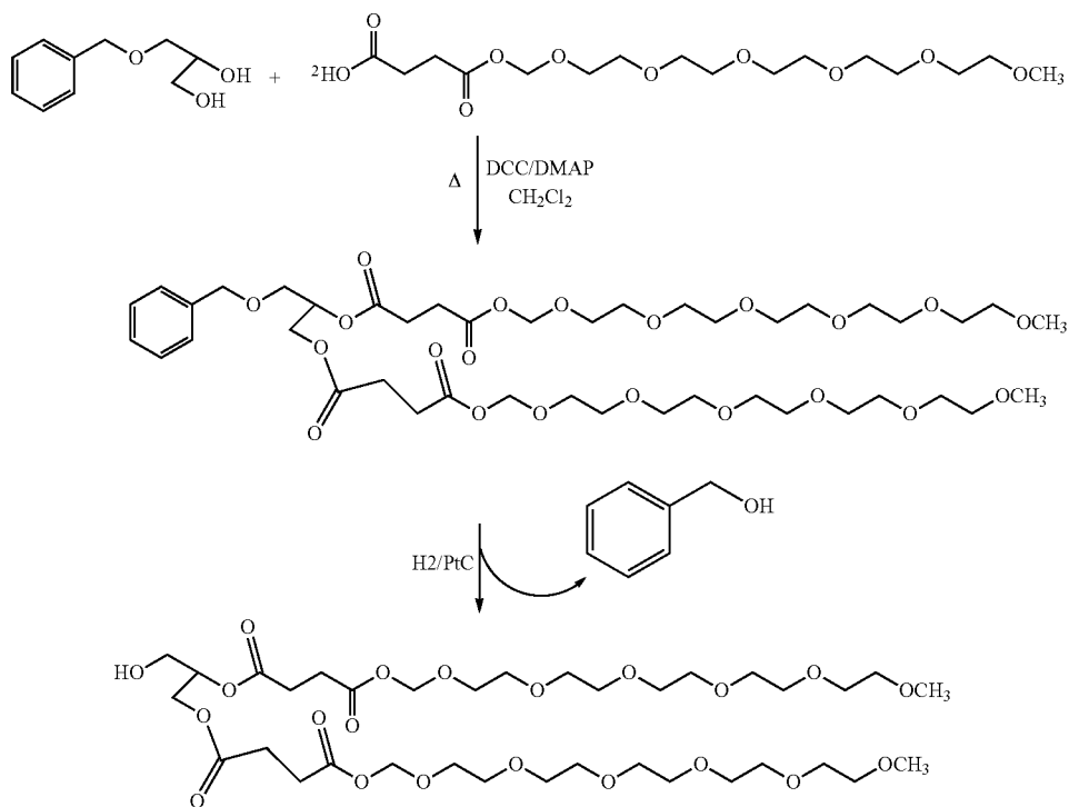
Reaction Scheme 7: Synthesis of 3-choleoyl-1,2-bis(methoxyhexaethylenesuccinyl glycol)-3-choleate
