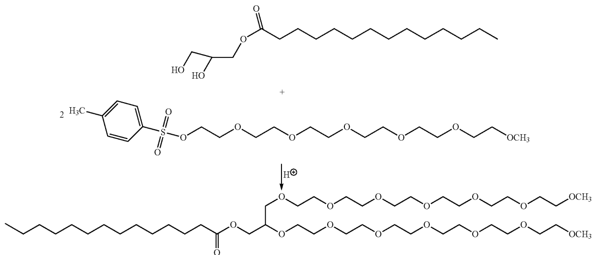
Reaction Scheme 6: Synthesis of 3-myristoyl-1,2-bis(methoxyhexaethylene glycol)glycerol
