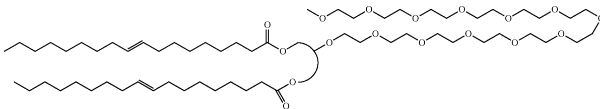
Chemical Structure 18: 1,3-dioleoyl-rac-2-monomethoxyDodecaethylene glycol (mPEG-12)-glycerol
