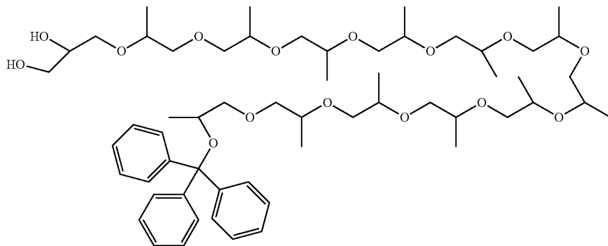
Chemical Structure 19: 3-trityl-dodecapropylene glycol-1,2-dihydroxyl-glycerol
