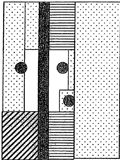
Figure 8A: NT Device Cross Section – SINGLE NANOTUBES
