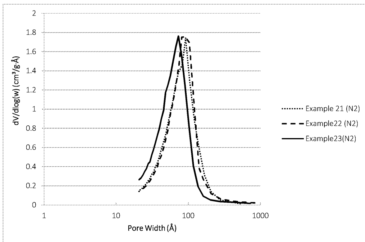
Figure 4: Mesopore Distribution of Silica-Zirconia Supports - Results of N 2 Adsorption for Examples 21 to 23.
