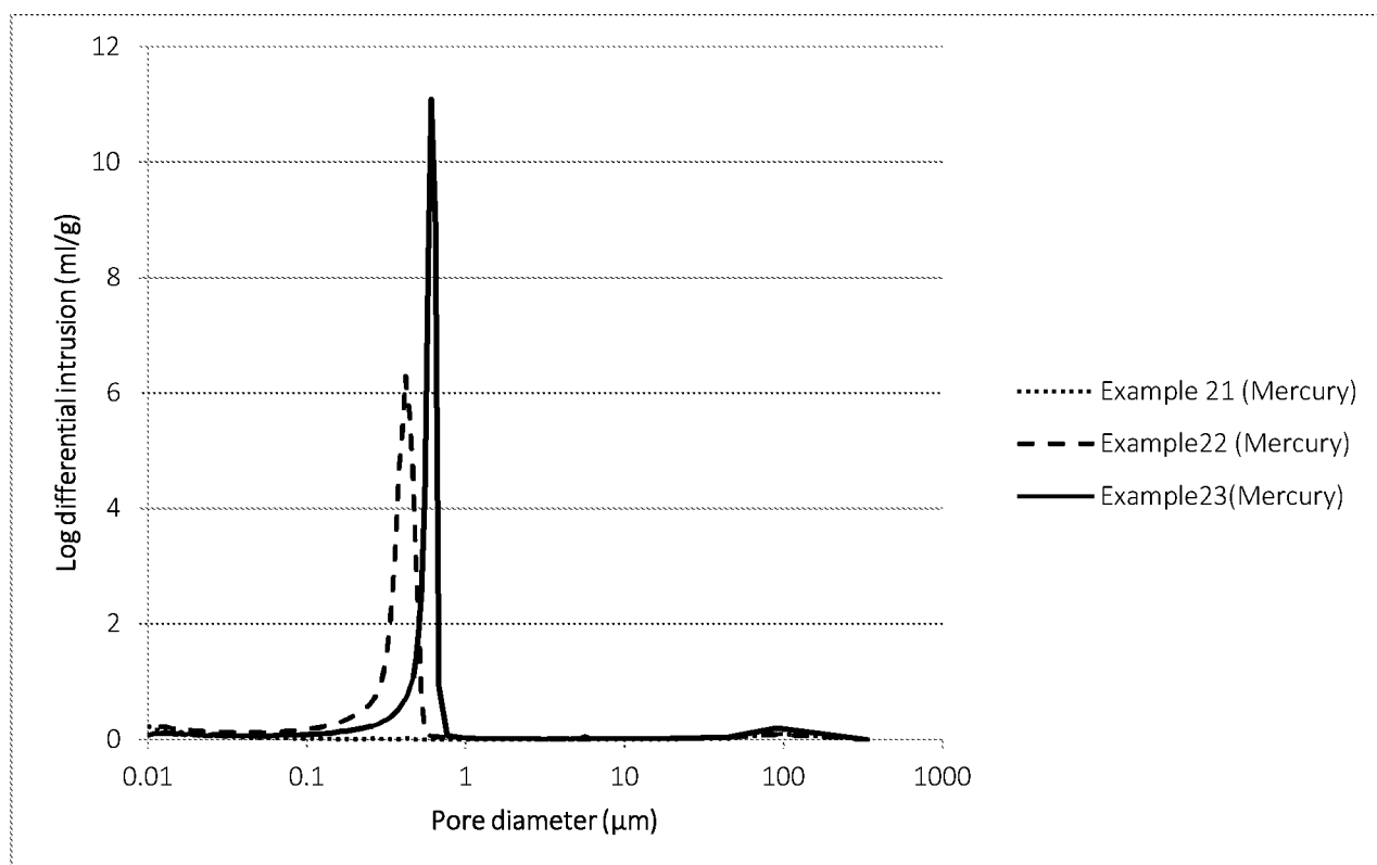
Figure 3: Macropore Distribution of Silica-Zirconia Supports - Results of Mercury Porosimetry for Examples 21 to 23.
