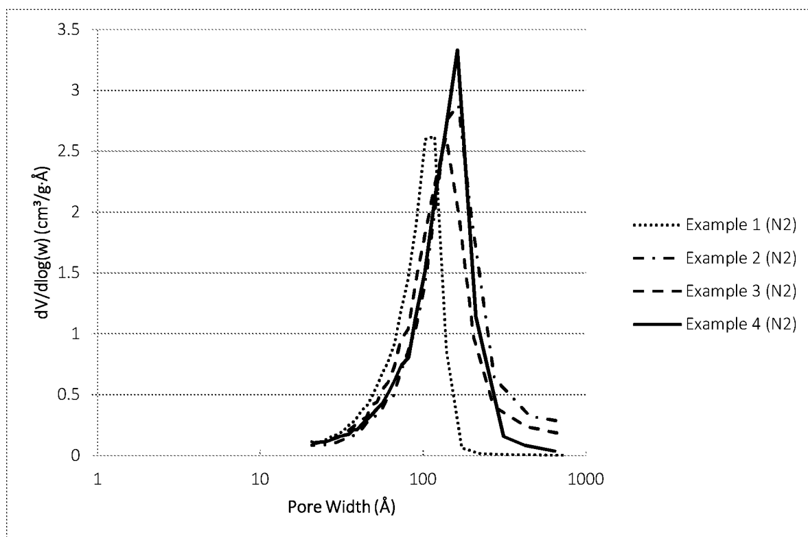
Figure 2: Mesopore Distribution of Silica Supports: Results of N 2 Adsorption for Examples 1 to 4.
