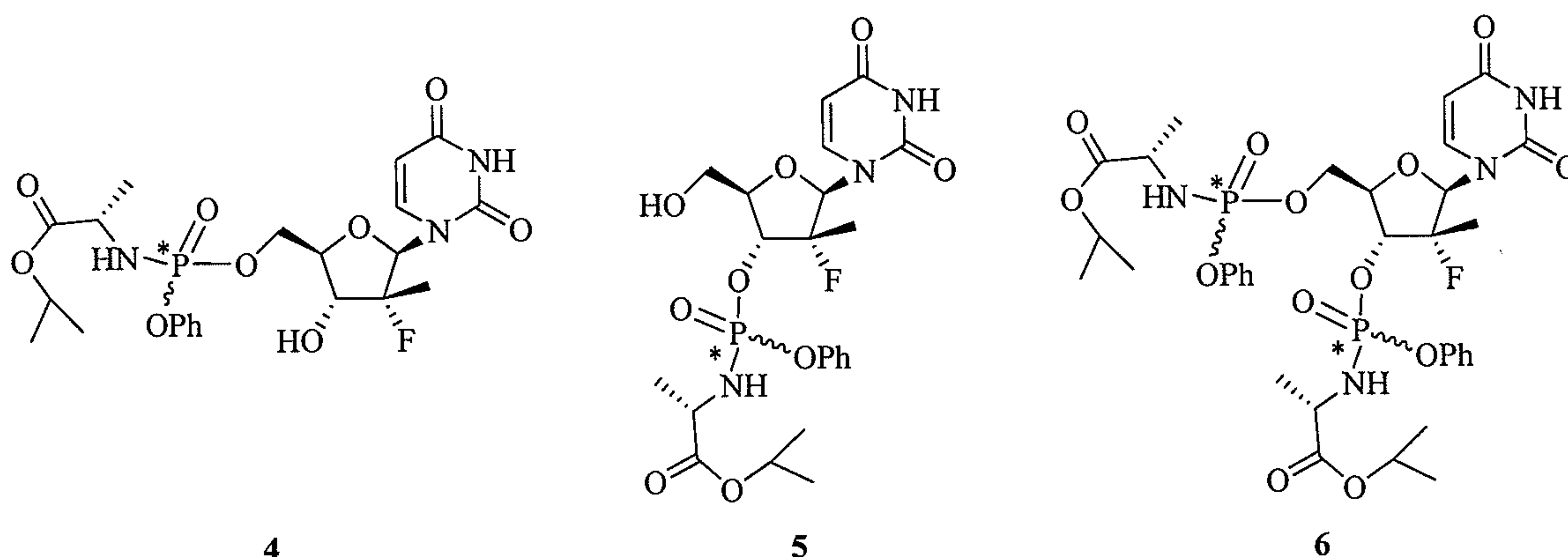
4 5'-O-phosphoramidate (2 diastereomers)
