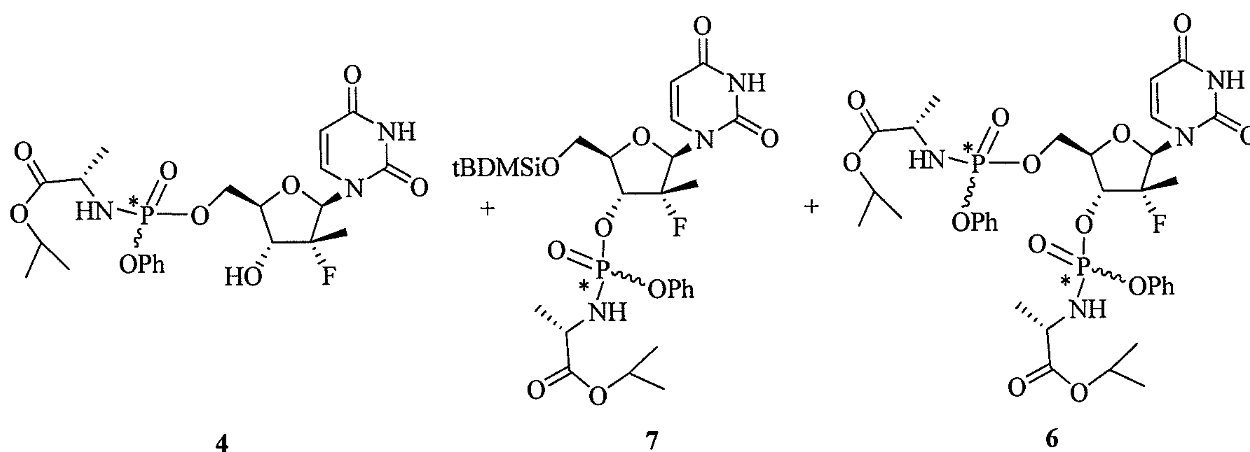
3'-O-phosphoramidate-5'-O-tBDMS (2 diastereomers)
