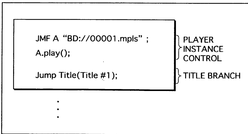
xlet PROGRAM
