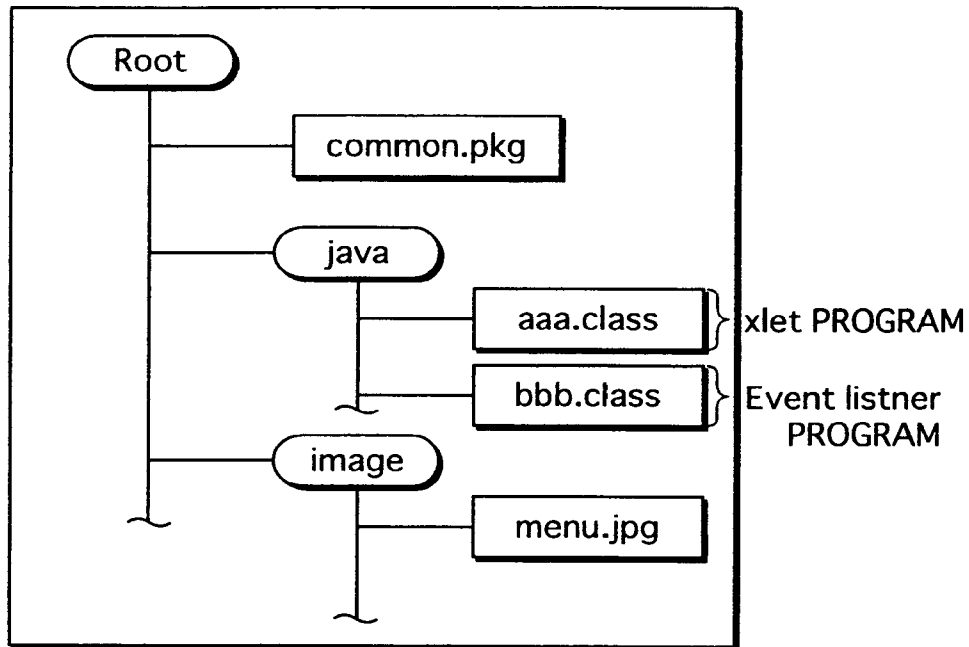
JAR FILE
